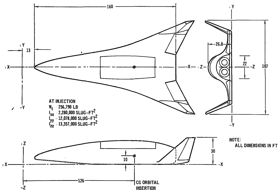
ORBITER B - HIGH CROSS RANGE
