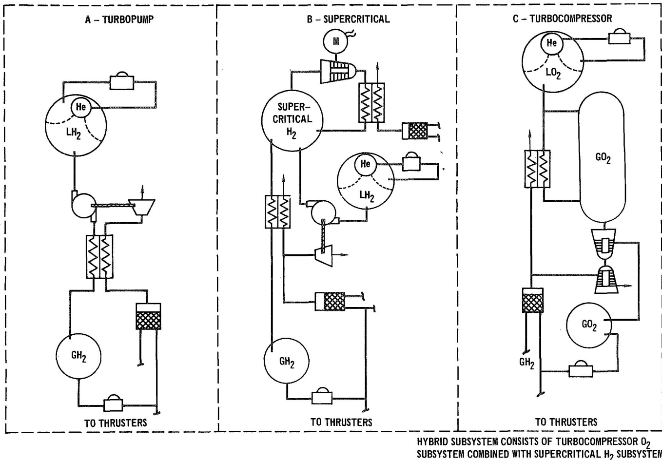
ORBITER APS CANDIDATE CONCEPTS
