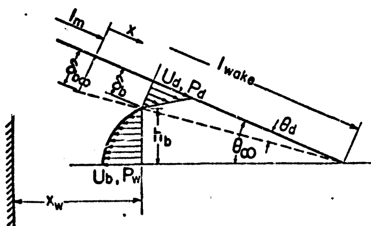
Figure 3b The Lower Viscous Layer
