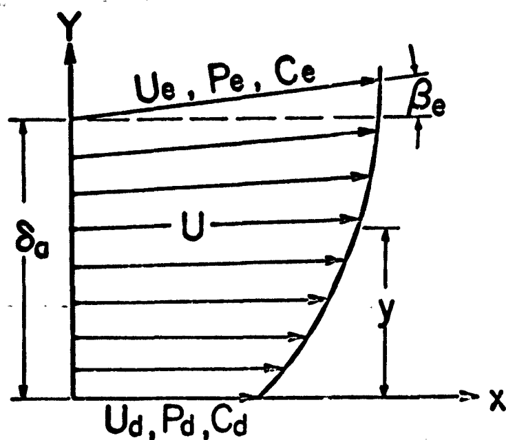
Figure 3a The Upper Viscous Layer
