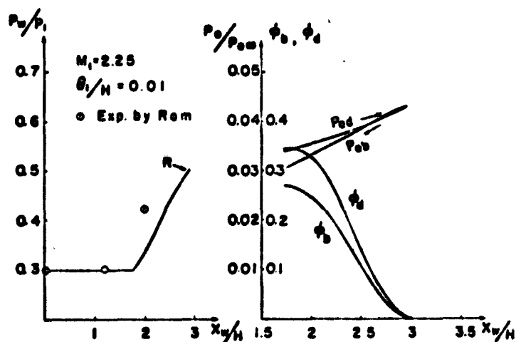
Figure 7 Results for M = 2.25 , \theta_1/H = 0.01
