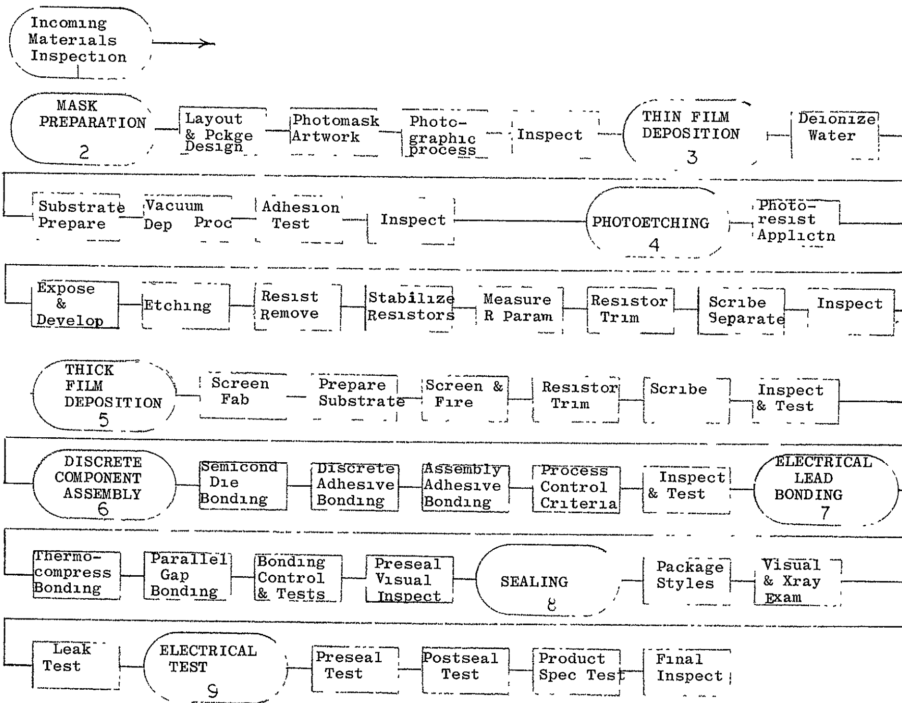
FIGURE 1-3. ECI HYBRID MICROCIRCUIT PROCESS- FLOW CHART
