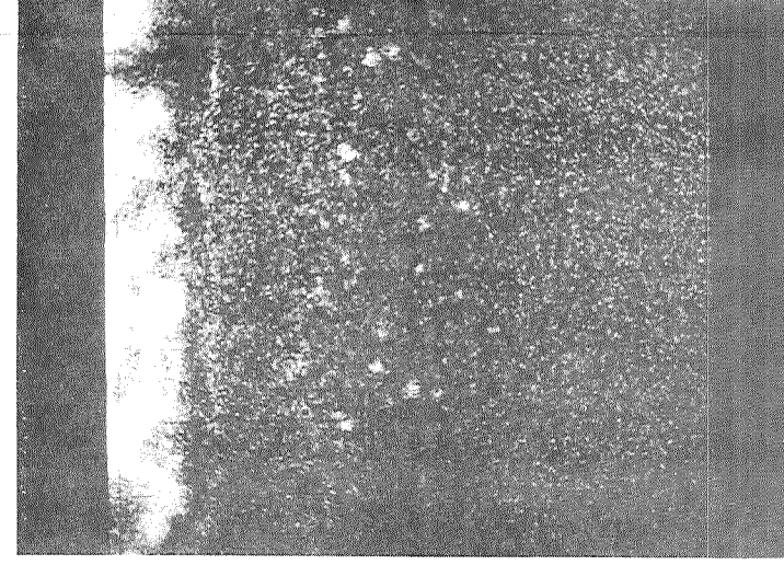
Figure 34. Microprobe Scans of Mn + Cr Metallide System on NASA/TRW VI-A Showing Metallized Elements and Ni Base After 20 Hours Dynamic Oxidation at 2000°F (1367°K) (E 4933, 360X).
