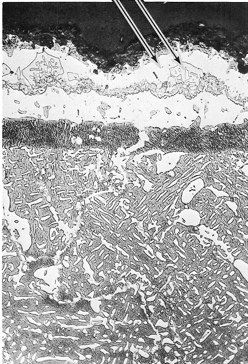
Figure 39. General Electric CODEP C-2 Pack-Type Aluminized Coating on IN-100 Alloy After 600 Hours Dynamic Oxidation at 2000°F (1367°K) (F 6022, 500X, TRW Etch).
