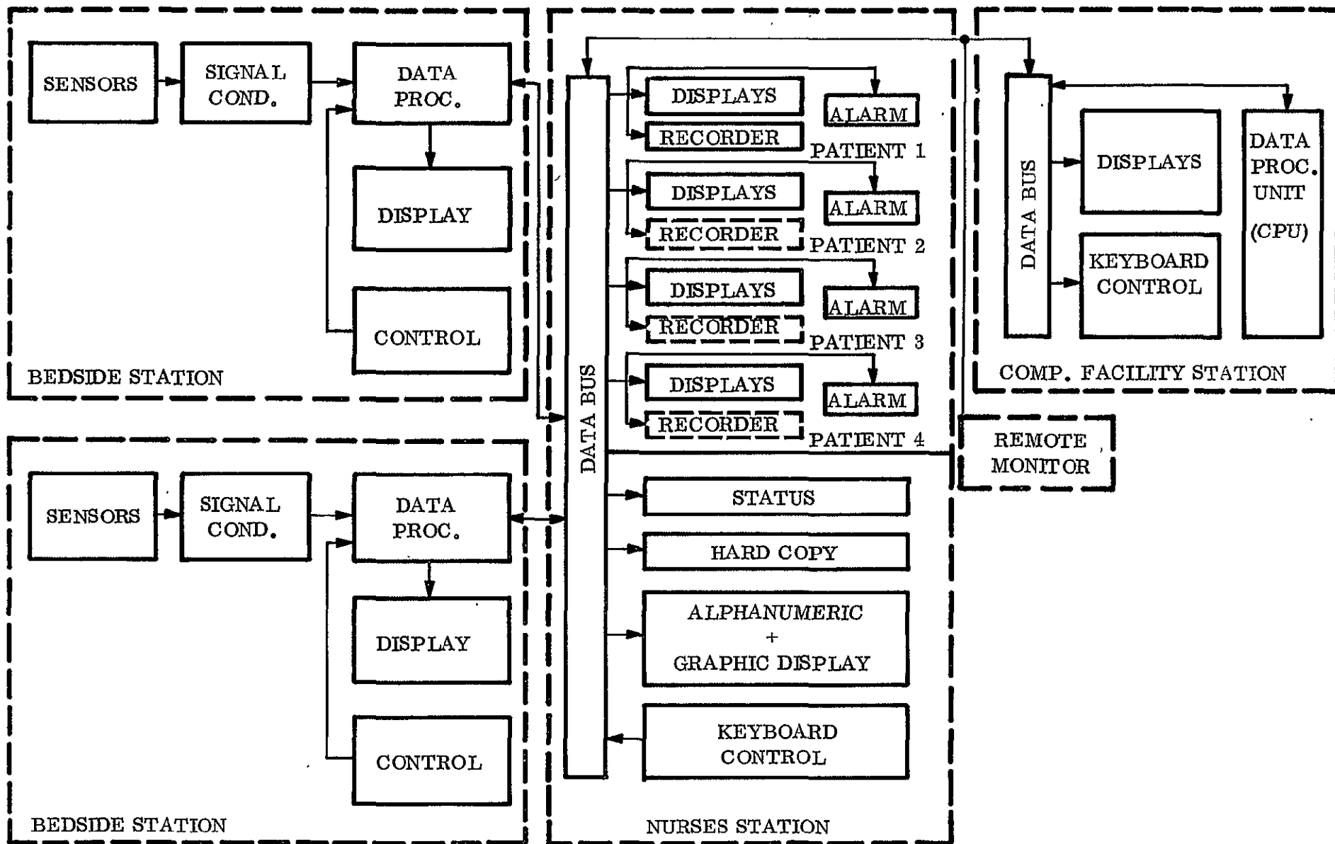
Figure V-1. Typical System Block Diagram
