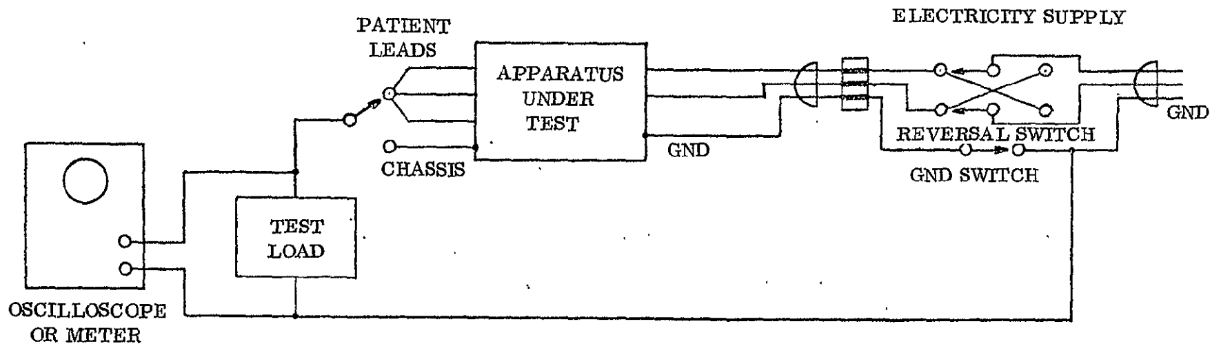
Figure 4.6.1. Test Circuit One (Paragraph 4.6.1 (a) )
