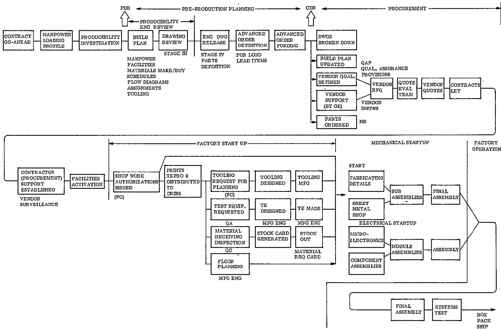
Figure 4.4-1. Manufacturing Flow
