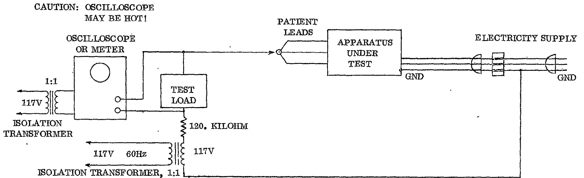
Figure 4.6.2. Test Circuit Two (Paragraph 4.6.1 (b) )
