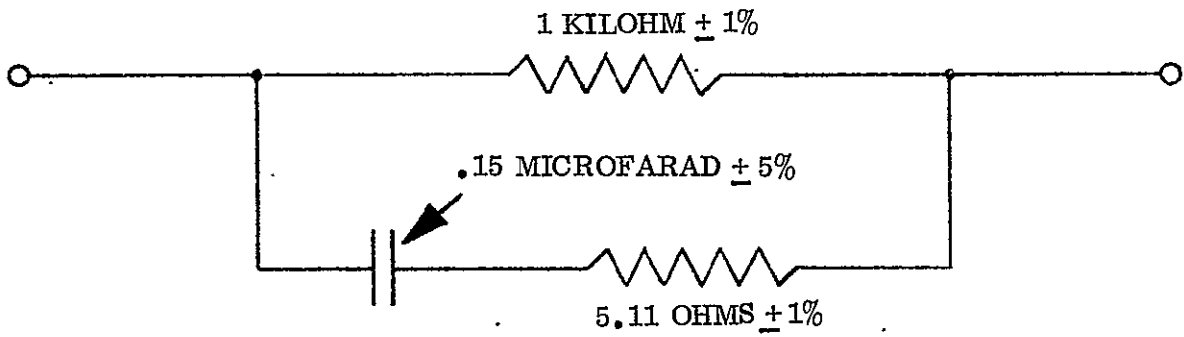
Figure 4.6.4. Test Load, Type A
