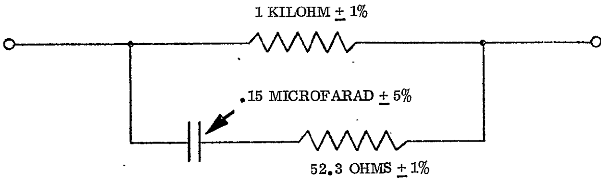
Figure 4.6.5. Test Load, Type B
