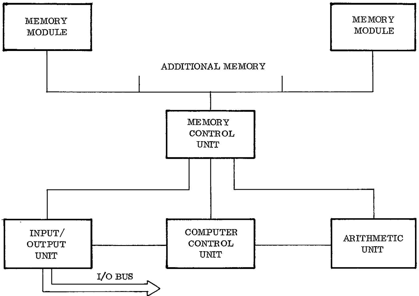
Figure V-9. Block Diagram of Basic Minicomputer
