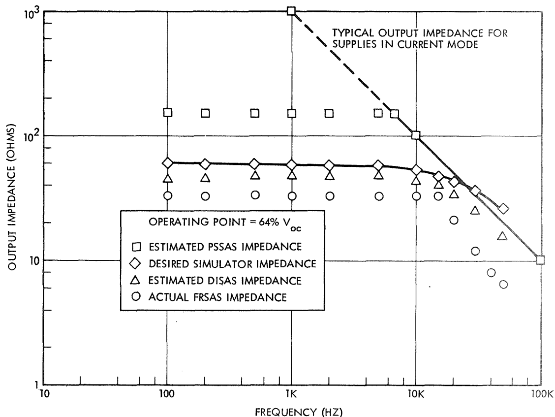
Figure 6.5-1. Comparison of the Impedance Simulation Capabilities of the FRSAS, PSSAS, and DISAS at One Operating Point for an Array of (N_s/N_p) = 1
