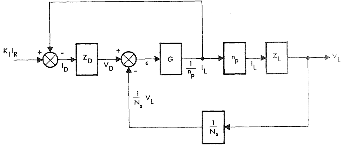
Figure 5.3-5. Analog System (After)
