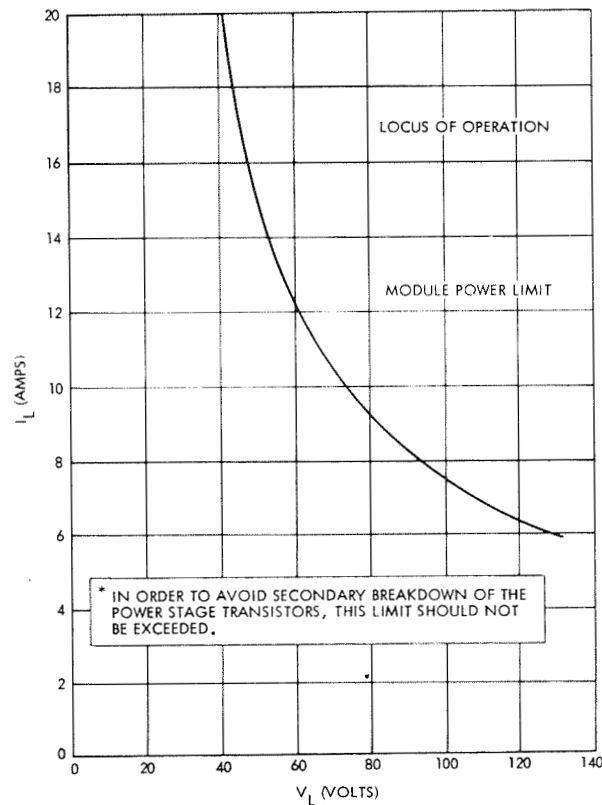
Figure 6.1.1. Output Power Limits of the FRSAS Basic Unit
