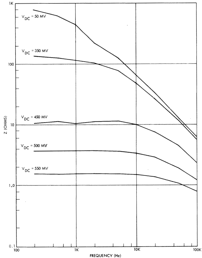
Figure 5.4-7. Forward Biased Solar Cell Ampedance Versus Frequency
