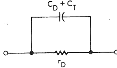
Figure 5.4-2. Simplified Equivalent Circuit For Cell
