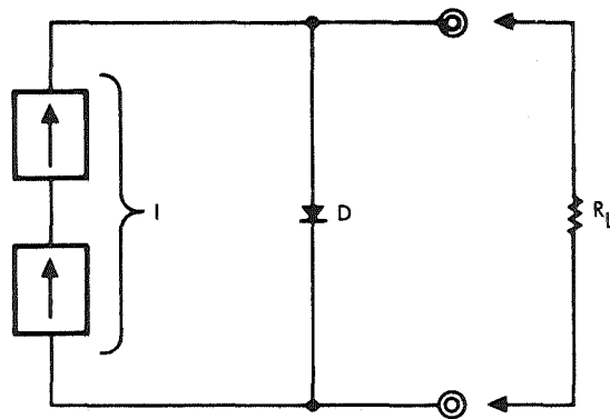
Figure 6.3-3. Simplified DISAS Using Supplies in Current Limit Mode
