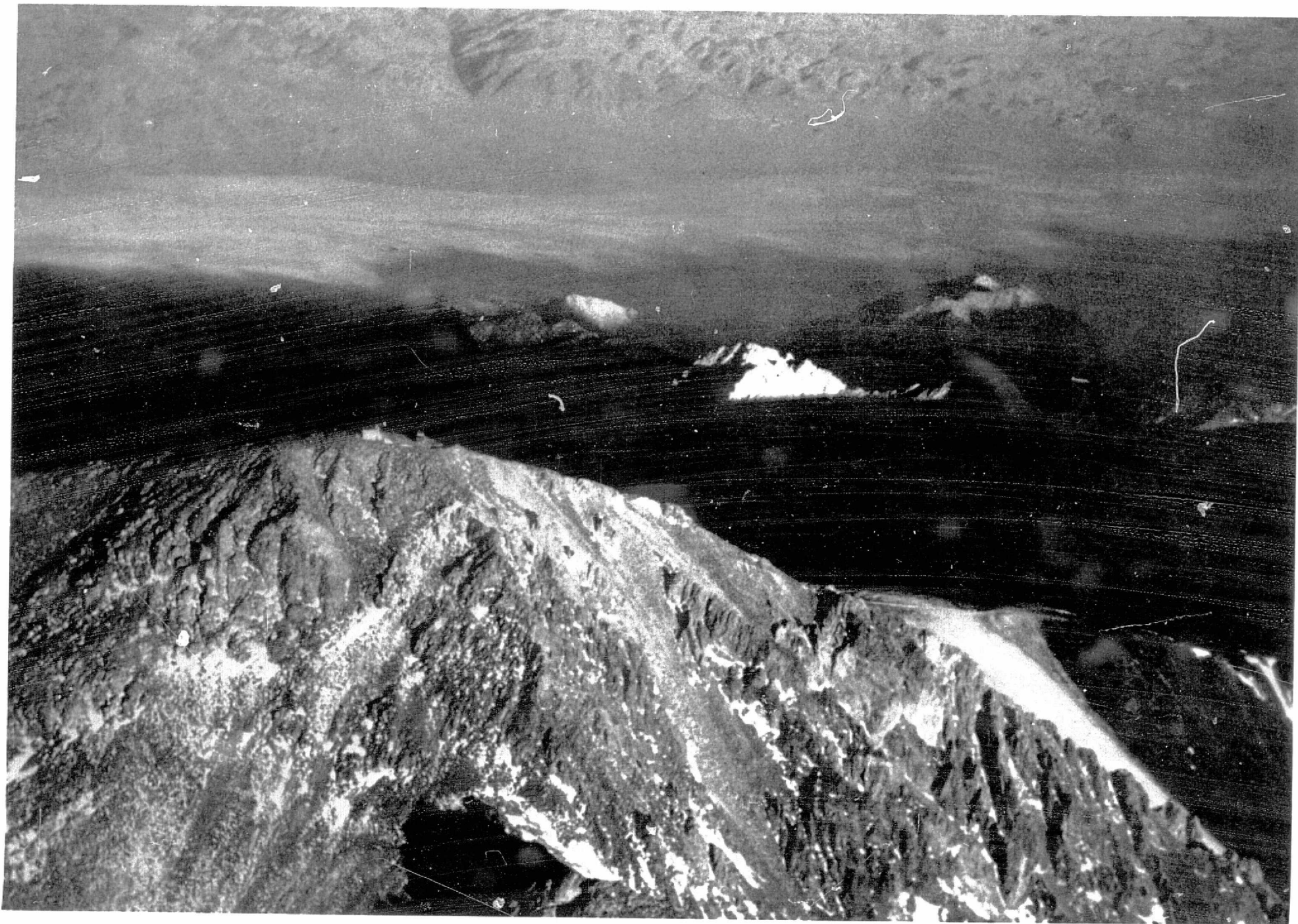
Fig. 16 Summit from W, like Fig. 12 but closer (light-colored wedge, 2 inches from right margin, also shown on Fig. 15, is sulphur, not snow).
