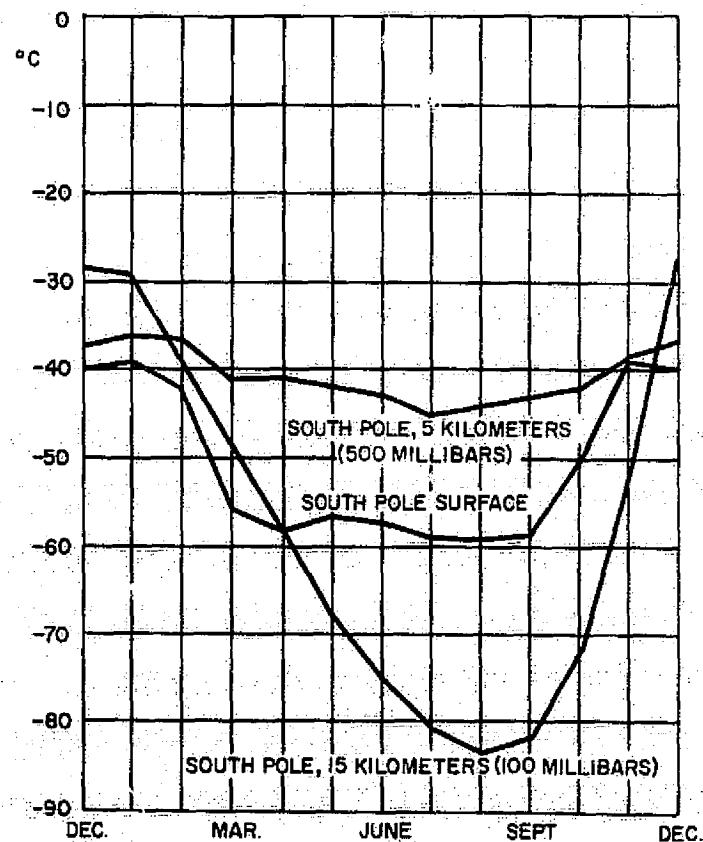
Fig. 1 Mean monthly temperatures at Amundsen-Scott Station, South Pole (Rubin, 1962).
