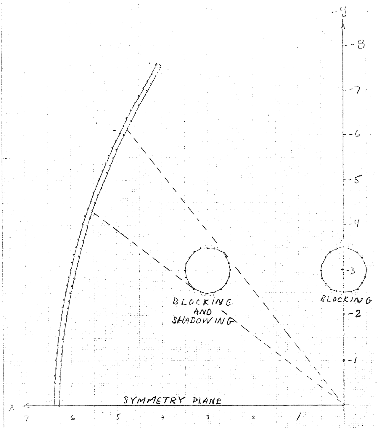
Fig. IV-19. Geometry of Blocked and Shadowed Cylindrical Parabola Reflector
