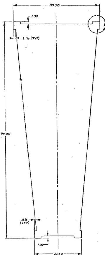
Fig. IV-10. Geometry of Cross Section of AAS Tetrapod Leg
