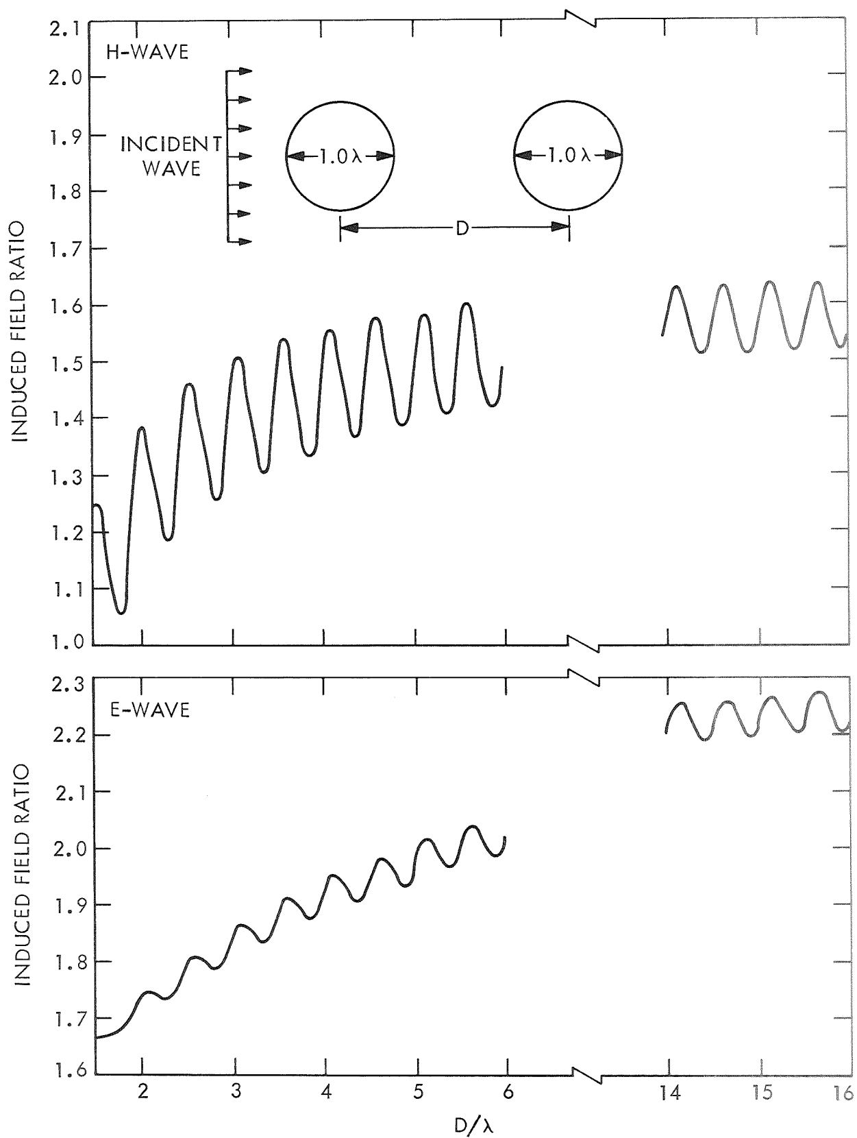
Fig. IV-6. Induced Field Ratio of Two Right-Circular Cylinders versus Longitudinal Separation
