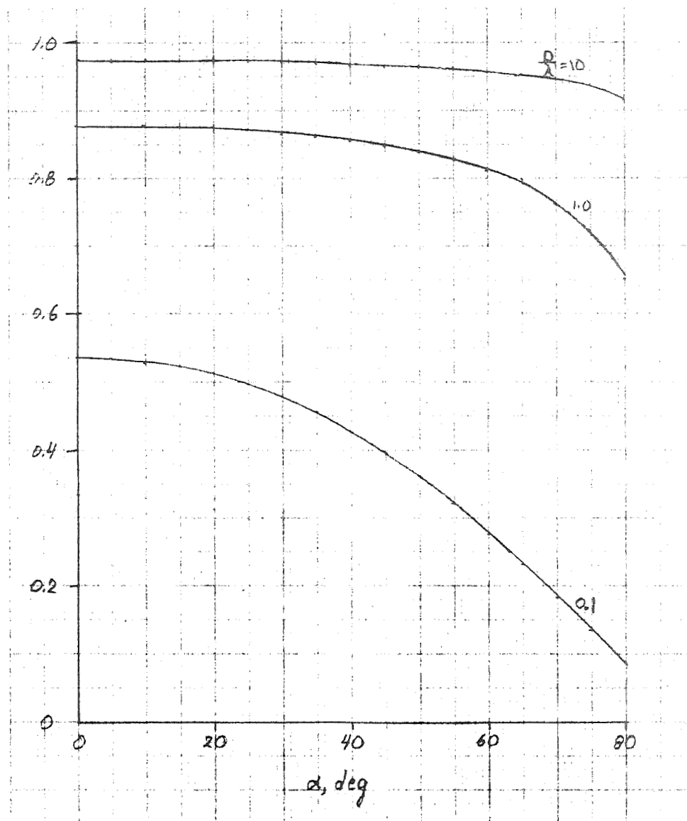
Fig. IV-4. Classical Results for H-Wave Induced Field Ratio versus Angle of Incidence
