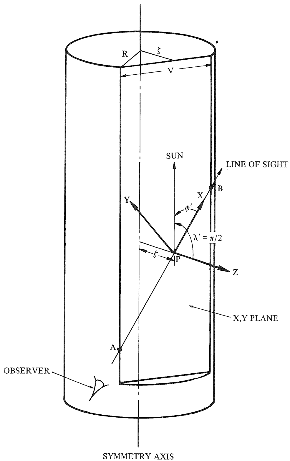
FIGURE 8 - SHADOW GEOMETRY FOR \lambda' = \pi/2 .
