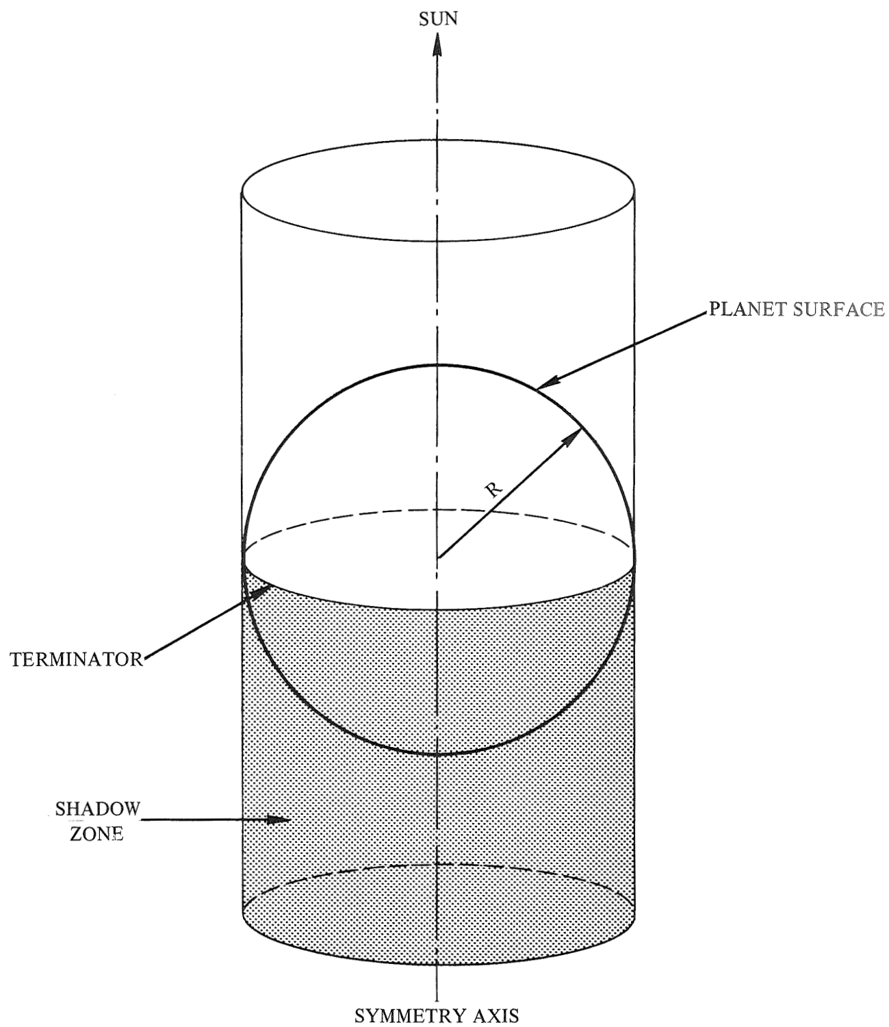
FIGURE 5 - THE SHADOW ZONE
