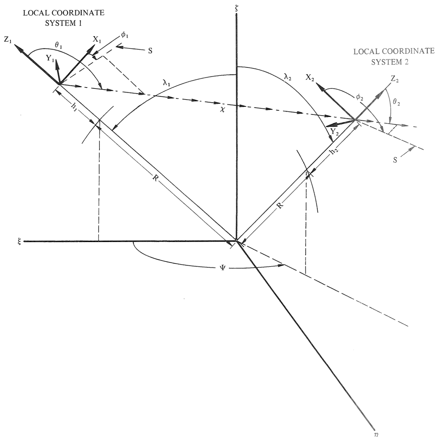
FIGURE 4 - LOCATION OF ONE LOCAL COORDINATE SYSTEM WITH RESPECT TO ANOTHER. THE ORIGIN OF THE \xi\eta\zeta COORDINATE SYSTEM IS AT THE CENTER OF THE PLANET; THE \xi AXIS POINTS TOWARD THE SUN. BOTH \phi_1 AND \phi_2 ARE SHOWN AS NEGATIVE ANGLES. THE LINES MARKED S ARE IN THE RESPECTIVE X-Y PLANES.
