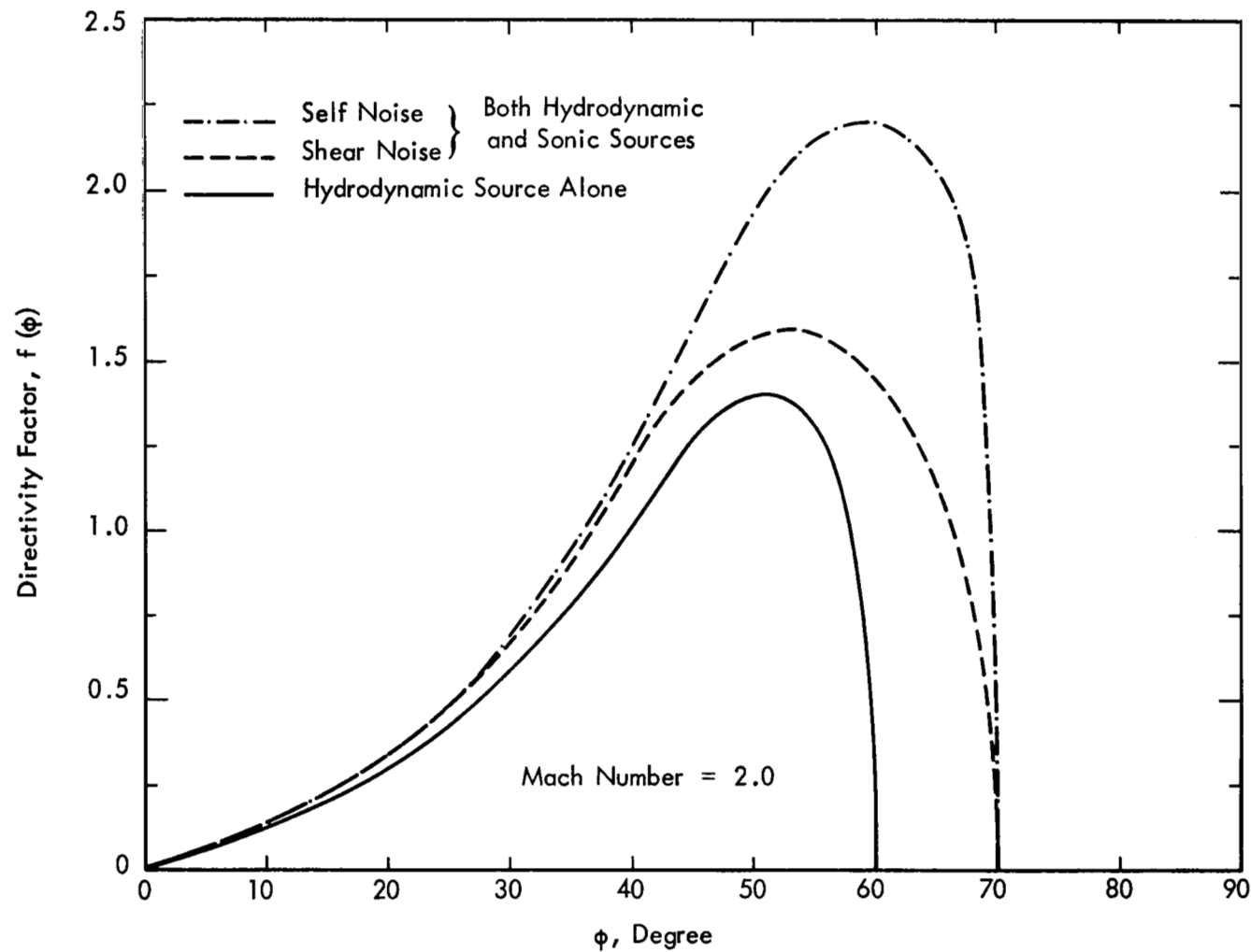
Figure 6. Noise Radiation Directivity Pattern for the Mach Modes [S.1] and [S.2]. The turbulent source strength is assumed to be constant across the shear layer
