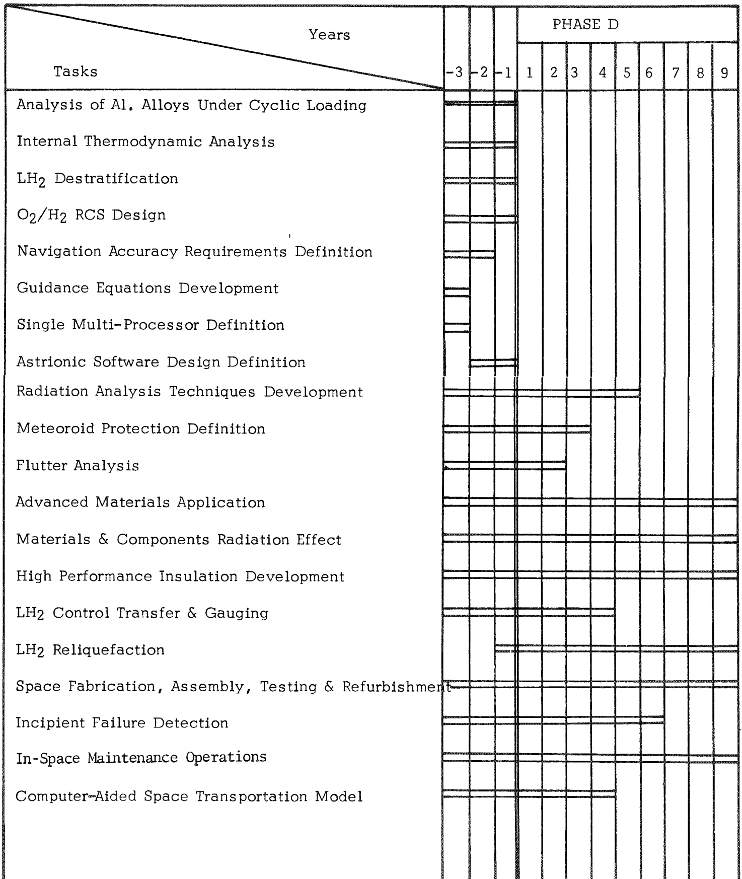
Figure 5-2. Supporting Research and Technology Program Schedule
