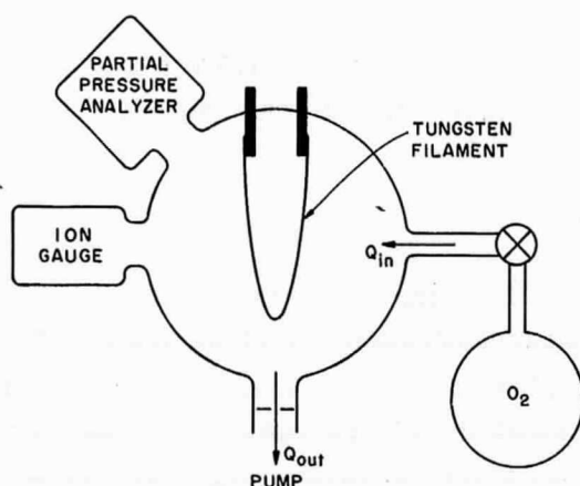
Fig. III-1. Singleton's experimental apparatus.
