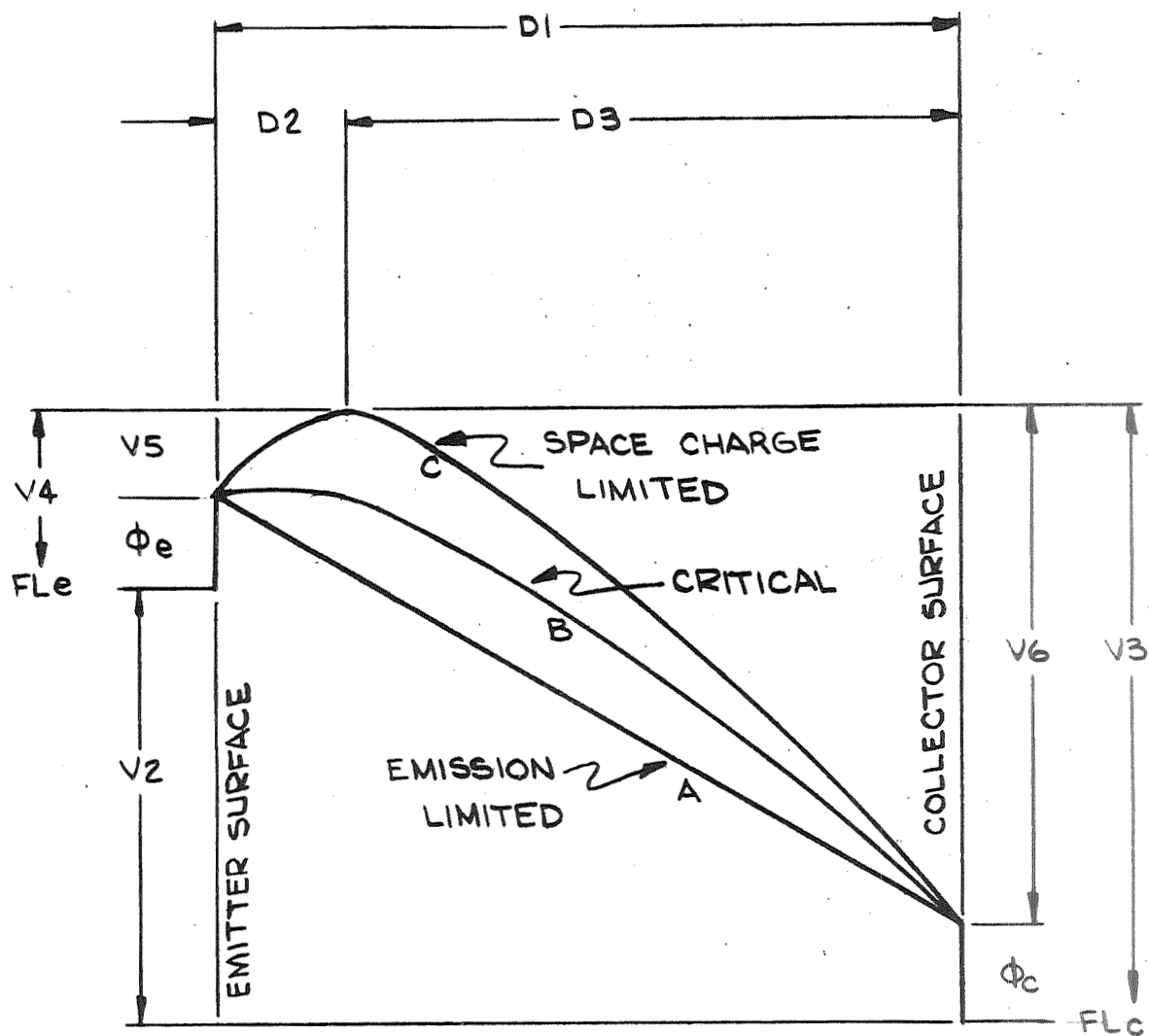
ELECTRON POTENTIAL ENERGY DIAGRAM
