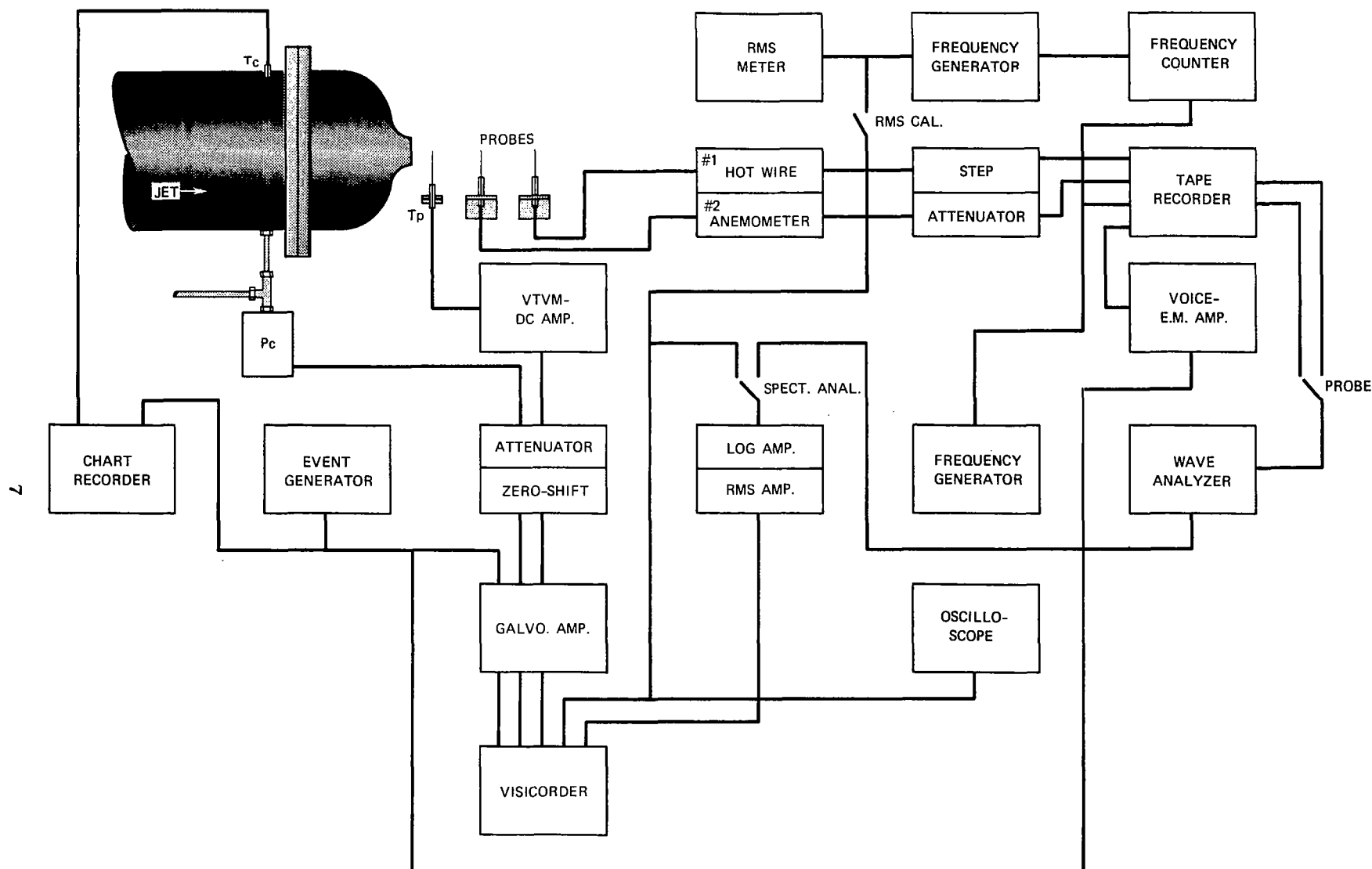
FIGURE 2 SCHEMATIC DIAGRAM OF INSTRUMENTATION
