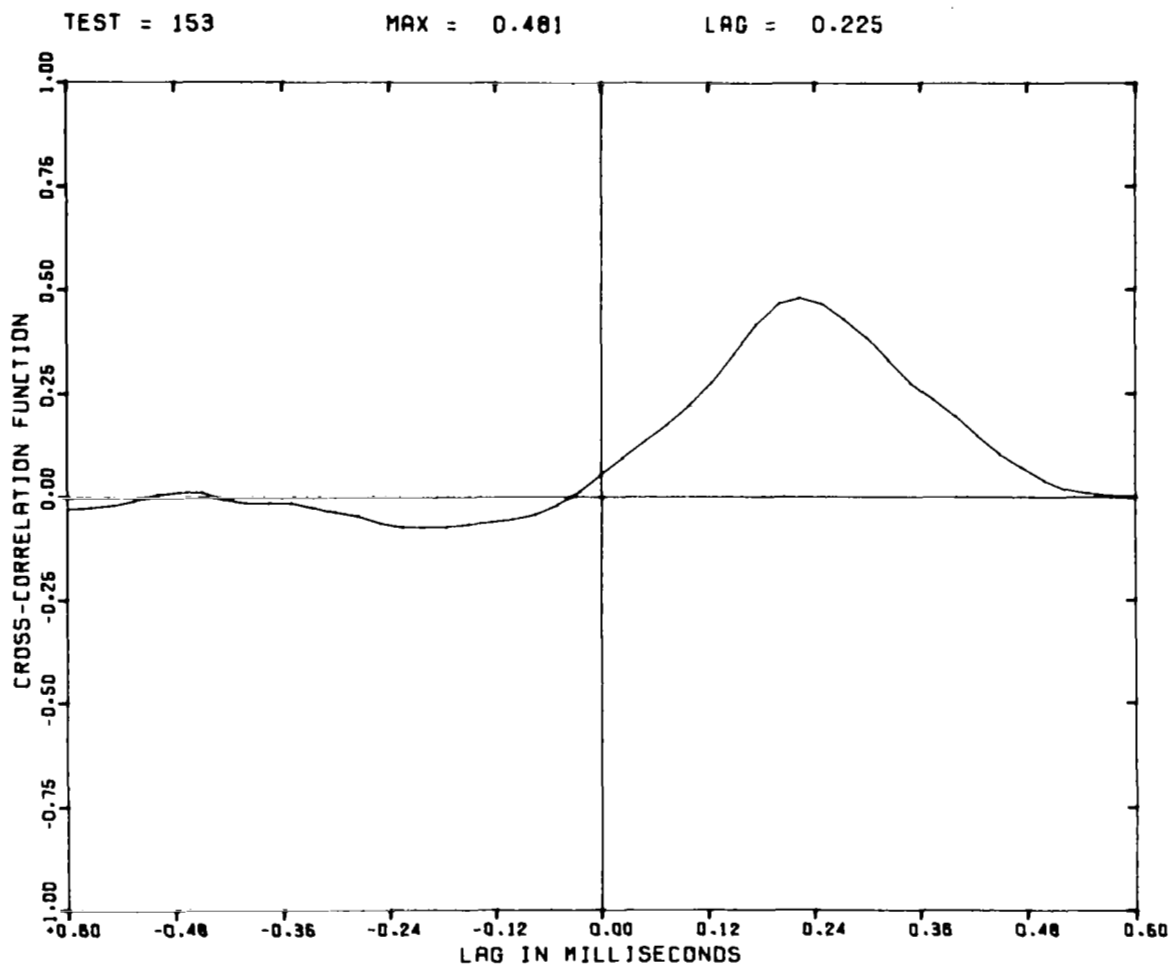
FIGURE 32 CROSS-CORRELATION FUNCTION R_{11} VERSUS TIME LAG
