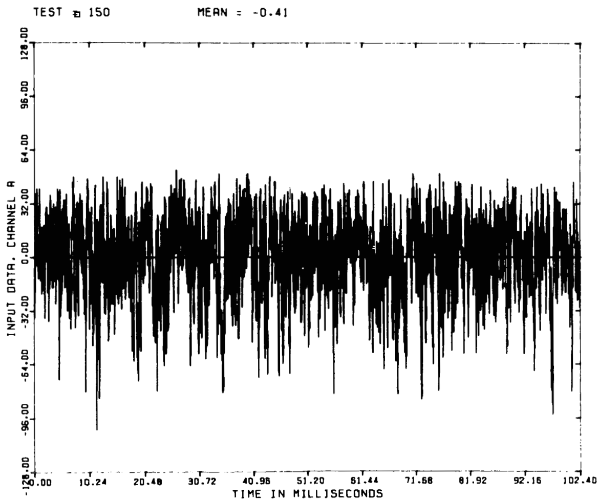
FIGURE 29 INPUT DATA: SIGNAL FROM UPSTREAM HOT WIRE
