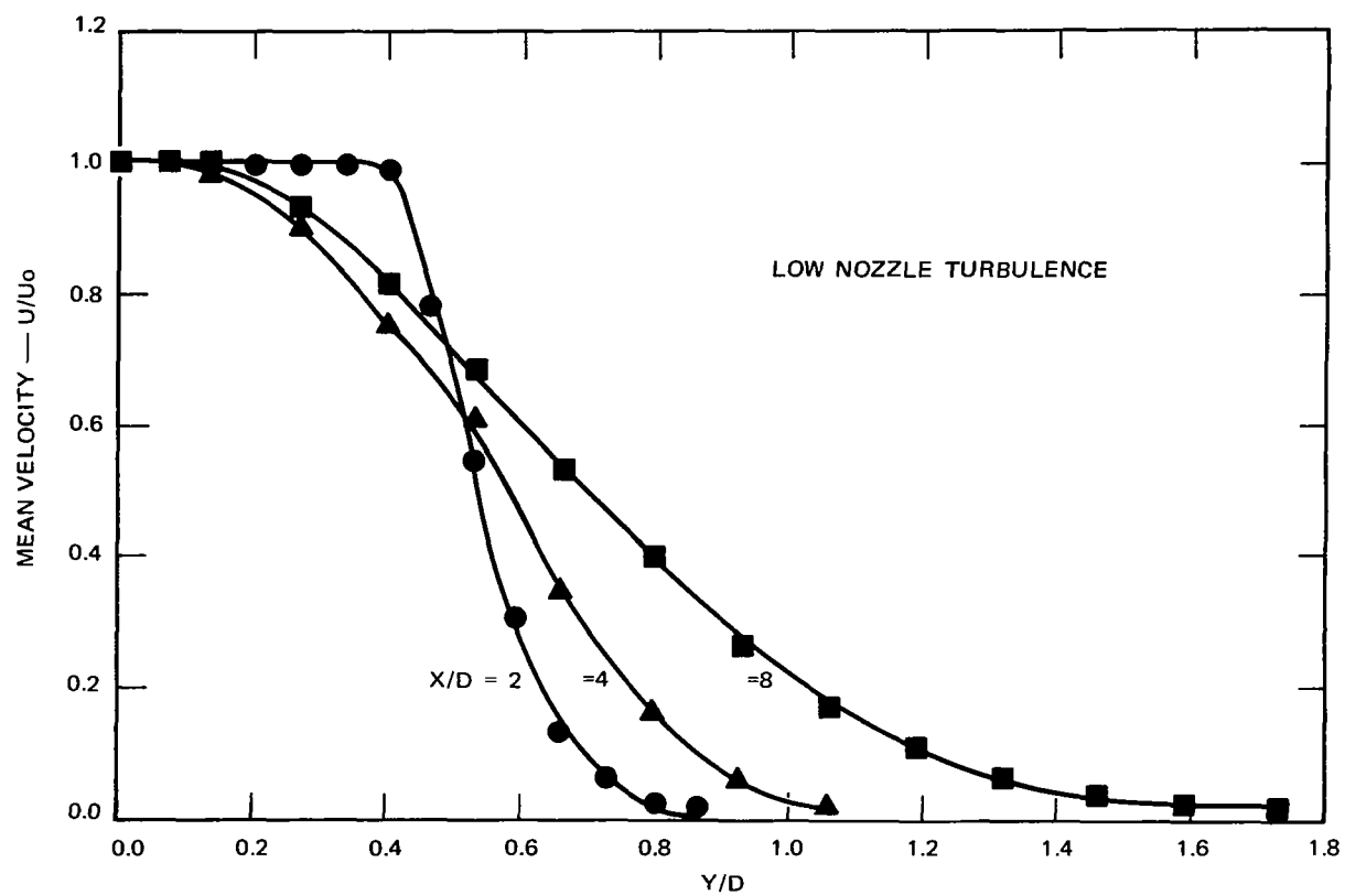
FIGURE 21 JET VELOCITY PROFILES FOR M \approx 0.68 AT VARIOUS X/D
