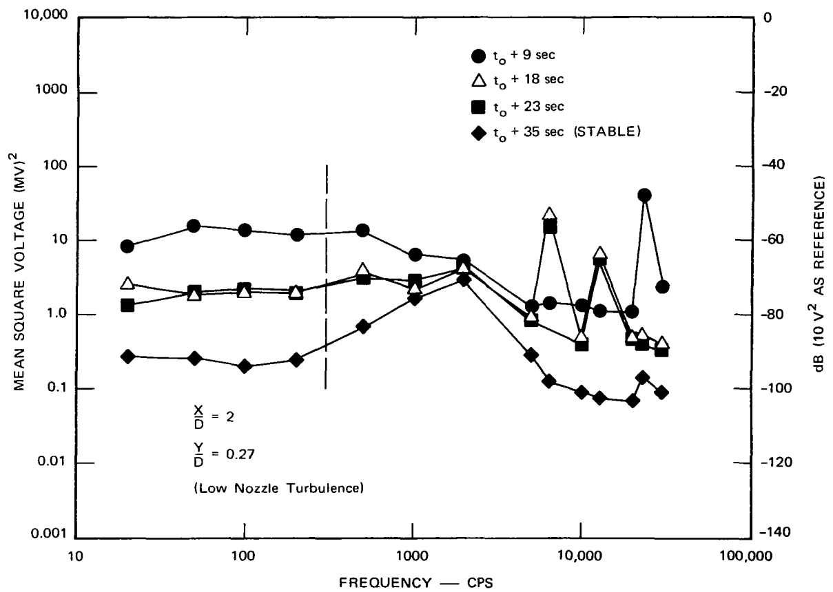
FIGURE 13 JET SPECTRUM AT M = 0.32
