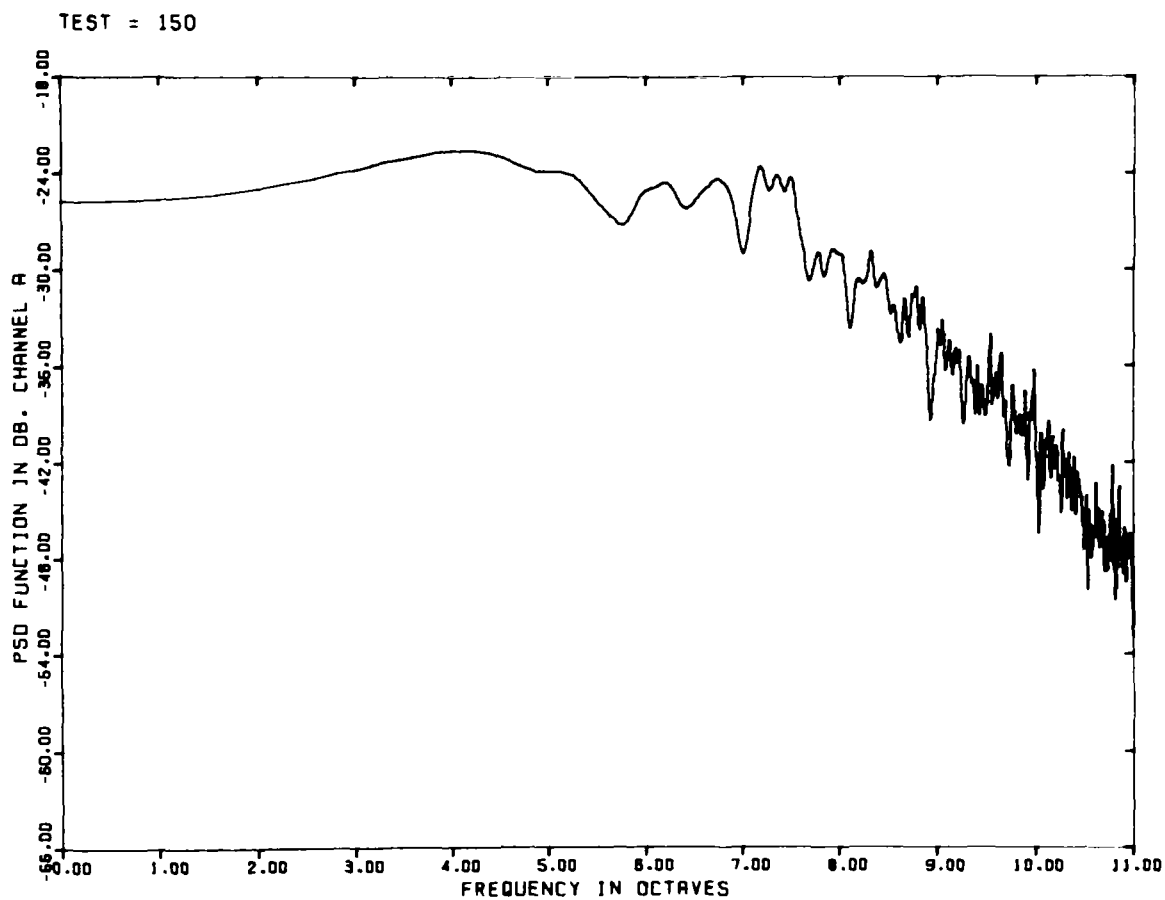
FIGURE 31 POWER SPECTRAL DENSITY OF SIGNAL FROM UPSTREAM WIRE
