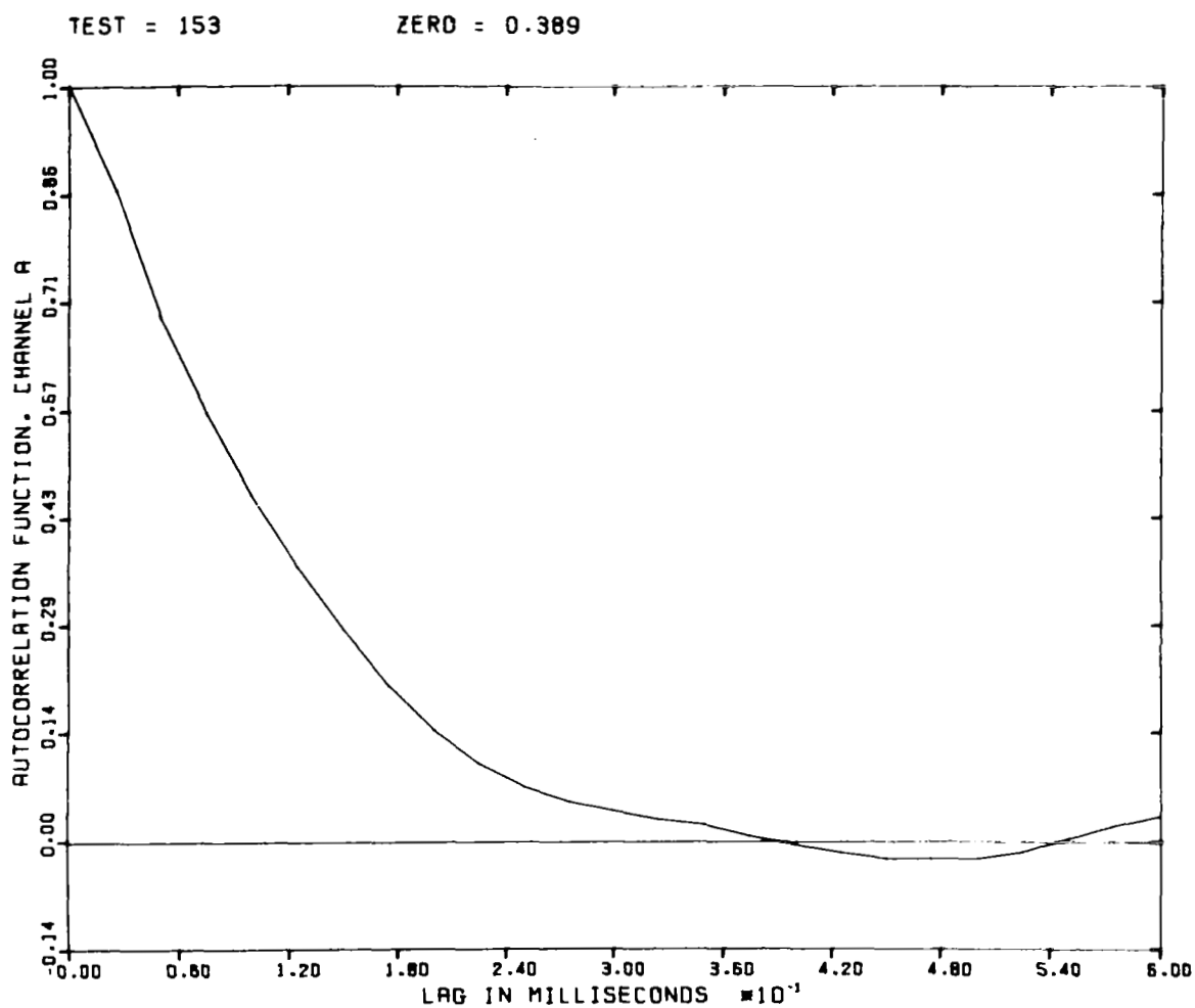
FIGURE 30 AUTOCORRELATION FUNCTION OF SIGNAL FROM UPSTREAM WIRE
