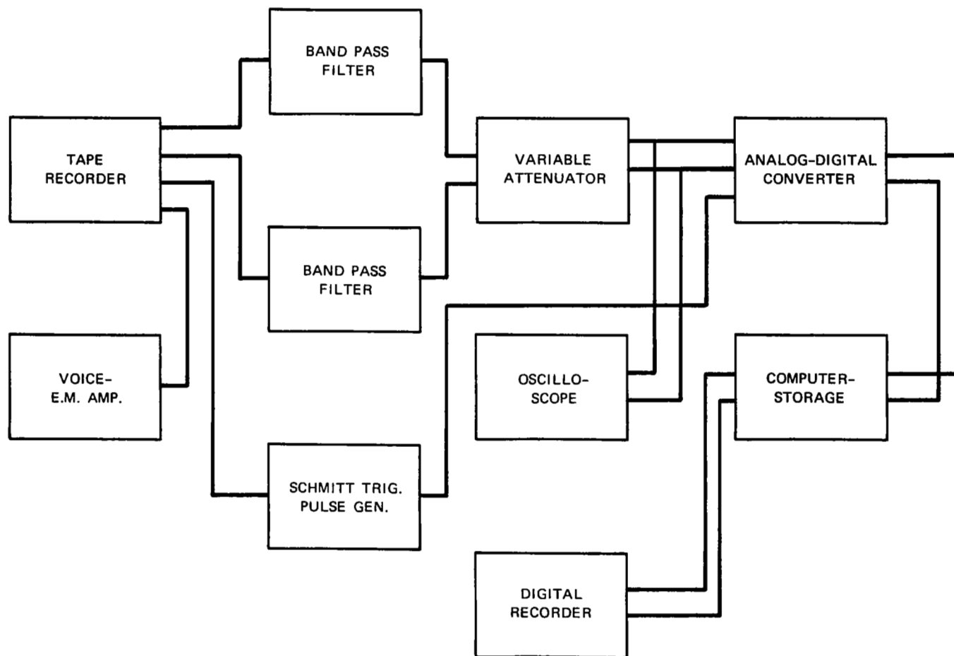
FIGURE 9 ANALOG-DIGITAL INSTRUMENTATION
