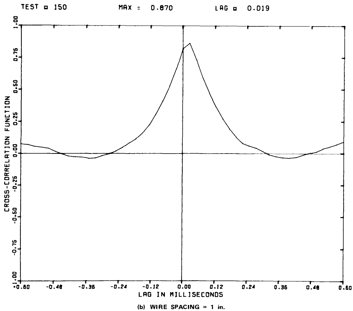
FIGURE 32 CROSS-CORRELATION FUNCTION R_{11} VERSUS TIME LAG (Concluded)
