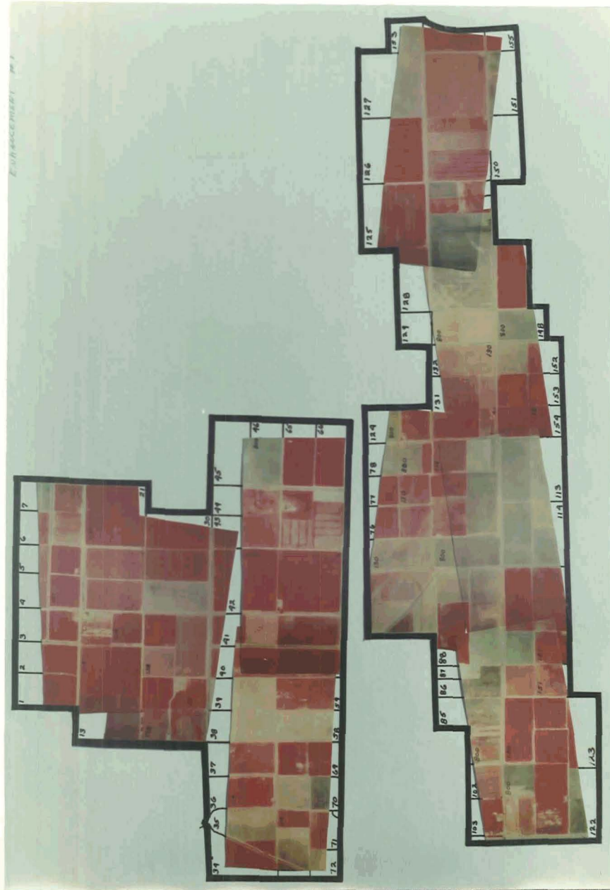
Figure 19. Enhancement A imagery and test results for the Imperial Valley, California, study area.
