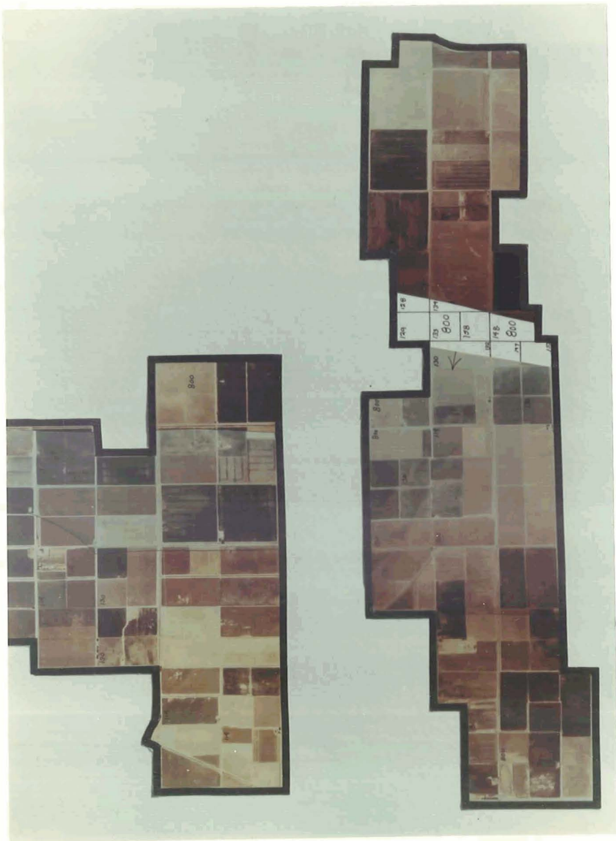
Figure 17. Aerial Ektachrome imagery and test results for the Imperial Valley, California, study area.
