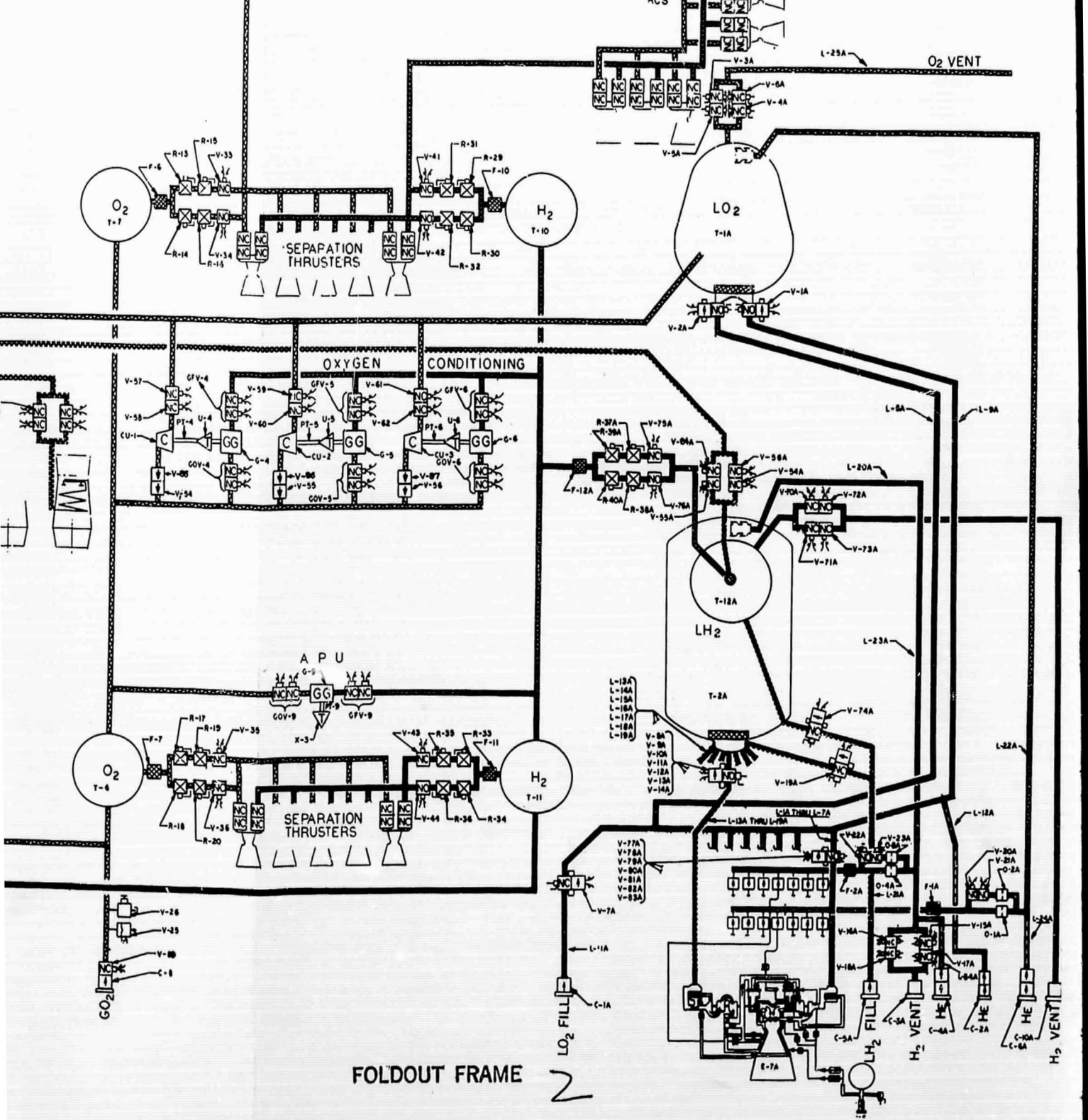
FIGURE II-4 BOOSTER PROPULSION
