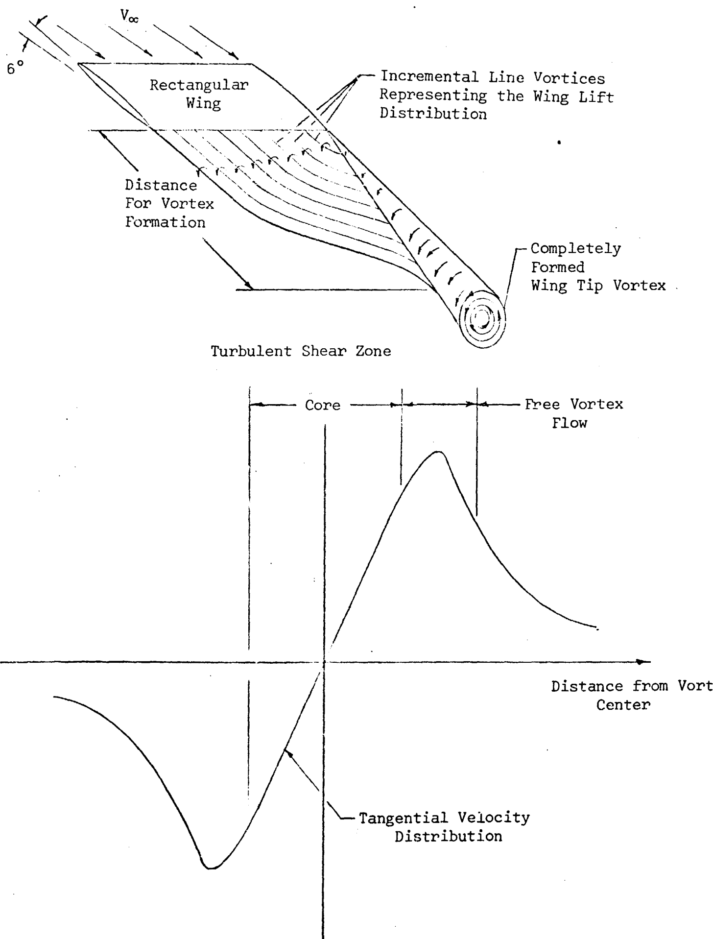
Figure 18 Schematic Representation of Wing Tip Vortex Formation and the Vortex Model Based on Tangential Velocity Distribution.
