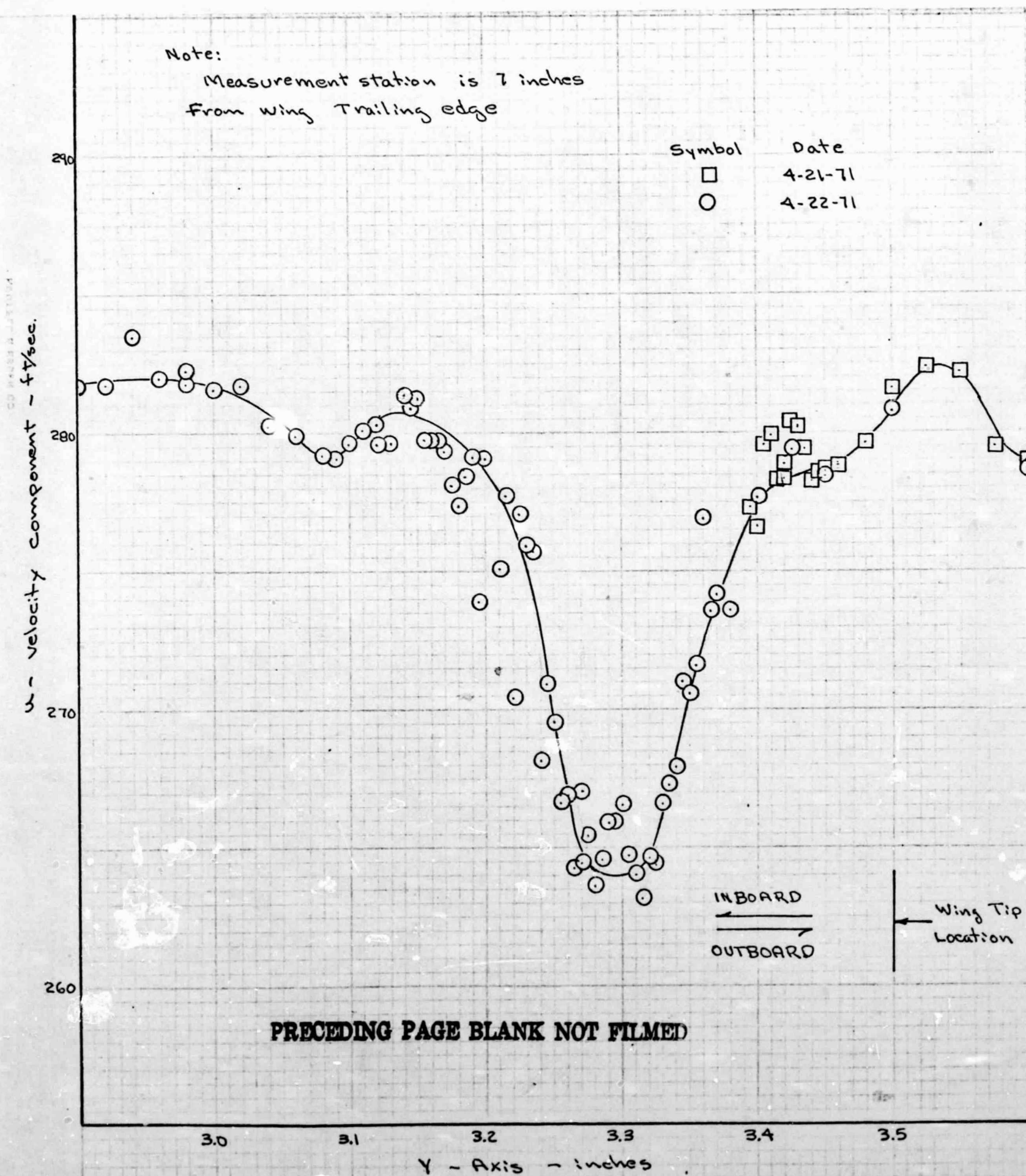
Figure 20 Variation in the u Velocity Component in a Wing Tip Trailing Vortex in MSFC 7 Inch Wind Tunnel
