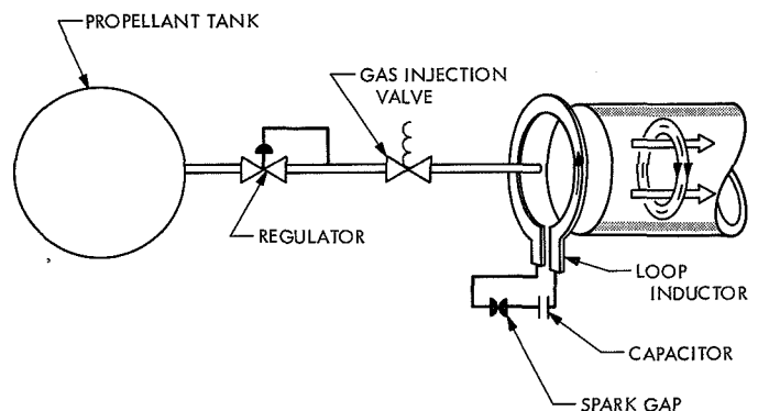
Fig. 34. Conceptual diagram of the pulsed inductive thruster
