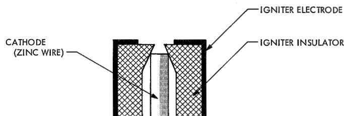
Fig. 44. Detail of cathode portion of the PVAT
