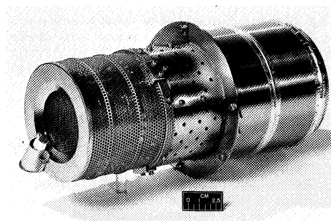
Fig. 17. Five-cm mercury bombardment thruster (photo courtesy of LeRC)
