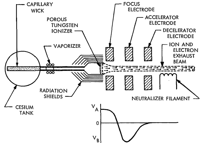
Fig. 1. Conceptual diagram of the contact-ion thruster
