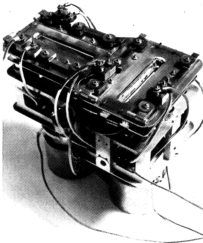
Fig. 13. HRL dual beam linear strip contact-ion thruster (photo courtesy of HRL)
