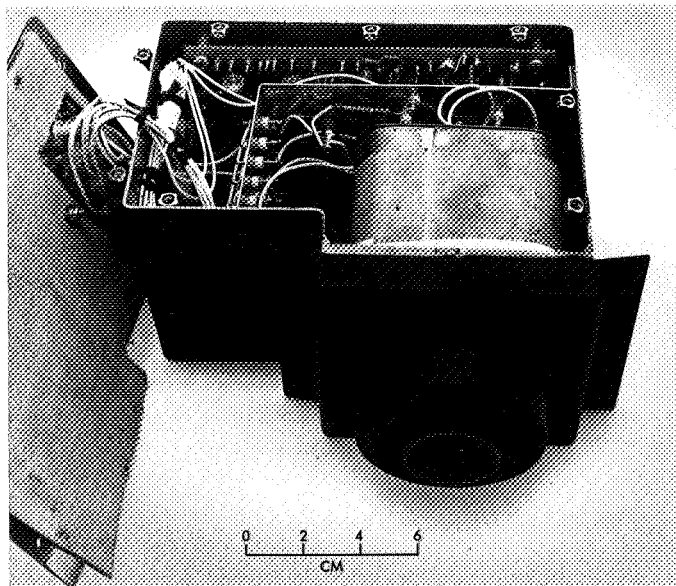
Fig. 41. SPET pulsed plasma thruster (photo courtesy of General Electric)
