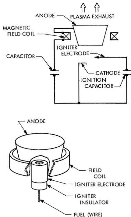
Fig. 43. Pulsed vacuum-arc thruster schematic
