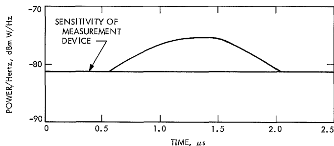
Fig. 39. Radio frequency interference from an early LES-7-type thruster
