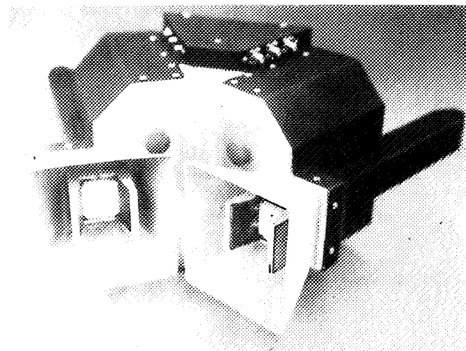
Fig. 38. LES-7 pulsed plasma thruster (photo courtesy of Fairchild-Hiller)
