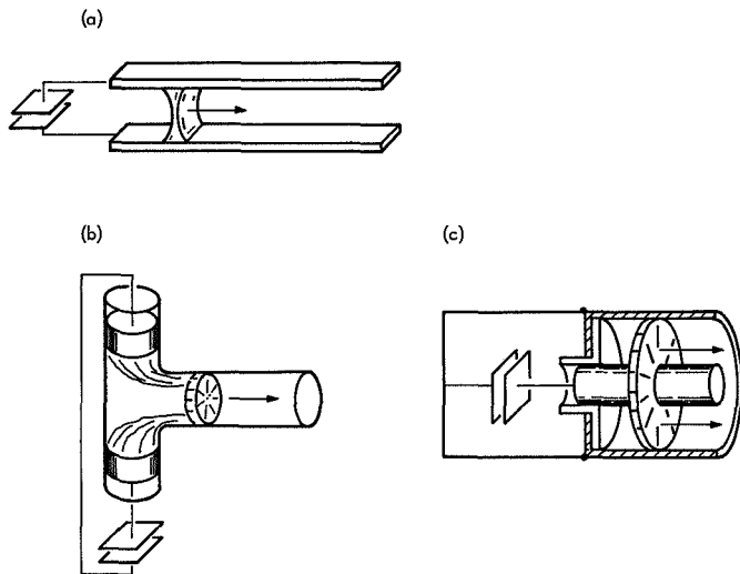
Fig. 31. Various pulsed plasma accelerators: (a) parallel-rail accelerator; (b) T tube; (c) coaxial gun (photo courtesy of R. G. Jahn in Physics of Electric Propulsion )
