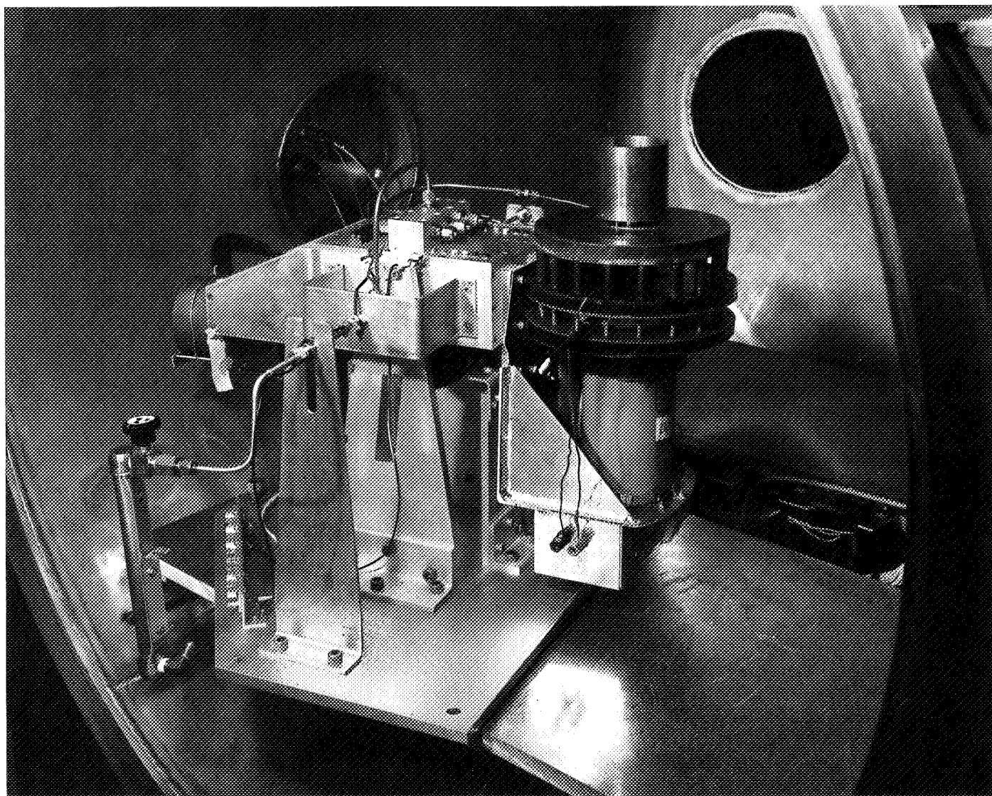
Fig. 45. TRW pulsed inductive thruster (photo courtesy of TRW Systems Group)
