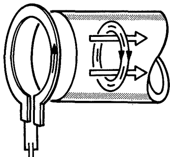
Fig. 32. Pulsed inductive accelerator loop inductor geometry (photo courtesy of R. G. Jahn in Physics of Electric Propulsion )
