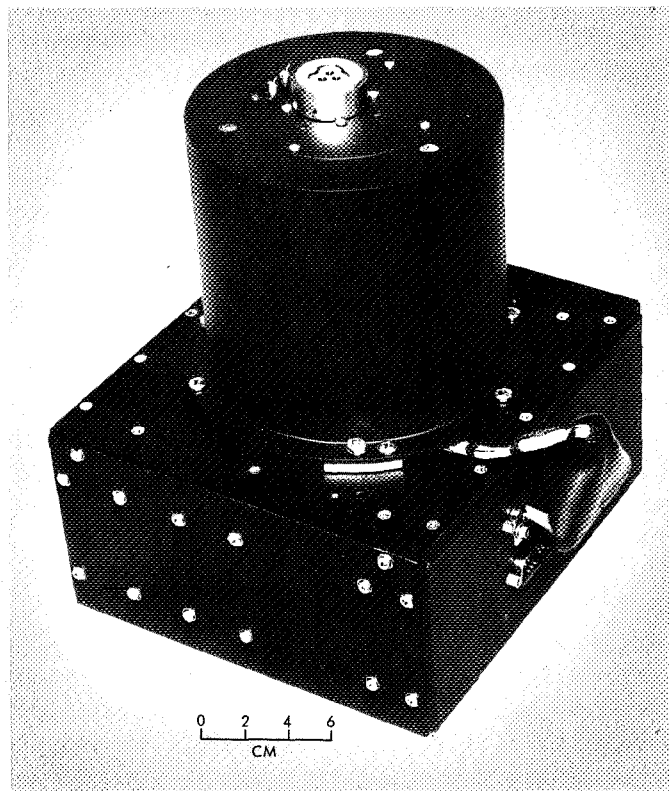
Fig. 23. Colloid microthruster system (photo courtesy of TRW Systems Group)
