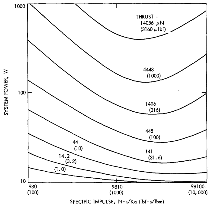
Fig. 8. Effect of system power and thrust on optimum specific impulse of electron-bombardment thrusters (Ref. 20).
