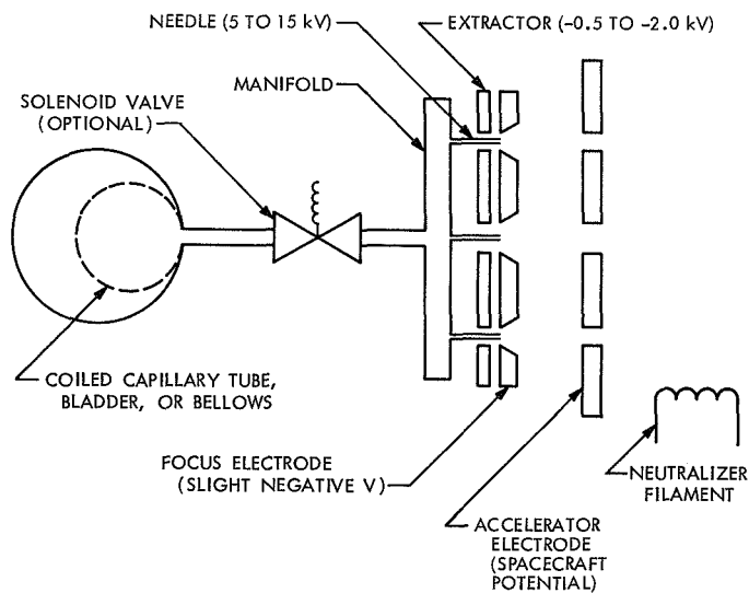
Fig. 19. Conceptual diagram of a colloid thruster
