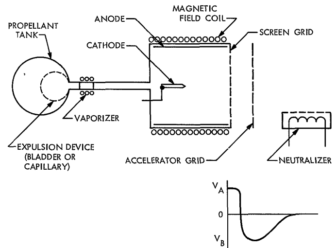
Fig. 2. Conceptual diagram of the electron-bombardment thruster
