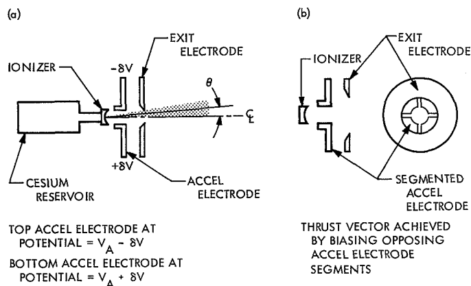
Fig. 4. Electrostatic beam deflection (a) of a linear strip contact-ion thruster, and (b) of a button contact-ion thruster
