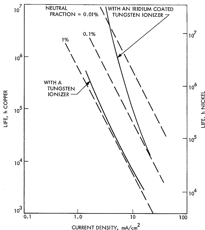
Fig. 12. Erosion of the accelerator electrode due to charge exchange ion bombardment (Ref. 19)
