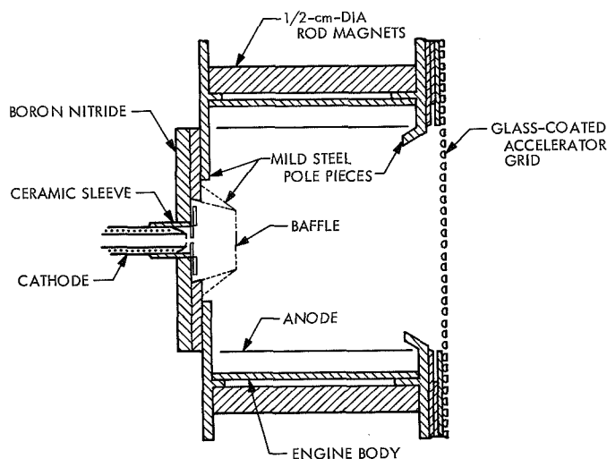
Fig. 18. Five-cm mercury bombardment thruster discharge chamber (representative of HRL and LeRC designs)
