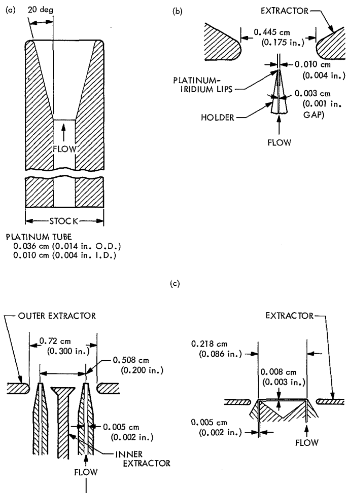
Fig. 20. Geometry of needles and slits: (a) standard needles, (b) linear slits, and (c) annular slits
