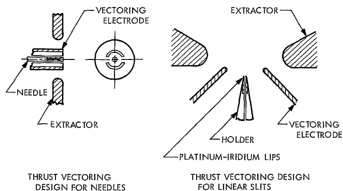
Fig. 22. Electrostatic beam deflection of colloid thrusters
