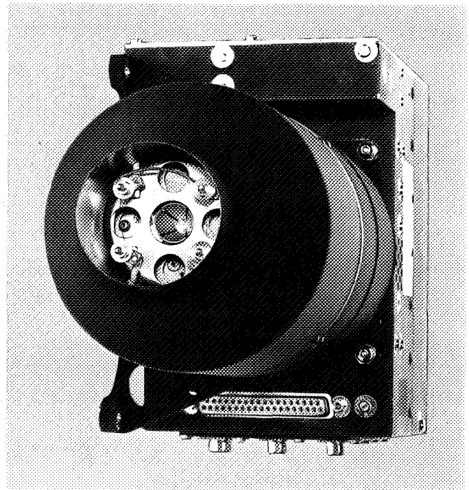
Fig. 10. EOS ATS-D and -E contact-ion microthruster (photo courtesy of EOS)
