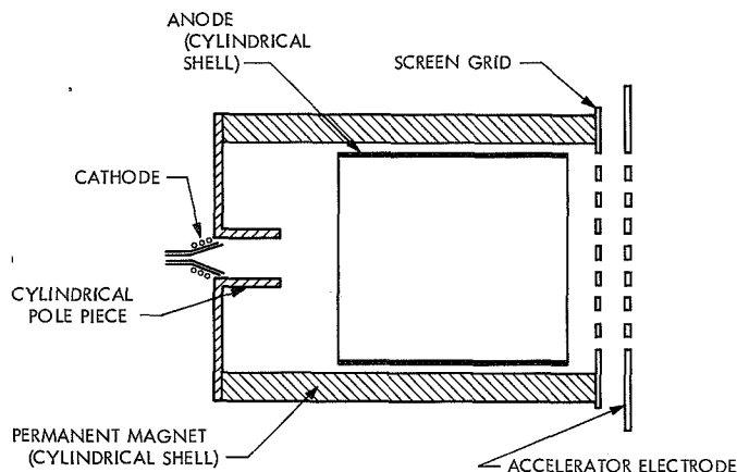
Fig. 15. EOS 445- \mu\text{N} (100- \mu\text{lbf} ) cesium electron-bombardment thruster discharge chamber
