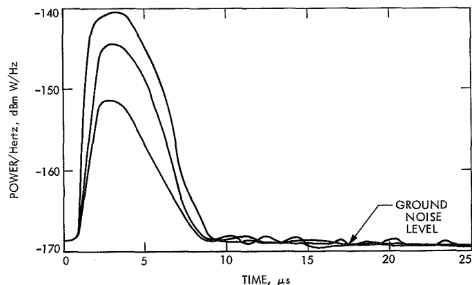
Fig. 37. Radio frequency interference from a LES-6 thruster at UHF frequency
