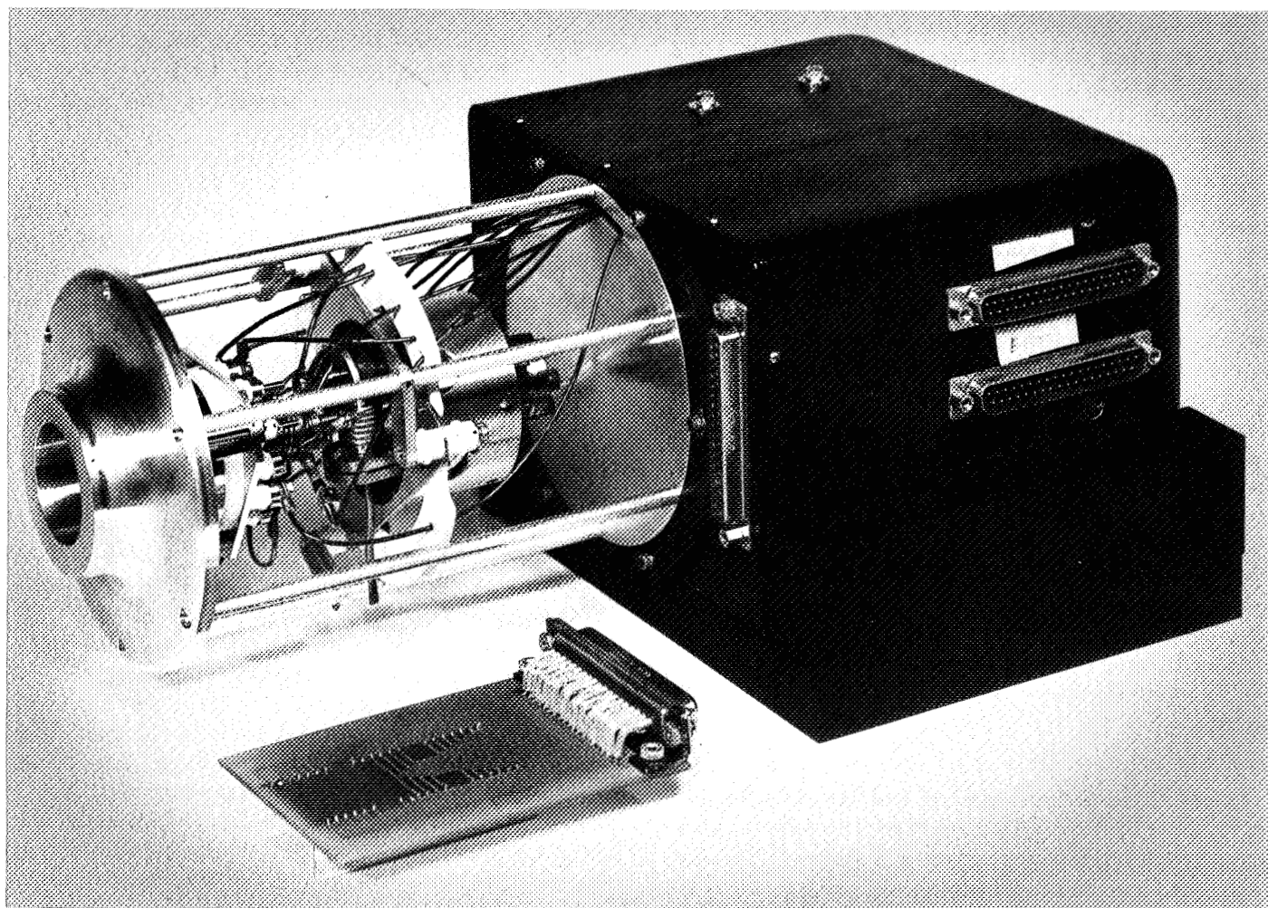
Fig. 11. HRL contact-ion microthruster (photo courtesy of HRL)
