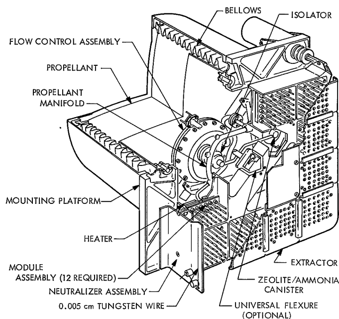
Fig. 24. TRW 4.45-mN (1-mlbf) colloid ADP thruster concept
