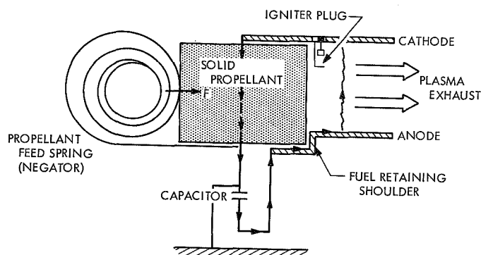
Fig. 36. LES-6 thruster schematic
