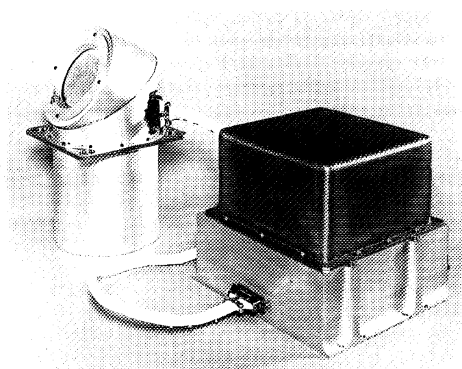
Fig. 16. EOS 4.45-mN (1-mlbf) cesium bombardment thruster (photo courtesy of EOS)
