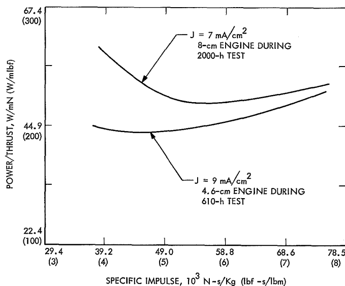
Fig. 3. Power-to-thrust vs specific impulse for contact-ion thrusters (Ref. 19)
