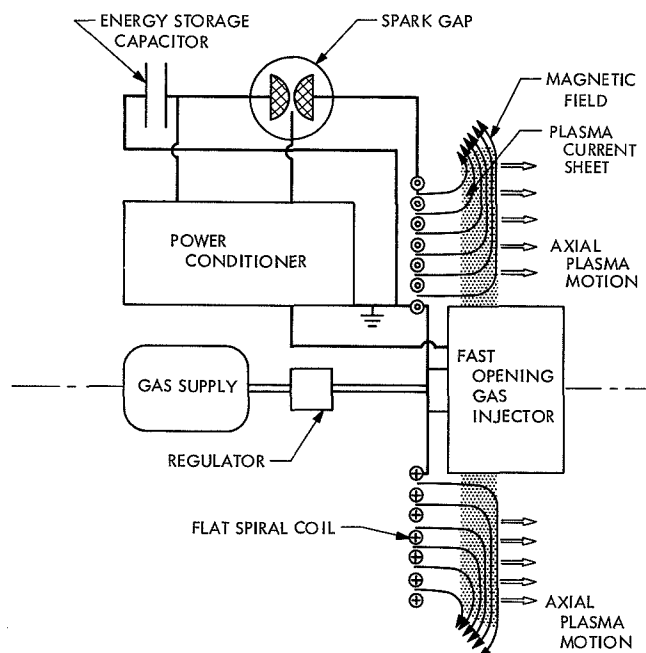
Fig. 46. Pulsed inductive thruster schematic
