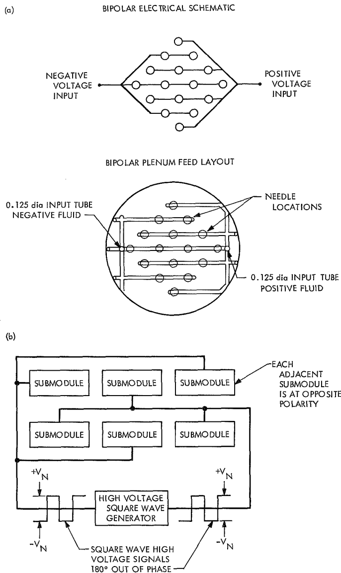
Fig. 21. Bipolar colloid arrays: (a) conventional array, and (b) block diagram of alternating pulse array
