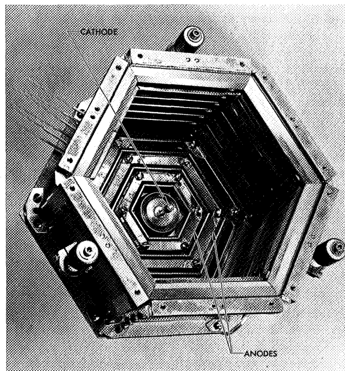
Fig. 6. Discharge chamber geometry of the EOS magneto-electrostatic containment (MESOC) thruster (photo courtesy of EOS)
