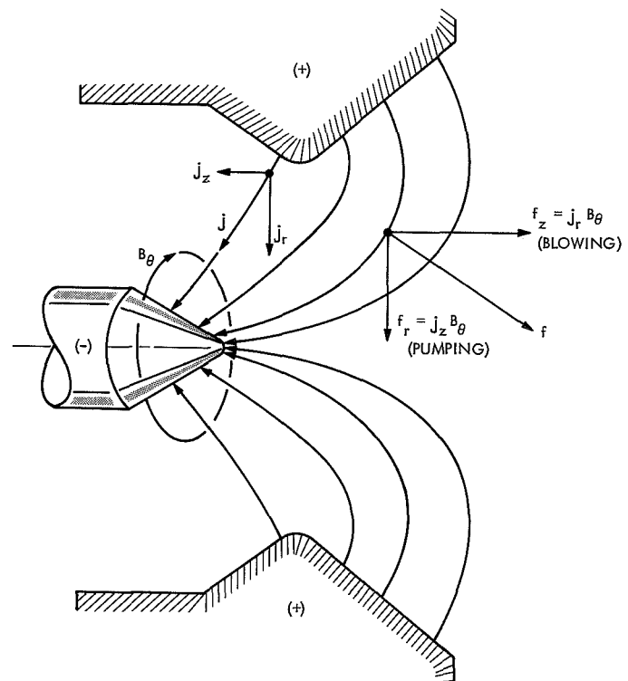
Fig. 26. Acceleration mechanism of a self-field MPD thruster
