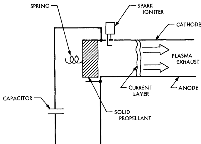
Fig. 33. Conceptual diagram of the pulsed plasma thruster
