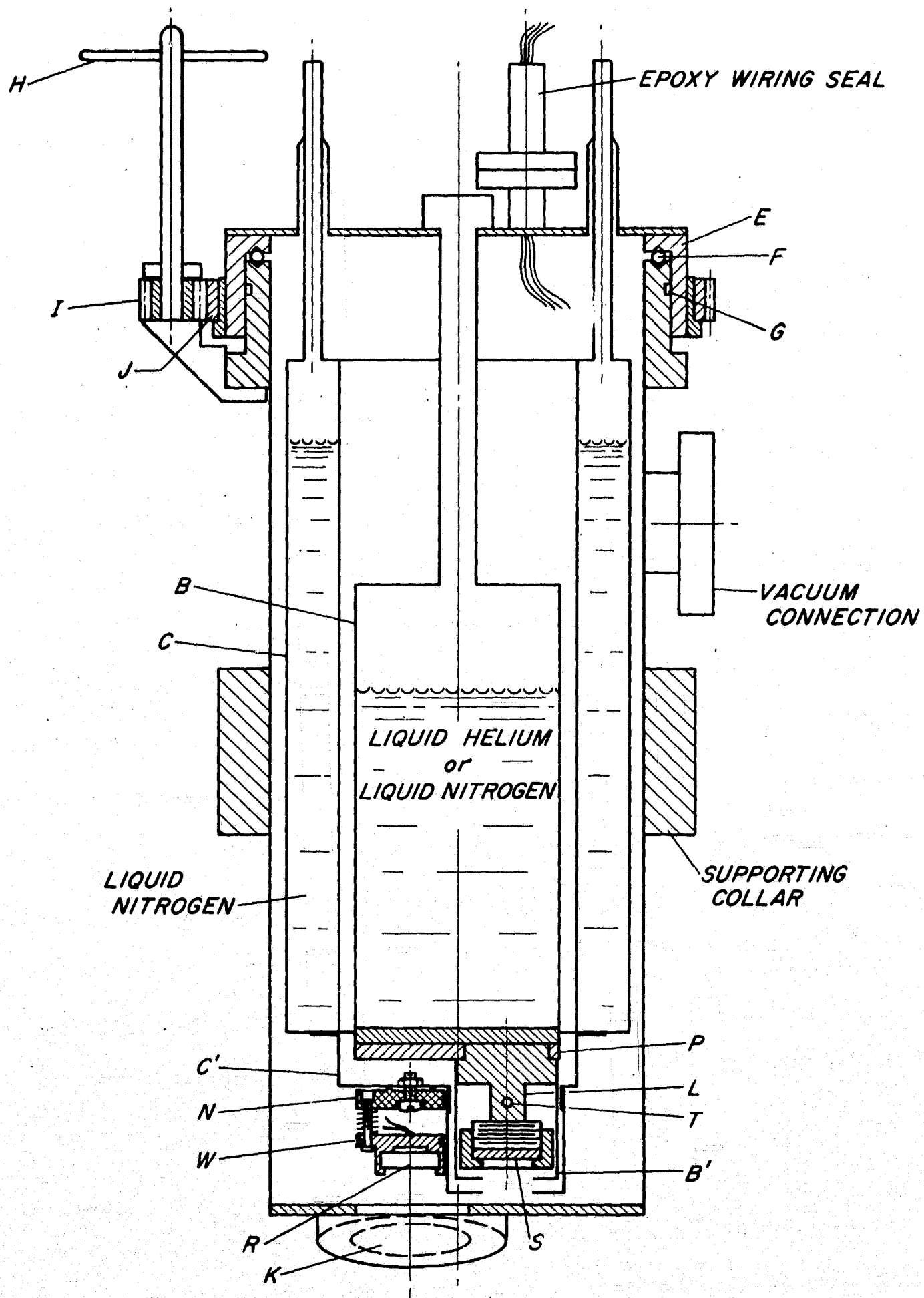
Figure 4. Cryostat
