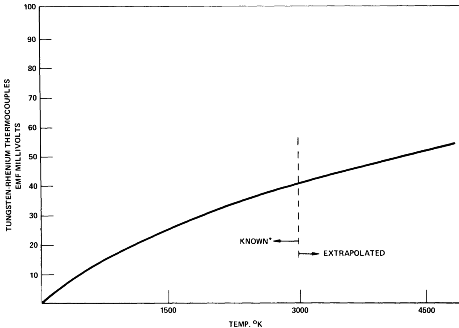
FIGURE 6. TUNGSTEN RHENIUM THERMOCOUPLE CONVERSION DATA
