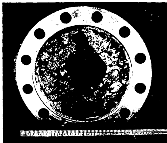
NOZZLE EROSION
