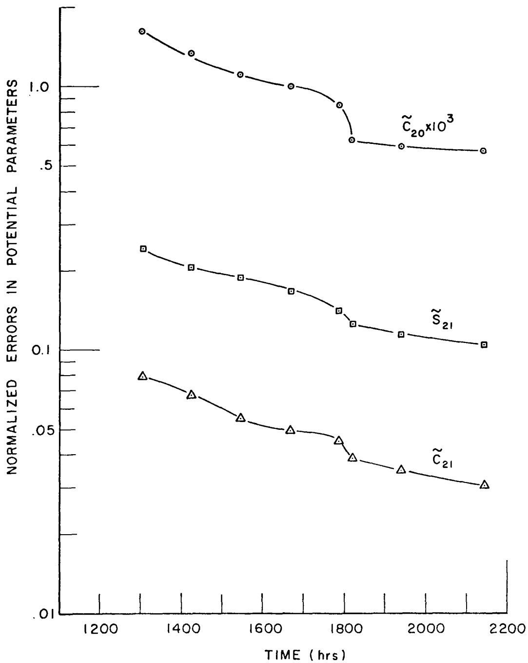
Figure 17: Normalized error in the harmonic coefficients as a function of sighting interval. Orbit No. 2.
