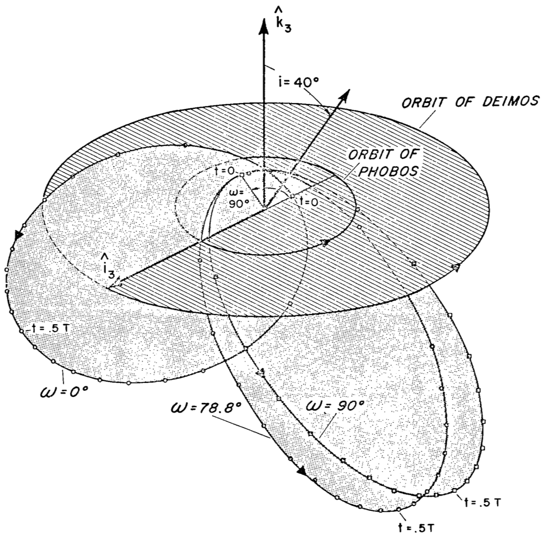
Figure 7: Geometry of three spacecraft orbits, each of which has the same orbital elements except for \omega . \Omega = 180^\circ , i = 40^\circ
