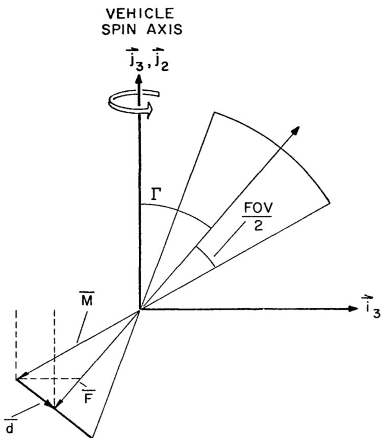
Figure 35: Orientation of optical system in spacecraft
