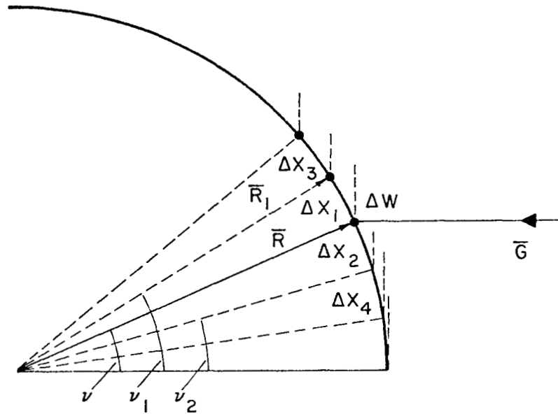
Figure 33: Improved approximation for large angles of dv .
