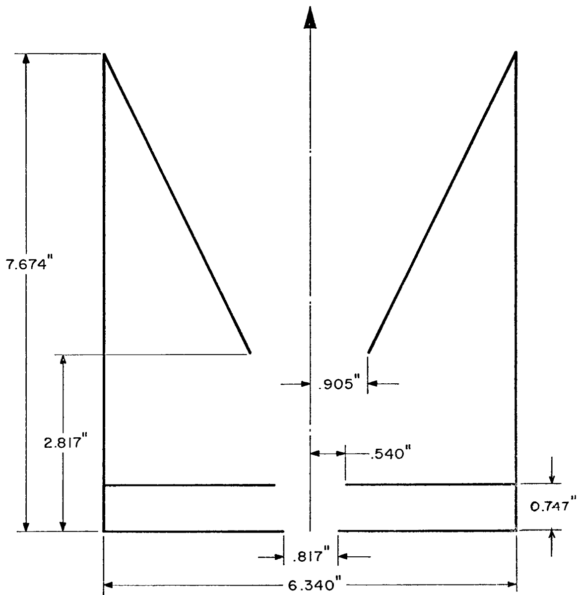
Figure 40: Shield dimensions.
