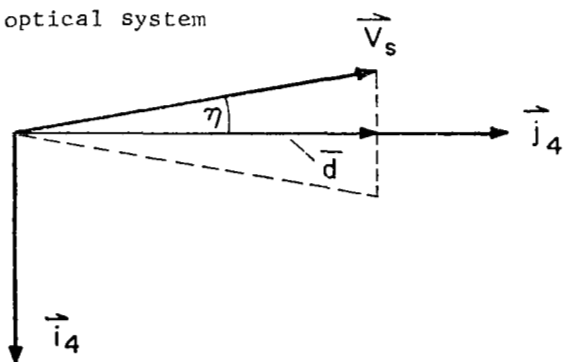
Figure 36: Orientation of sensor slit(s) in focal plane
