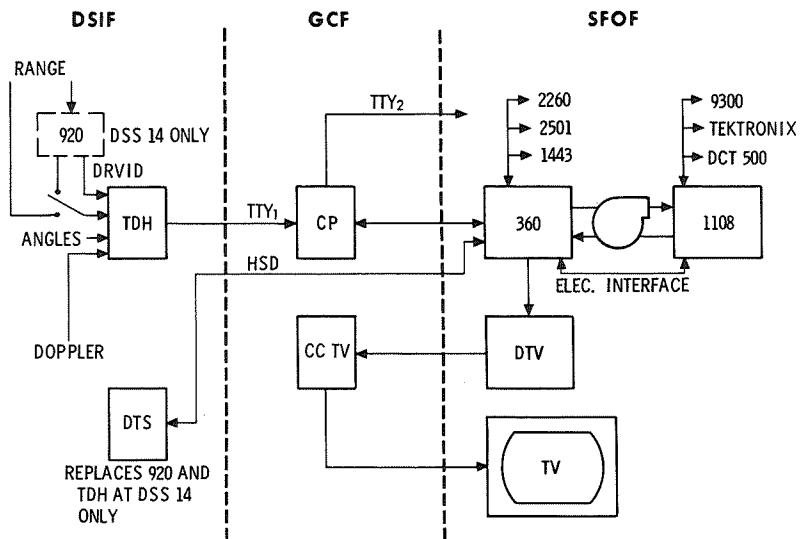
Fig. 4. Tracking system
