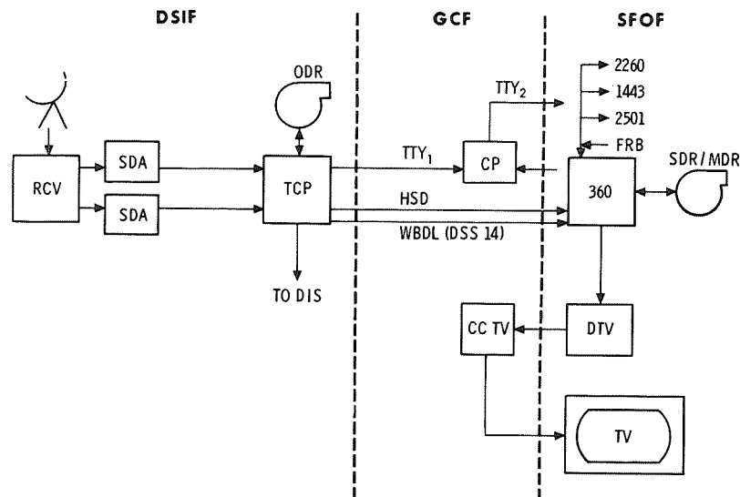
Fig. 1. Telemetry system
