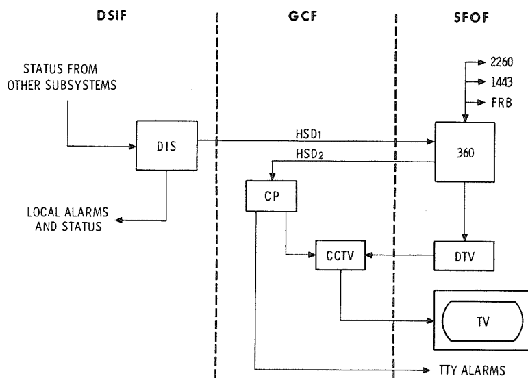
Fig. 6. Monitor system
