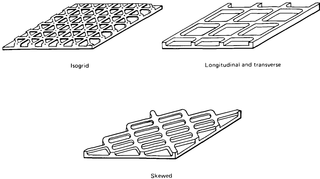
Figure 2. – Types of waffle stiffening.
