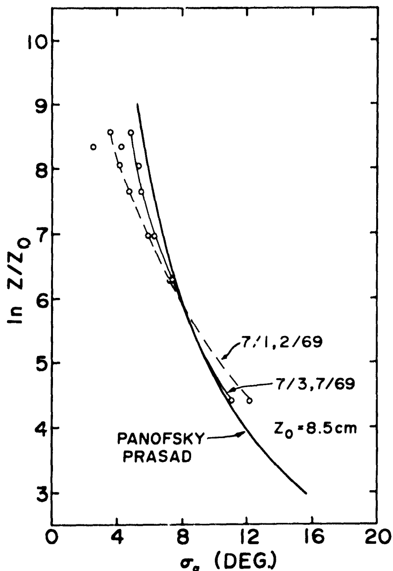
Figure 12. Same as figure 11 for z_0 = 8.5 cm.
