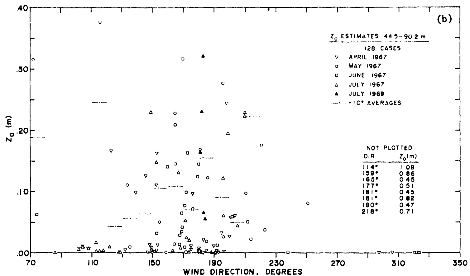
Figure 9. Roughness length estimates vs. wind direction: (a) from 7.0 and 44.5 m points; (b) from 44.5 and 90.2 m points; (c) from regression line through 7.0, 44.5, and 90.2 m points.
