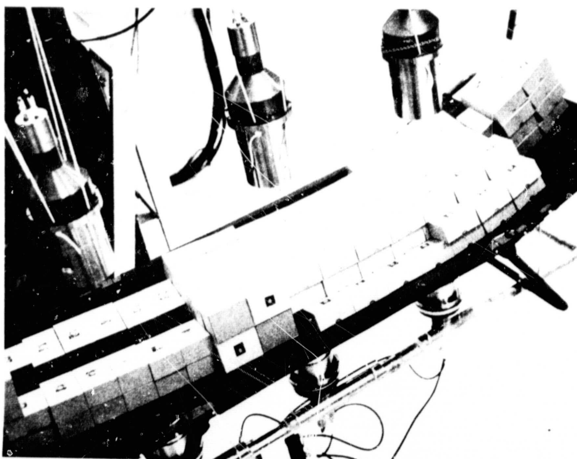
FIGURE 3 141 Pound Phantom in Place in the NASA-MSC Whole Body Counter
