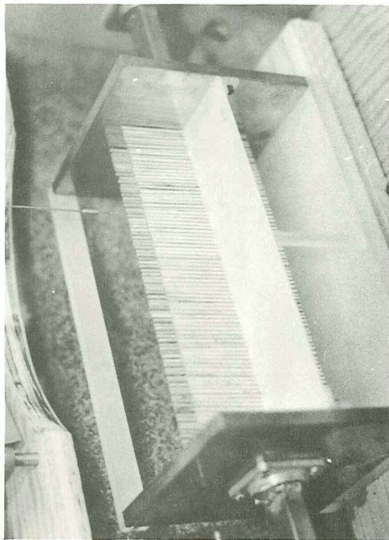
Figure 3.5 Prototype guide, narrow spacing.
