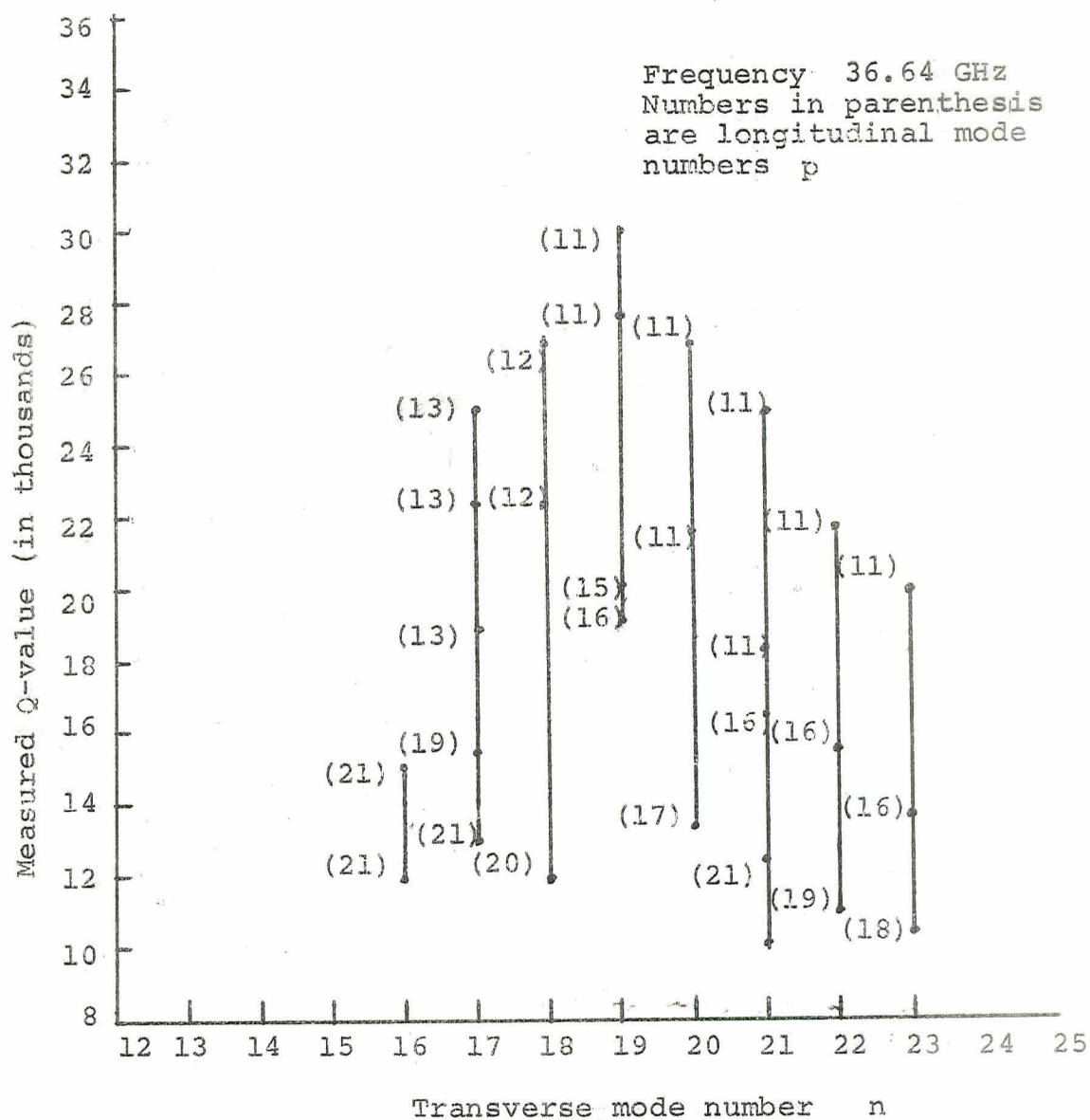
Fig. 6 Quality factor Q versus transverse mode number n .
