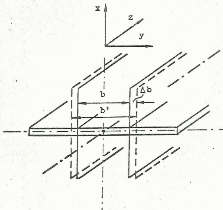
Fig. 2. Equivalent widths of waveguides.
