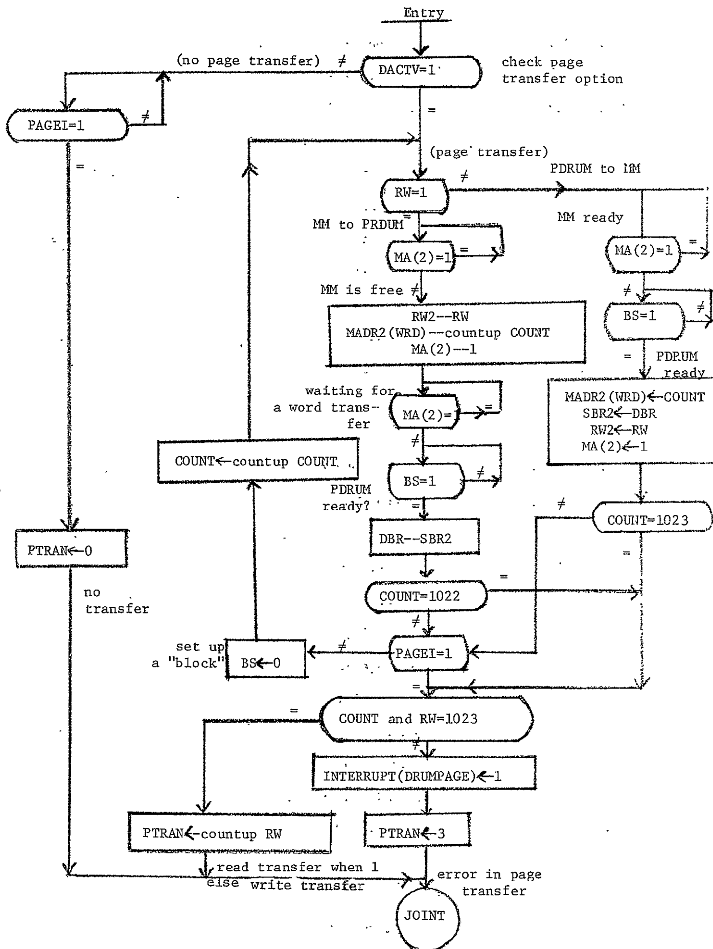
Fig. 20 Drum read/write Subsequence
