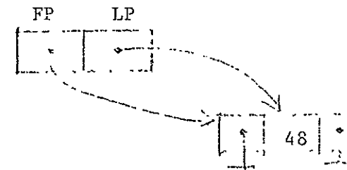
Fig. 28 Manipulation of Sector Queues 0, 1, and 15
