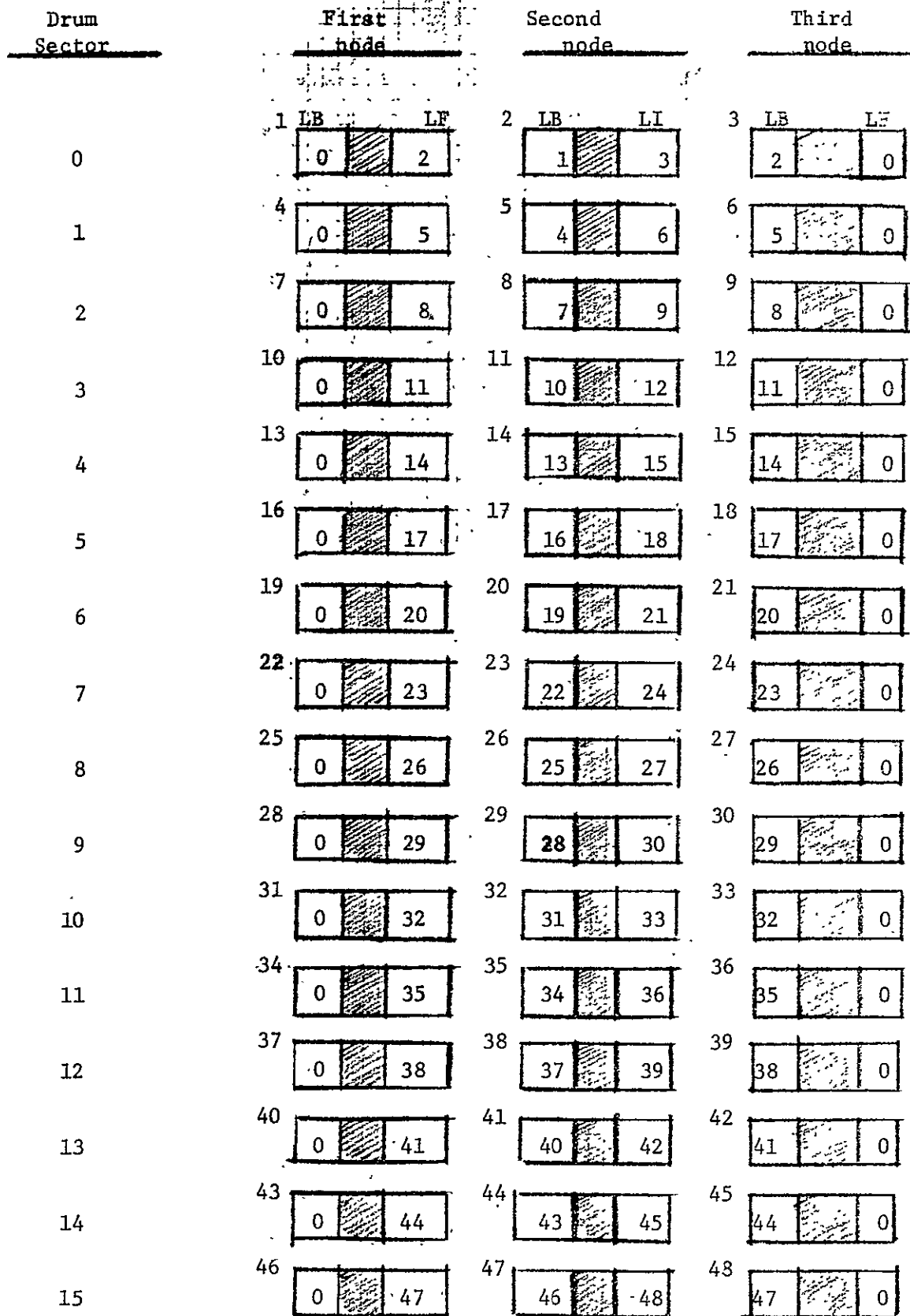
Fig. 24 Initial Forward and Backward Links in the Page Descriptors Which Form the 16 Sector Queues
