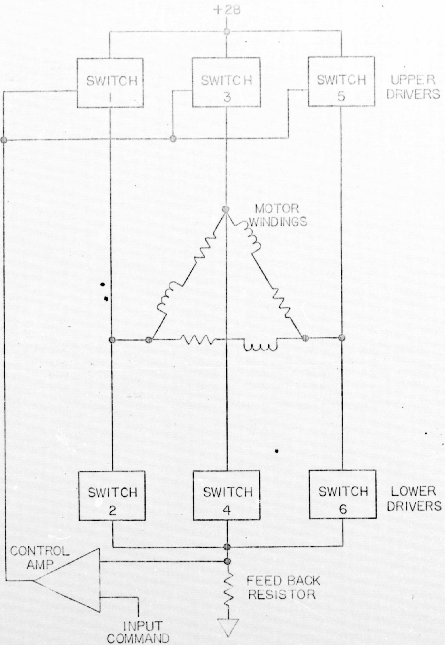
FIGURE 1. DRIVER SYSTEM
