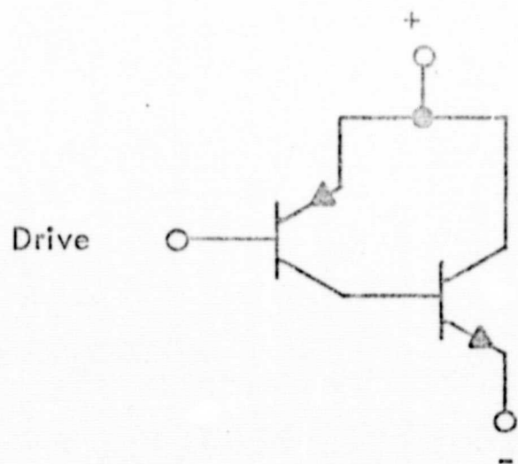
Figure 9. OUTPUT DRIVER STAGE
