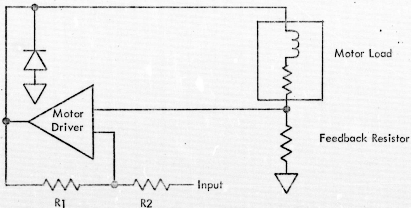
Figure 10. SWITCHING REGULATOR
