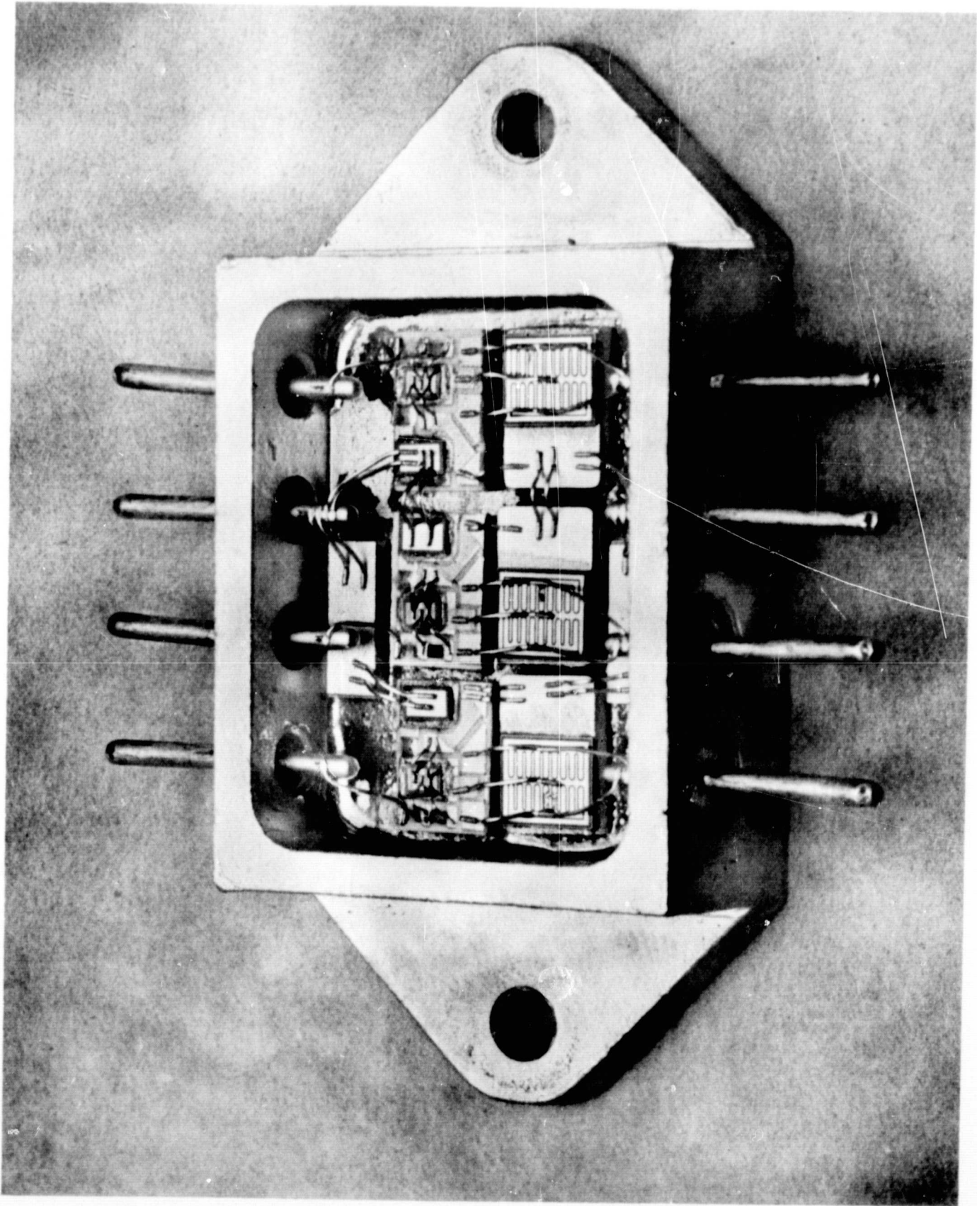
Figure 16. HIGH POWER DRIVER
