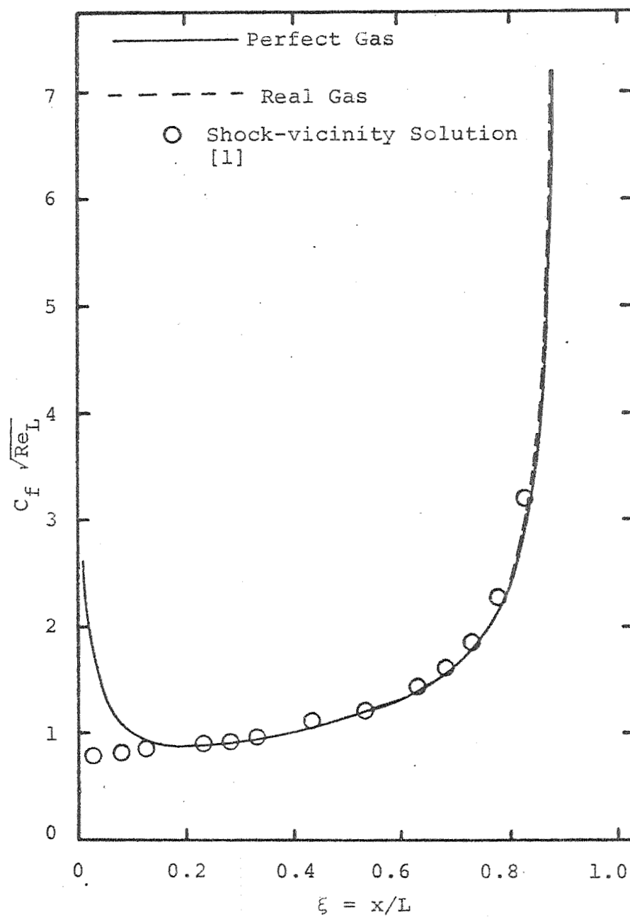
Figure 8. Comparison of Skin-Friction Coefficient with Shock-Vicinity Solution [1] for M_s = 1.6 .
