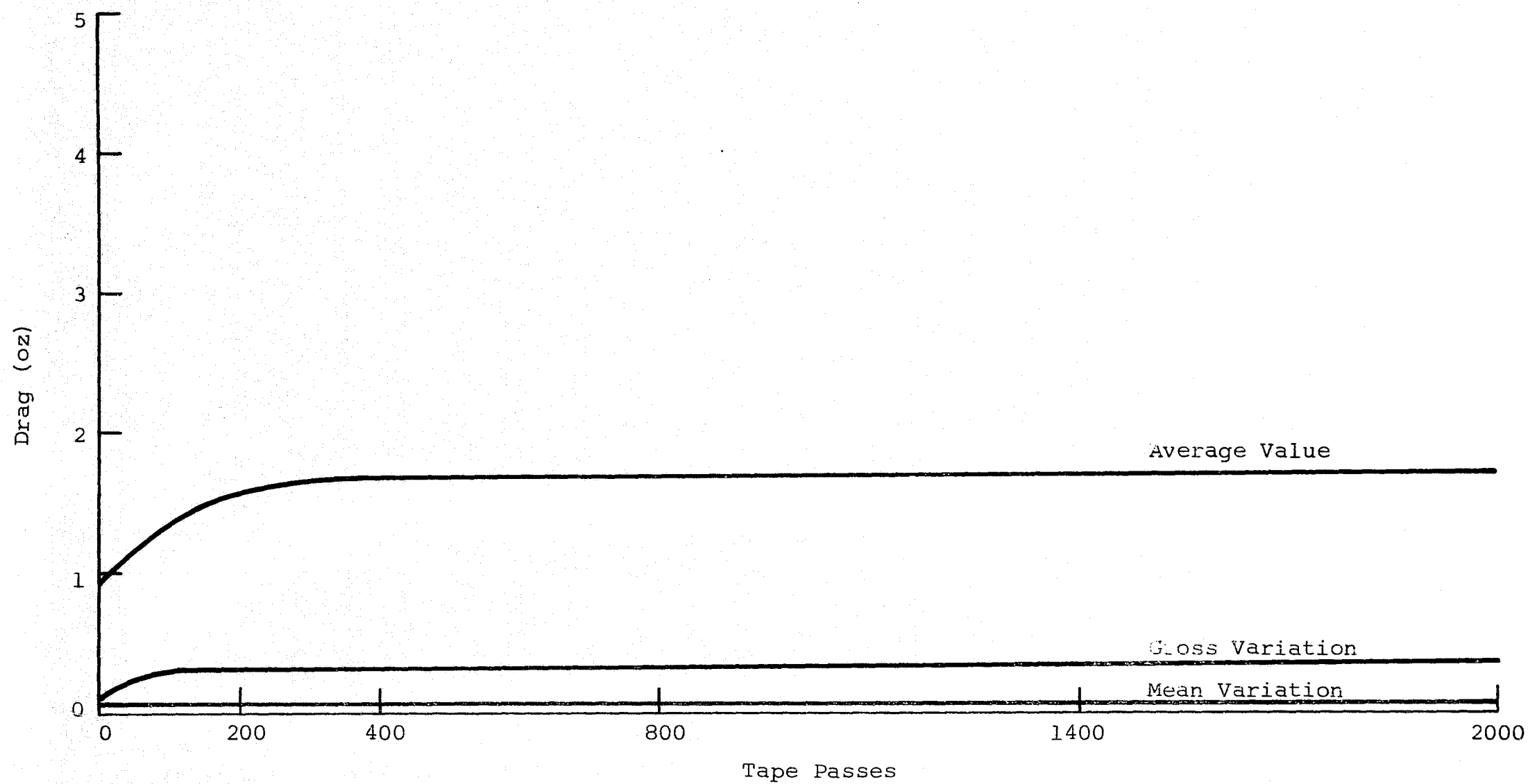
Fig. 6e AVERAGE, MEAN, AND GROSS VARIATIONS IN DRAG AGAINST NUMBER OF TAPE PASSES FOR TEST NUMBER 5 AT A REPRODUCE TAPE SPEED OF 0.15 INCHES PER SECOND
