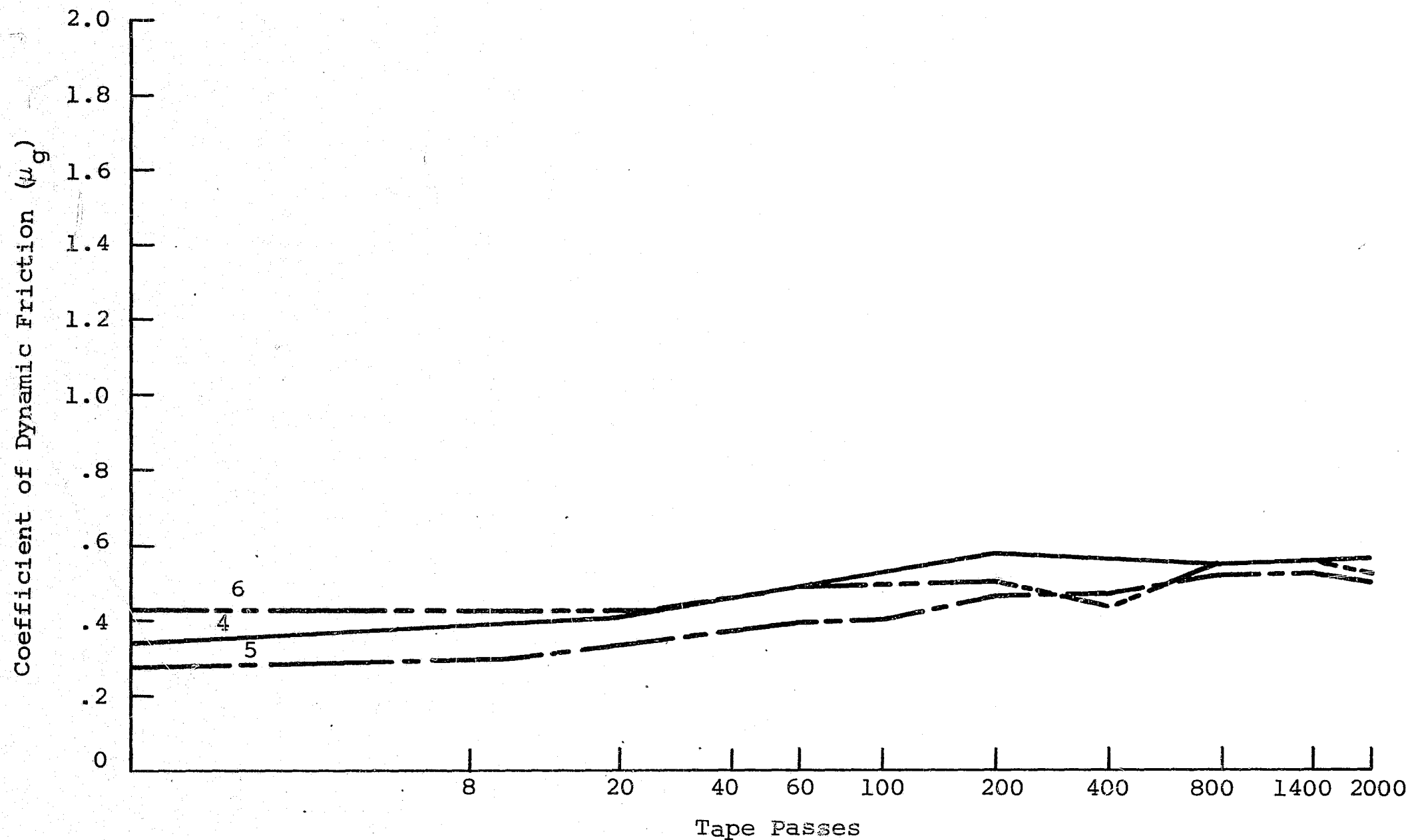
Fig. 8b CHANGE IN THE COEFFICIENT OF DYNAMIC FRICTION AGAINST NUMBER OF TAPE PASSES MEASURED AT A REPRODUCE TAPE SPEED OF 0.15 INCHES PER SECOND
