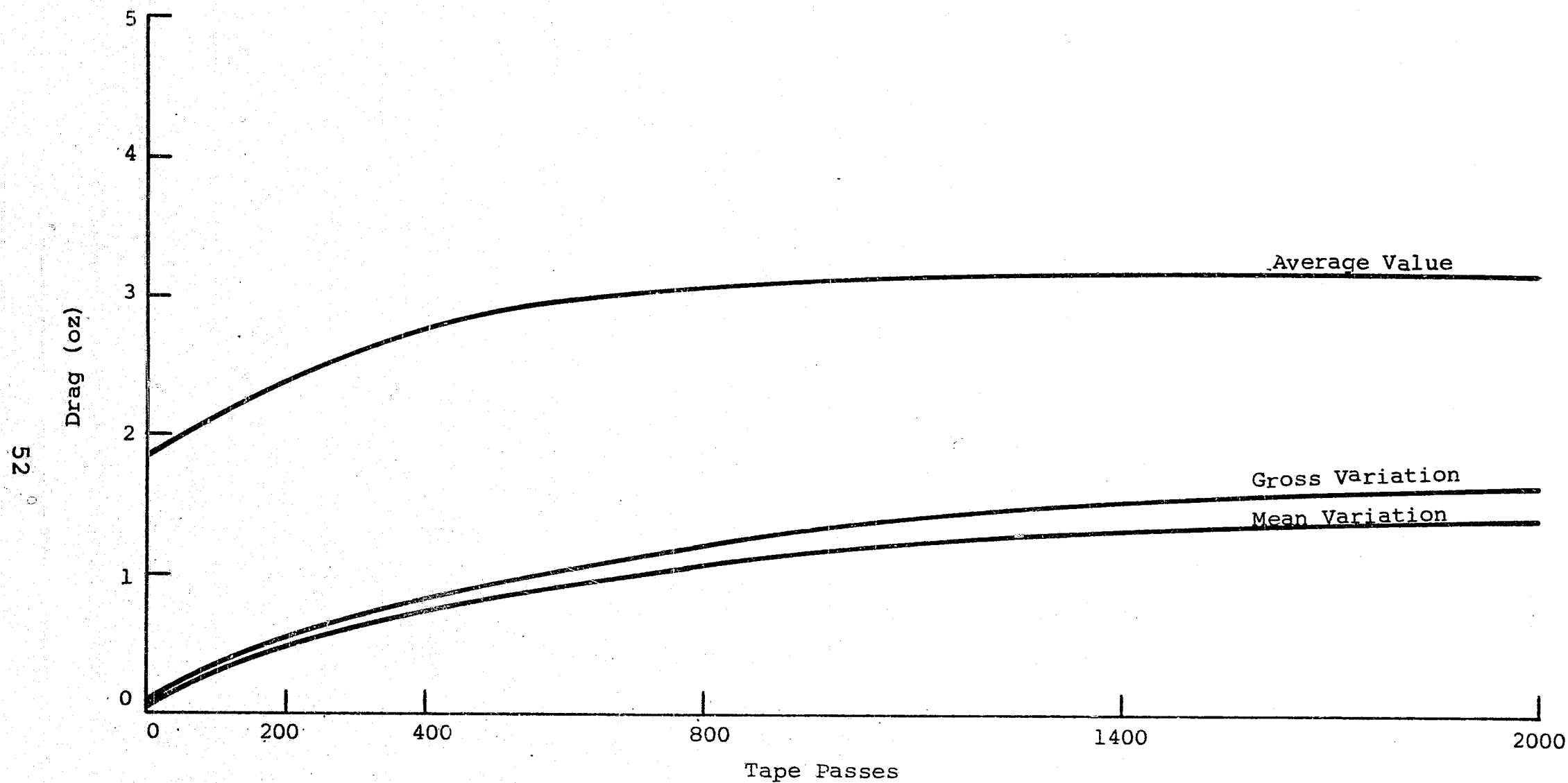
Fig. 6k AVERAGE, MEAN, AND GROSS VARIATIONS IN DRAG AGAINST NUMBER OF TAPE PASSES FOR TEST NUMBER 11 AT A REPRODUCE TAPE SPEED OF 0.15 INCHES PER SECOND
