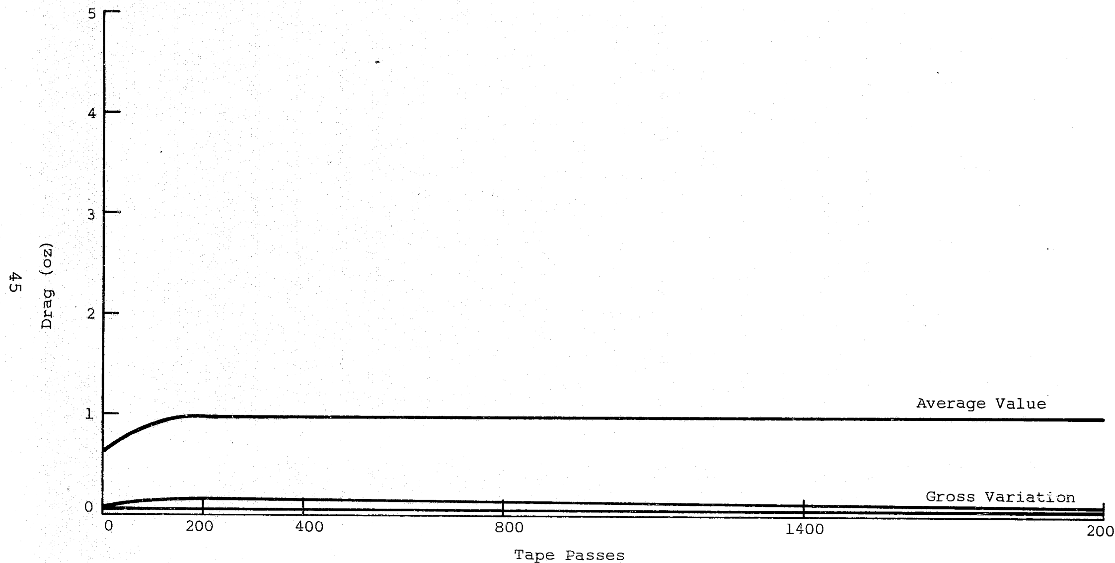
Fig. 6d AVERAGE, MEAN, AND GROSS VARIATIONS IN DRAG AGAINST NUMBER OF TAPE PASSES FOR TEST NUMBER 4 AT A REPRODUCE TAPE SPEED OF 0.15 INCHES PER SECOND
