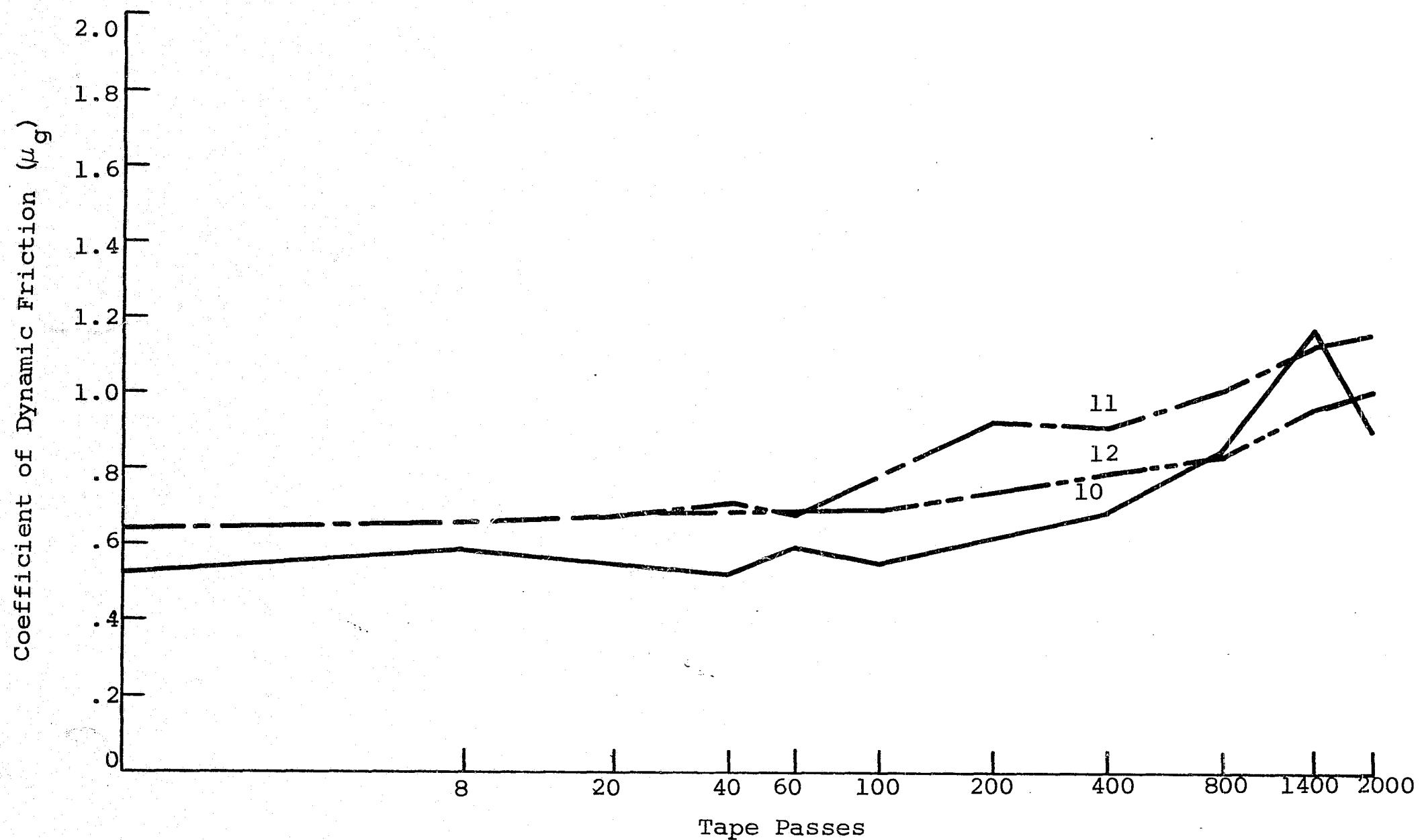
Fig. 8d CHANGE IN THE COEFFICIENT OF DYNAMIC FRICTION AGAINST NUMBER OF TAPE PASSES MEASURED AT A REPRODUCE TAPE SPEED OF 0.15 INCHES PER SECOND
