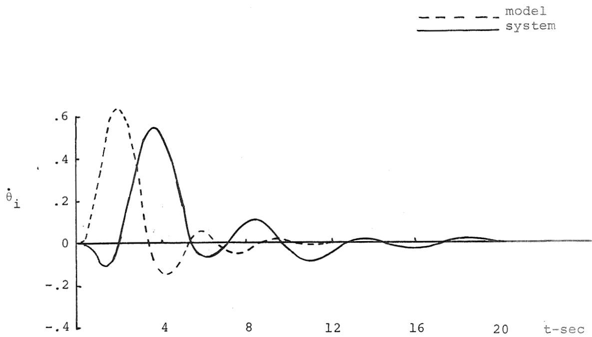
Pitch rate response at gyro station
