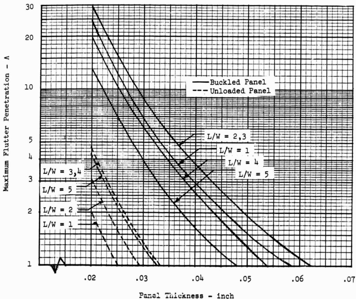
Figure 10 - Maximum Flutter Penetration as a Function of Panel Geometry
