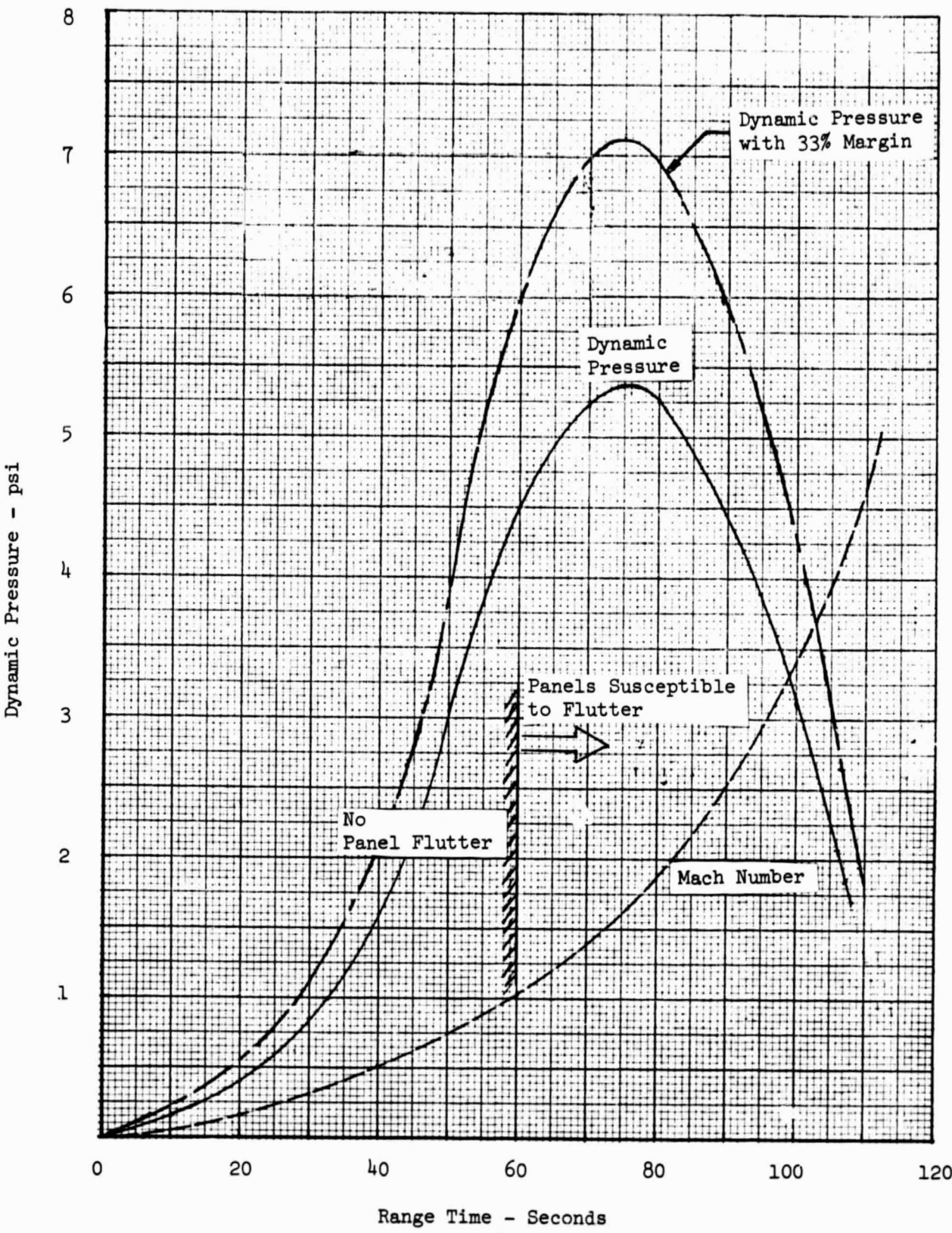
Figure 9 - Apollo/Lunar Trajectory
