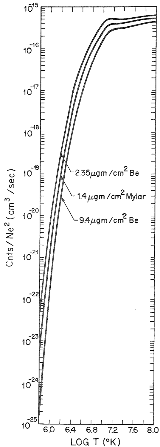
Figure 3-9. Curves of the counting rate integrals of the OSO-IV detector as a function of temperature for the three filters. The integrals are calculated by the OSOINT program. Flat detector response is assumed. The SHI ratios of Figure 3-3 are produced from these integrals.
