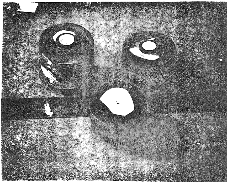
Figure 17b. Photograph of plugs used in adhesive energy apparatus with bovine teeth, approximating analytical model of Figure 4b (Reference 36).
