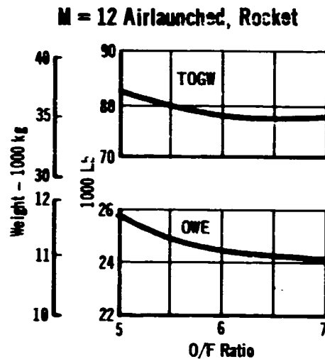
FIGURE 8 EFFECT OF PROPELLANT MIXTURE RATIO
