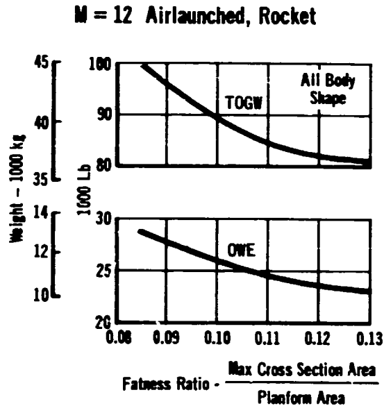
FIGURE 10 EFFECT OF FATNESS RATIO
