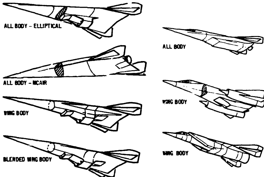
FIGURE 3 VEHICLE CONFIGURATIONS
