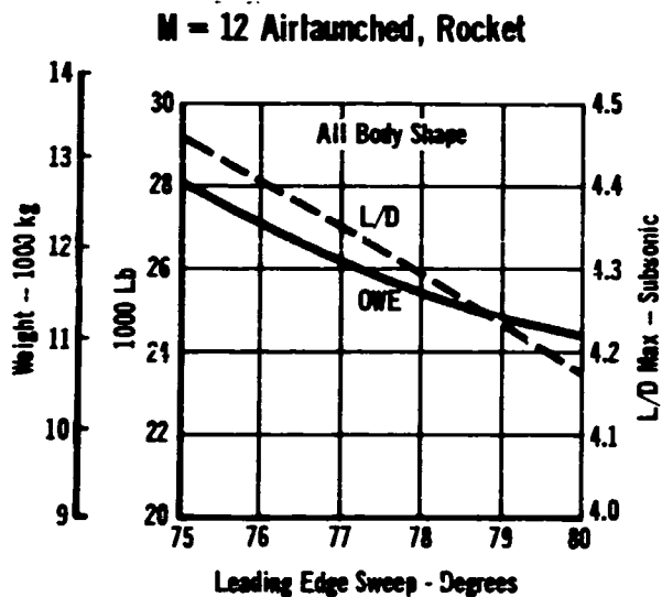
FIGURE 9 EFFECT OF LEADING EDGE SWEEP
