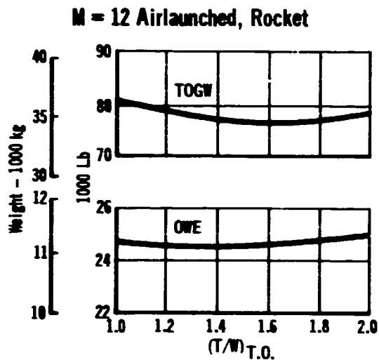
FIGURE 7 EFFECT OF THRUST LOADING
