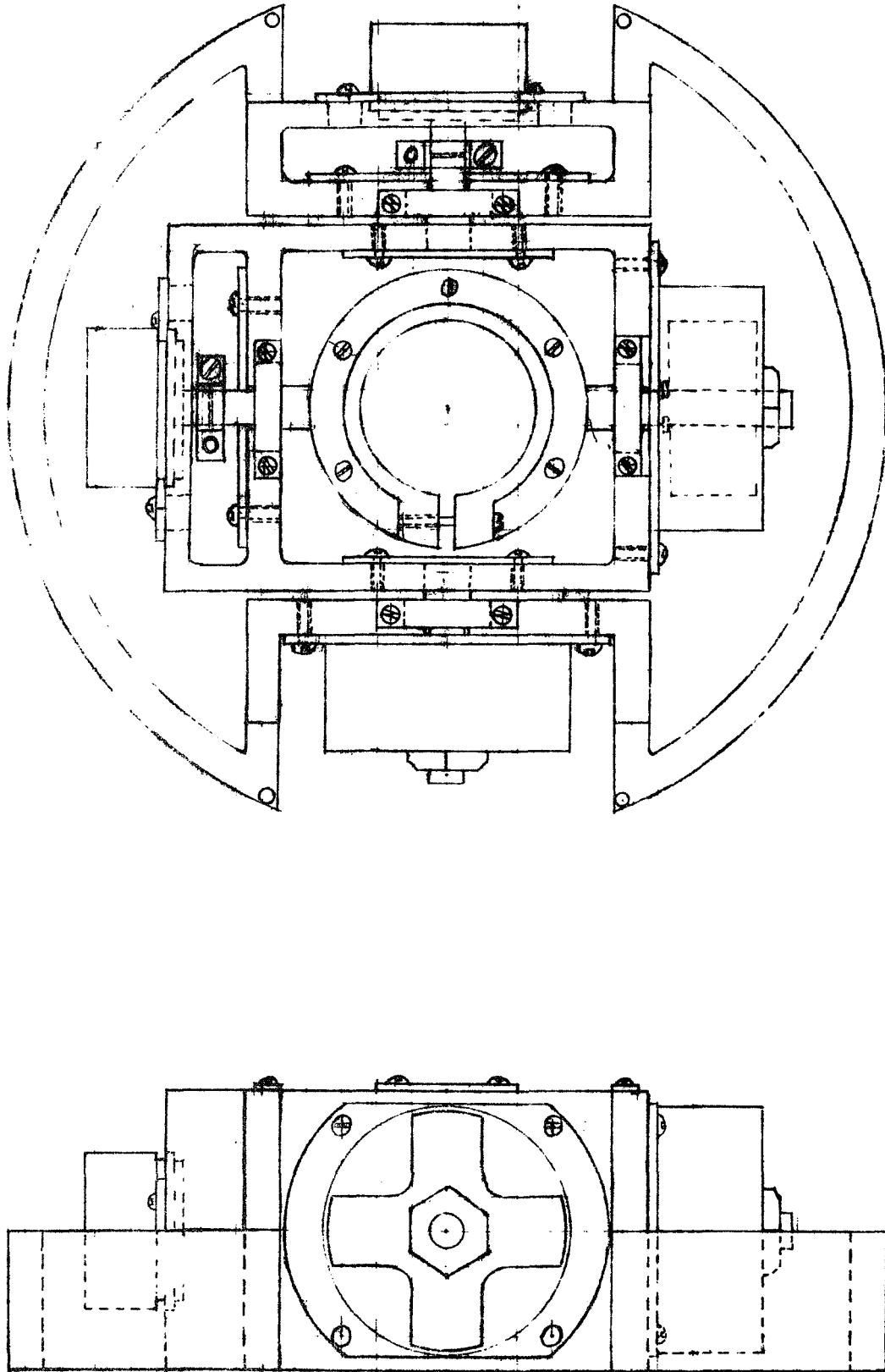
Figure 11. Gimballed Detector Mount Assembly.
