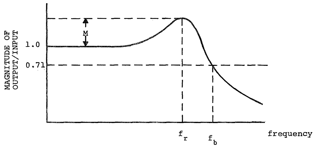
FREQUENCY RESPONSE
