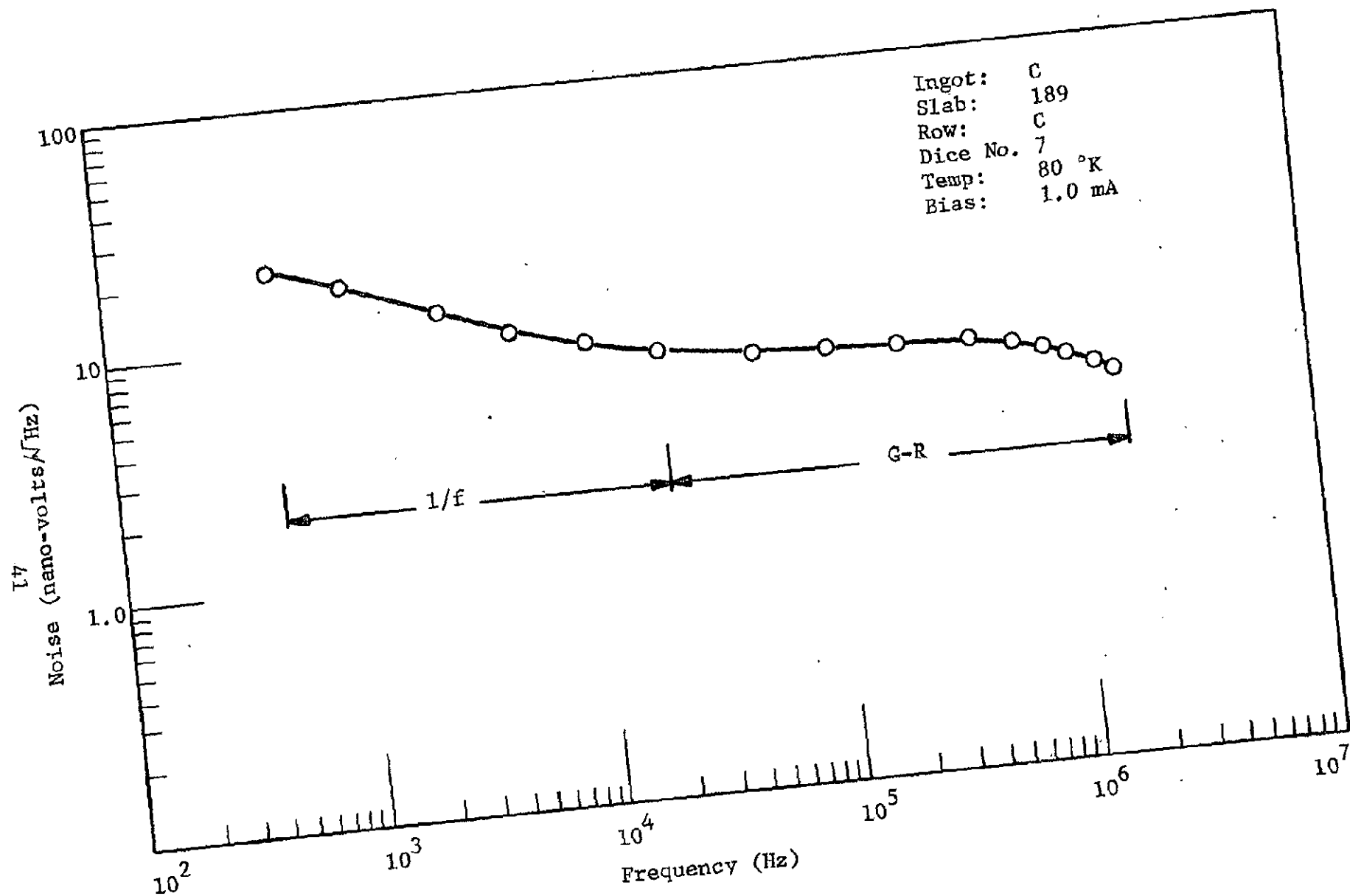
Figure 20 NOISE SPECTRUM
