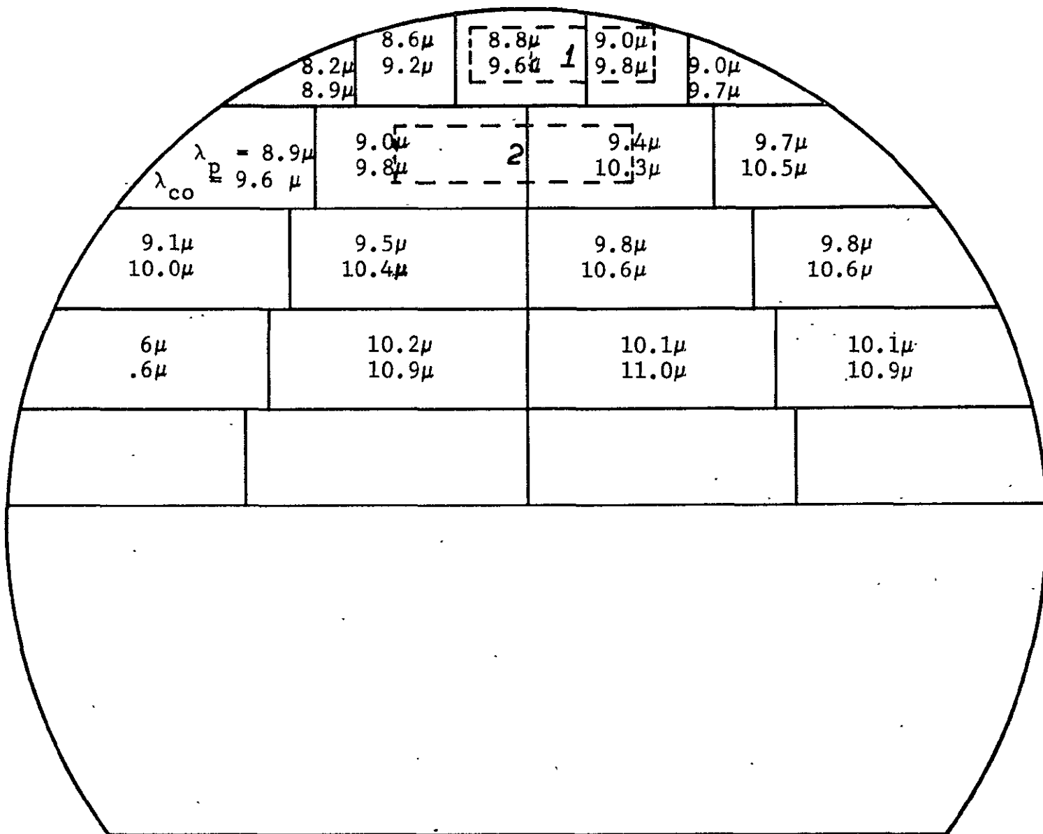
Figure 16. SPECTRAL RESPONSE OF SLAB 145 TO DETERMINE REGIONS OF PROPER WAVELENGTH FOR TOP DETECTORS
