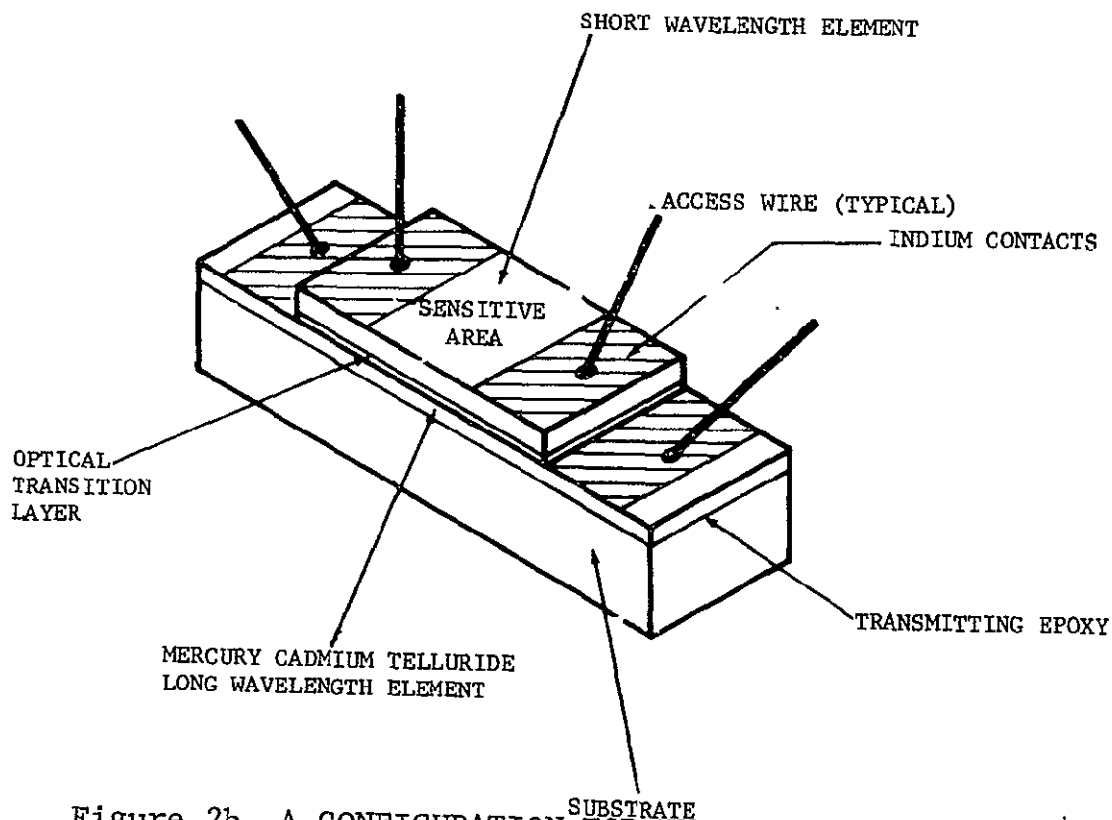
Figure 2b A CONFIGURATION FOR TWO-COLOR DETECTORS (CROSSED)
