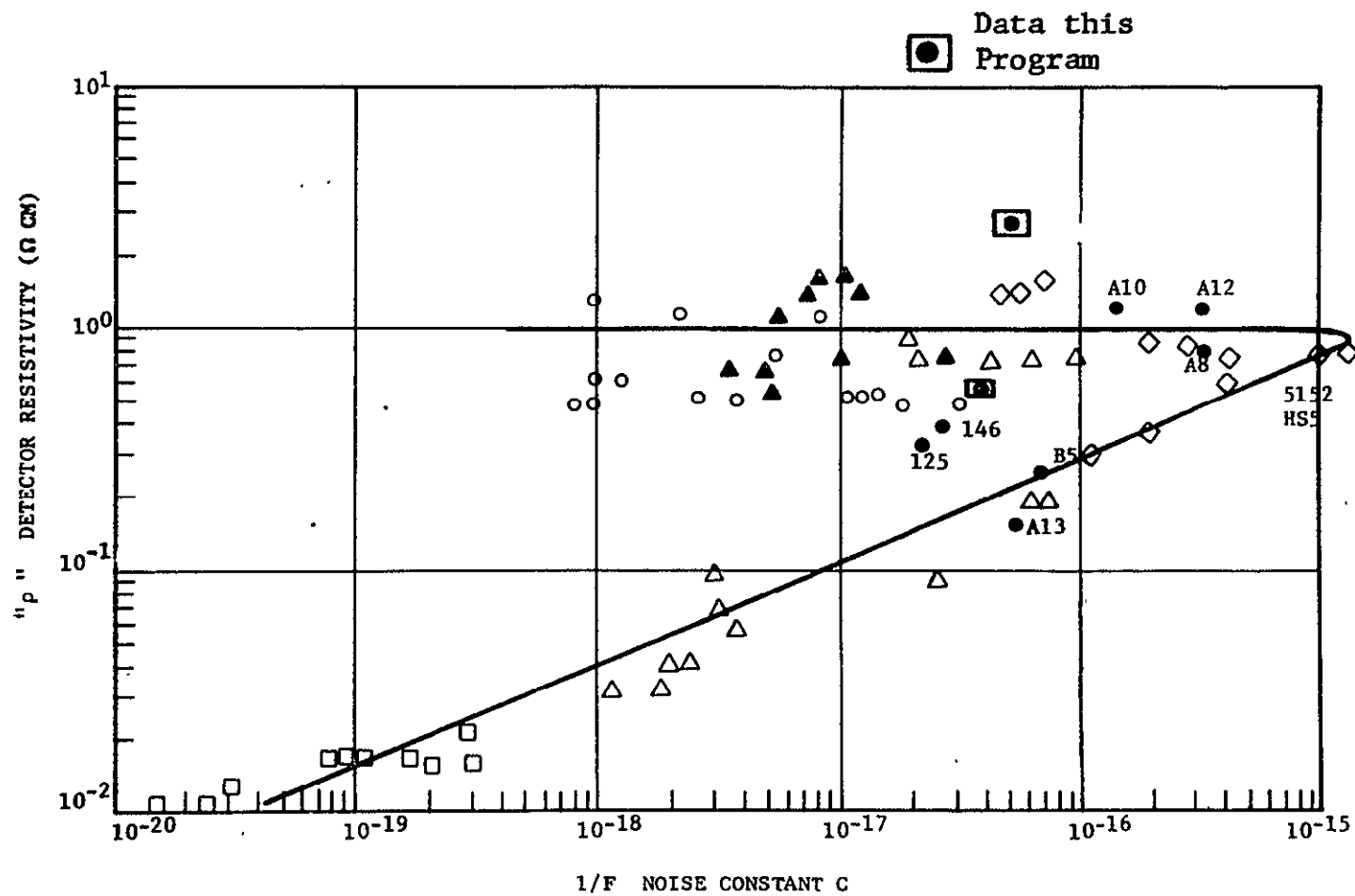
Figure 21 \rho VERSUS 1/f CONSTANT "C"
