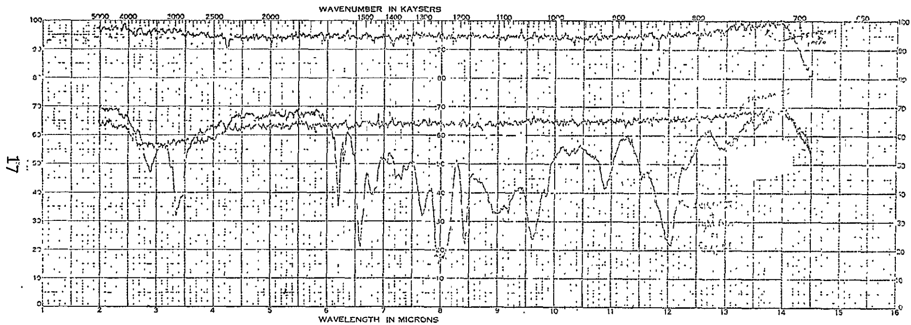
Figure 9. EPOXY G.L. 300 °K
