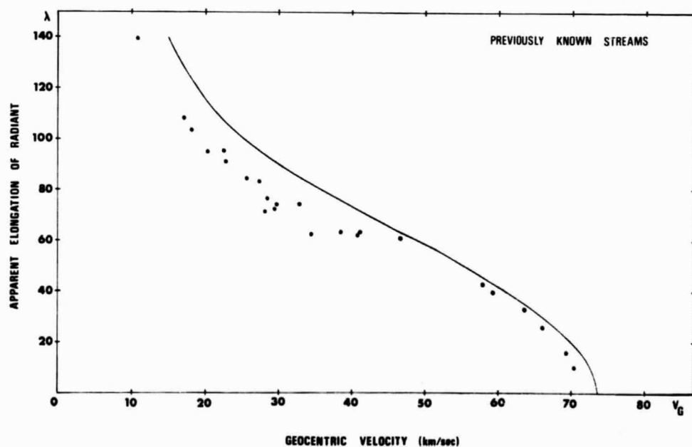
FIGURE 2.—Velocity-elongation diagram for previously known photographic streams.
