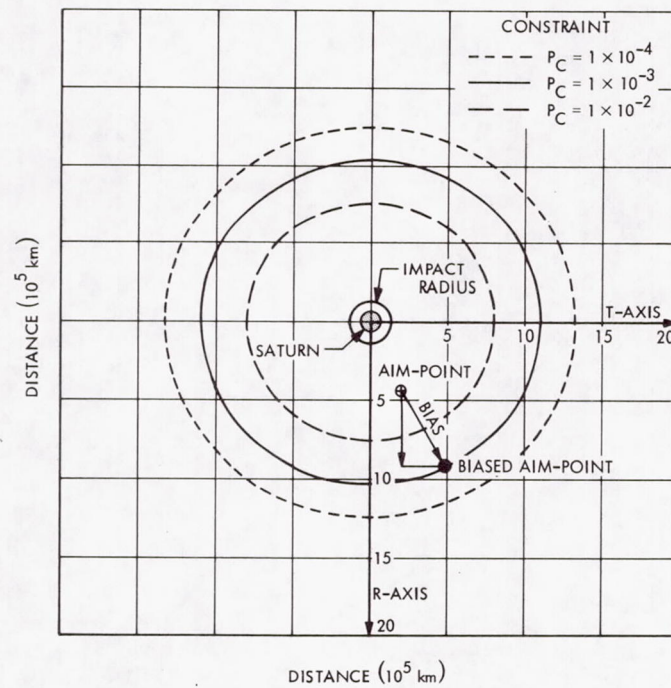
Fig. 3. Impact probability contours at Saturn aim-plane, due to swing-by error at Jupiter, 1977 J-S-P
