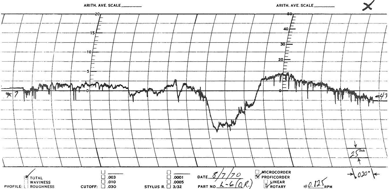
Figure 43. Comparative Profilometer Traces From AISI 440C Outer Race Run With AISI 440C Balls and Chemloy 719 Lubricant (L6)
