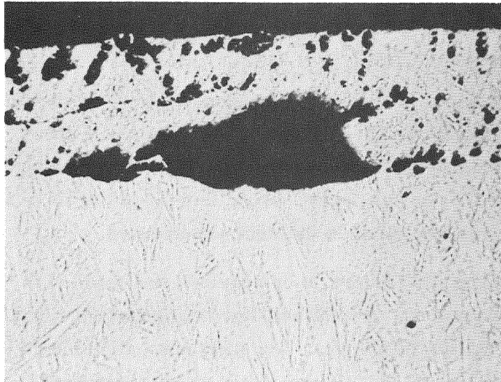
Figure 23a. Photomicrograph Shows Various Sized Voids at Surface of No. 4 Ball From L1 Bearing
