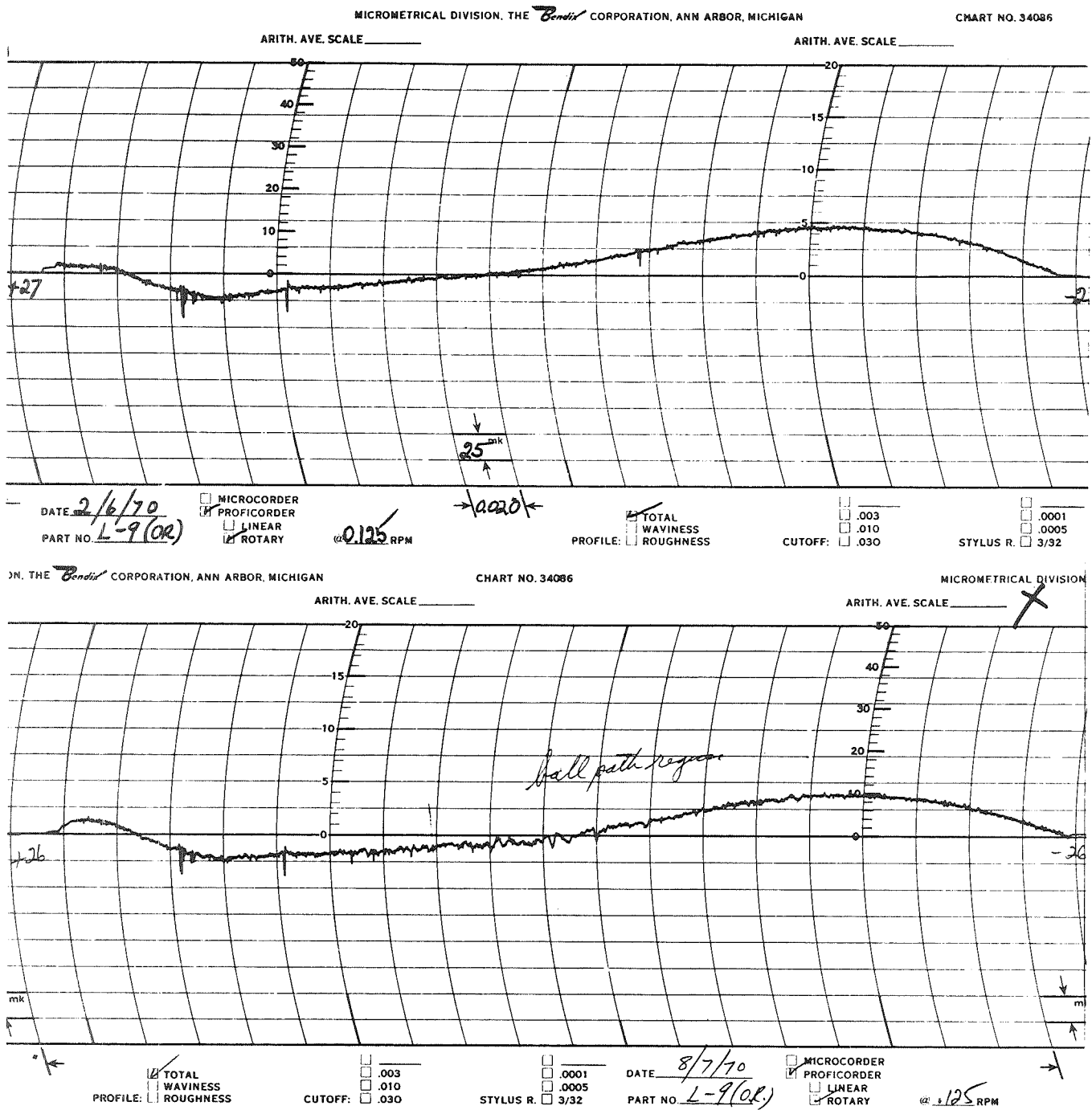
Figure 39. Comparative Profilometer Traces From AISI 440C Outer Race Run With Star J Balls and Salox-M Lubricant (L9)
