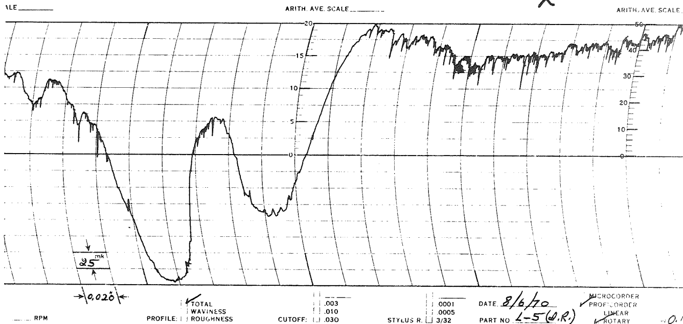
Figure 42. Comparative Profilometer Traces From AISI 440C Inner Race Run With AISI Balls and Chemloy 719 Lubricant (L5)
