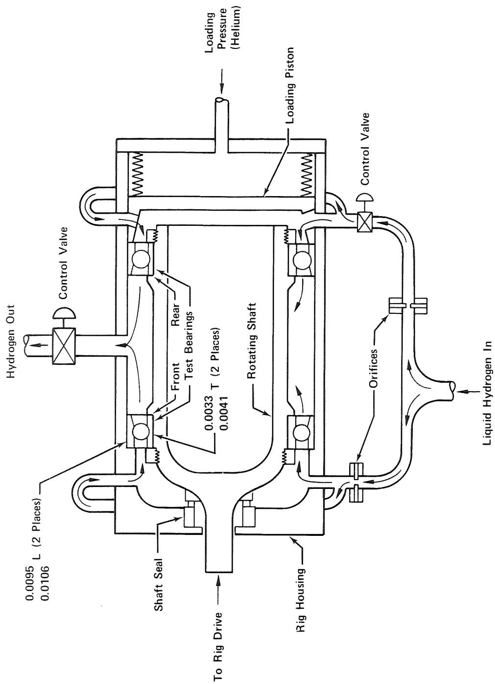
Figure 3. Bearing Test Rig Schematic Showing Coolant Flowpath
