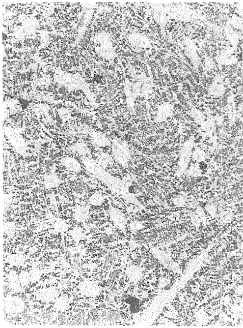
Microstructure of a Ball Adjacent to the Failed Ball Center
