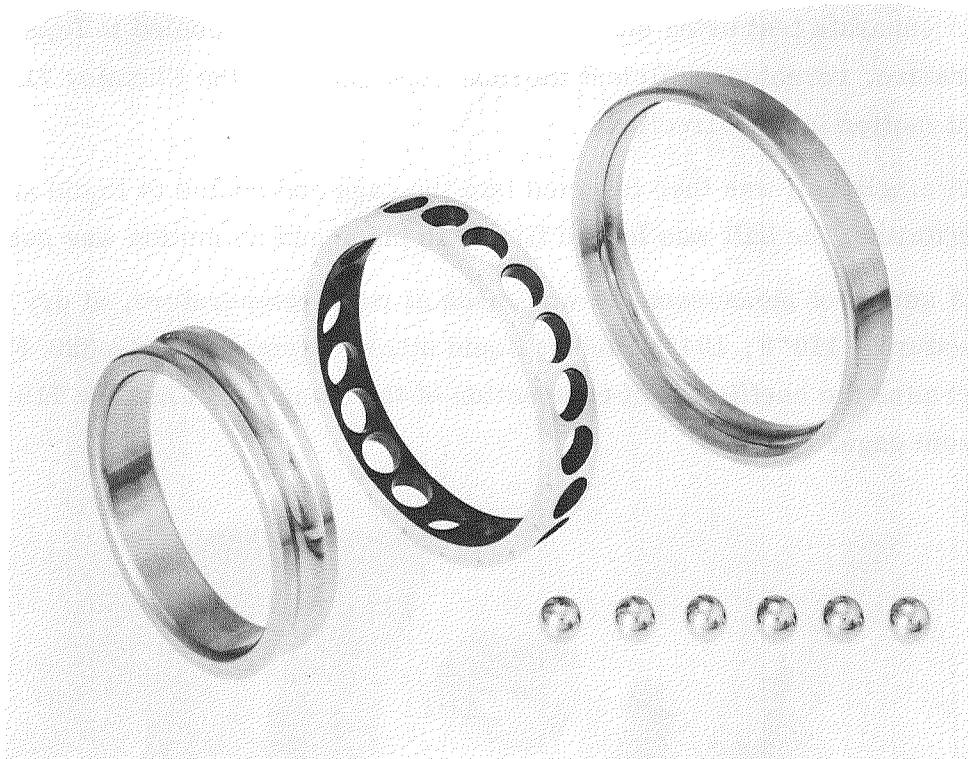
Figure 17. 110-mm Bearing, S/N 226 With AISI 440 Races and Balls; Chemloy 719 20-Pocket Cage
