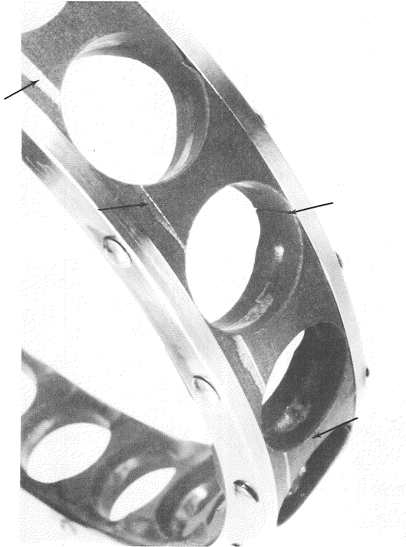
Figure 35. Cage L7, Fractures and Outer Race Rub, Test No. 15
