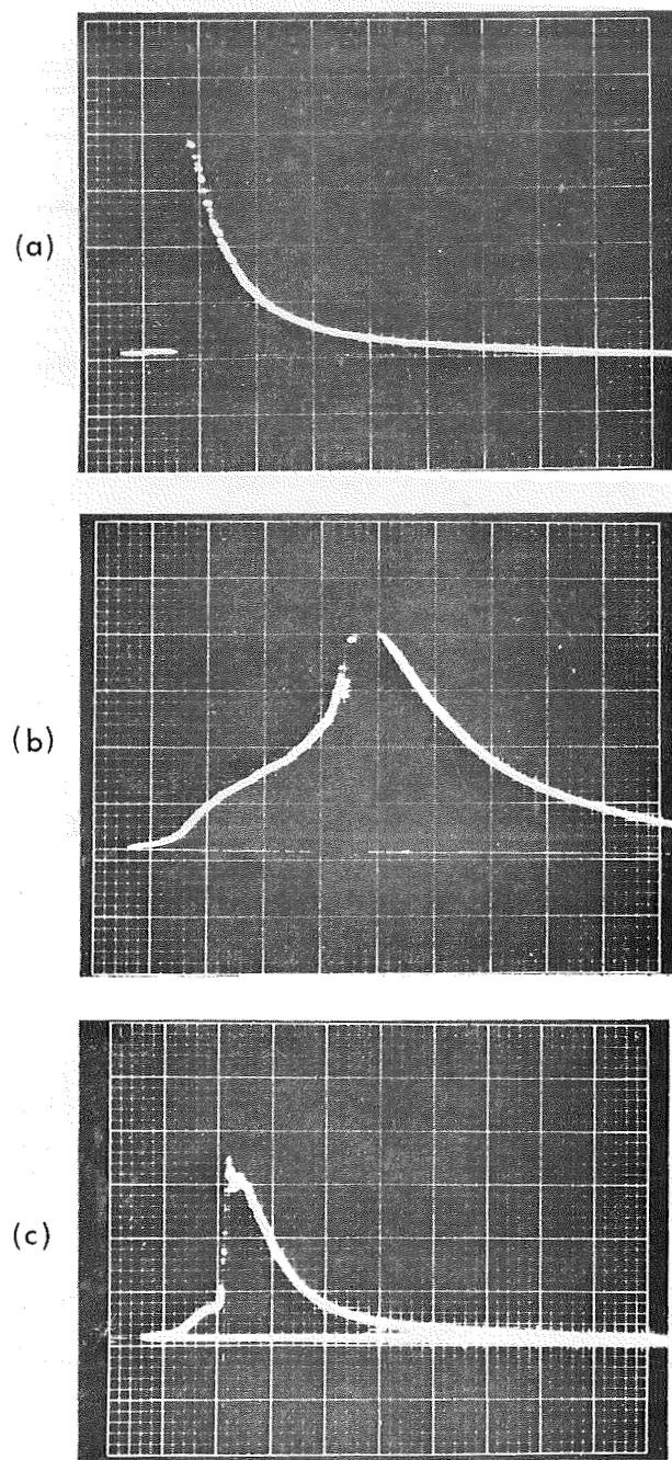
Fig. 3 - Oscilloscope traces for specimens fractured in 3.0 M HCl at -0.26 V ( A \approx 0.05 cm 2 ) horizontal - 2 ms/cm, vertical - 20 mA/cm Ti:14% Mo brittle Ti:14% Mo ductile Commercially pure Ti.
