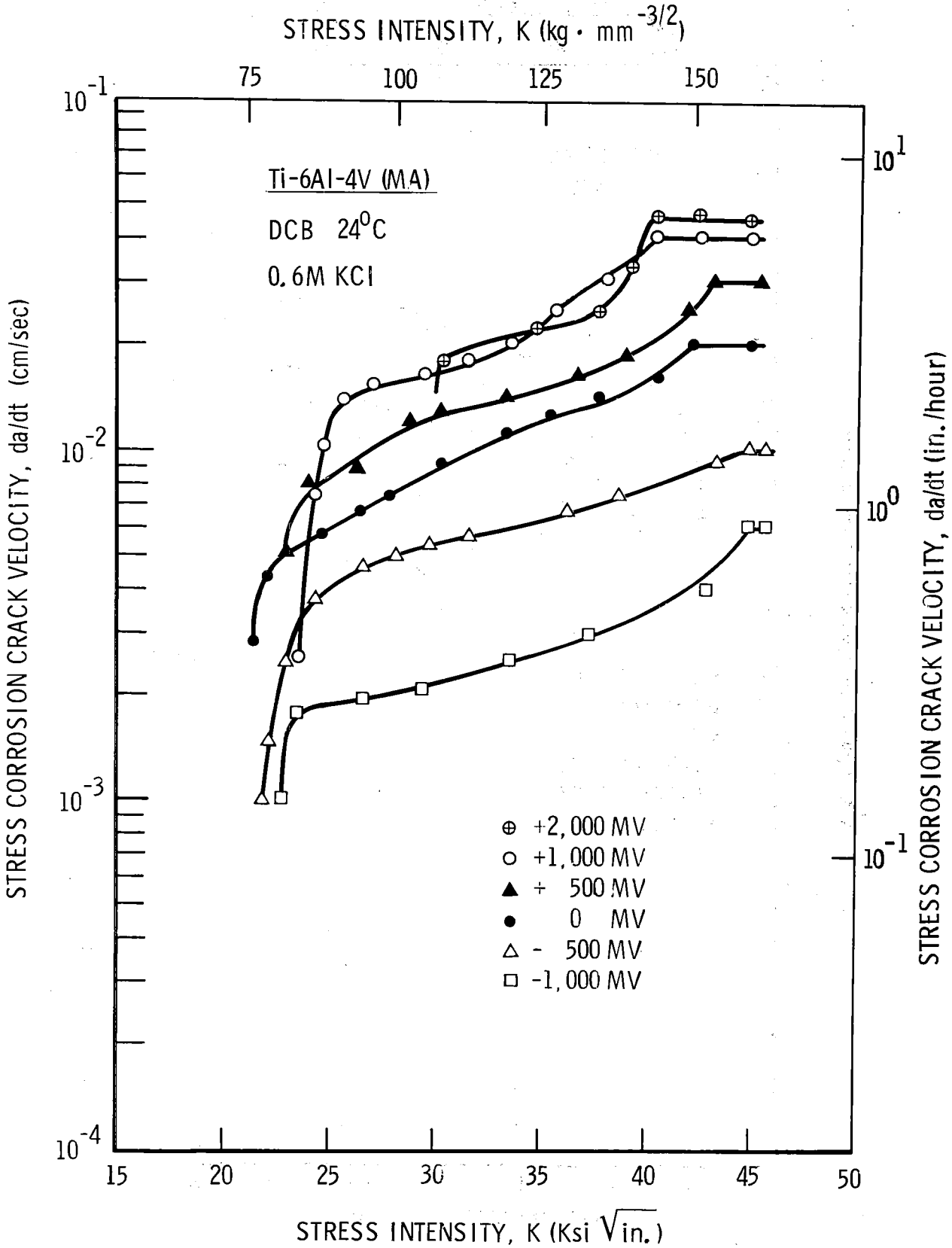
Figure 7 Velocity (V) vs stress intensity (K) relationships for Ti-6Al-4V tested in 0.6M KCL at room temperature and at several applied potentials
