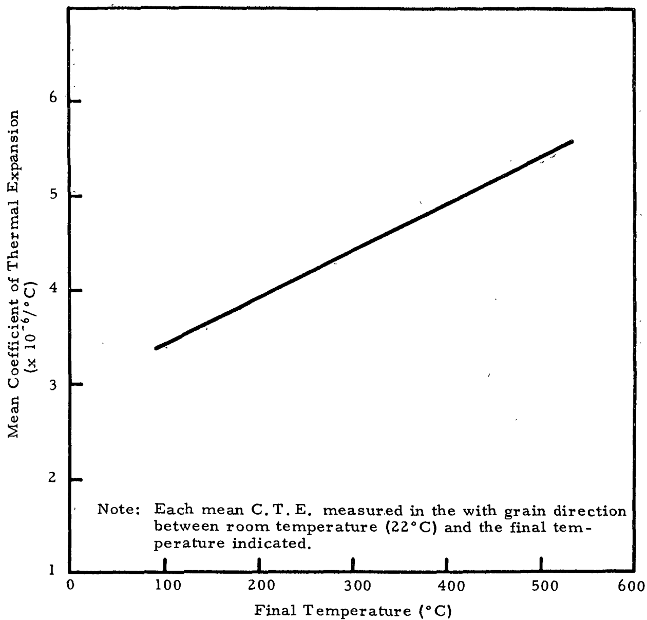
Figure 5. Mean Coefficient of Thermal Expansion - Grade CDJ-83.
