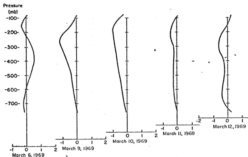
Figure 3.1. Vertical profiles of \frac{\delta \bar{\tau}_x}{\delta p} \Delta p in units of \text{kg m}^{-1} \text{sec}^{-2} per 100 mb, or \frac{\delta \bar{\tau}_x}{\delta p} in 10^{-4} , at 1800 GMT for days indicated. The pronounced reversal of profile occurred between March 8 and March 9, 1969.
