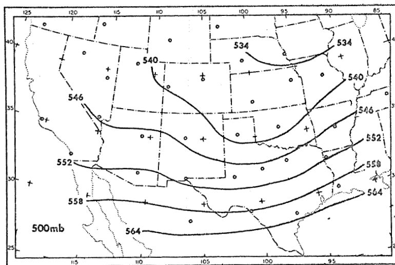
Figure 2.8. Height contours in tens of meters for 1800 GMT March 8, 1969 interpolated 300 mb (above) and 500 mb (below) maps.
