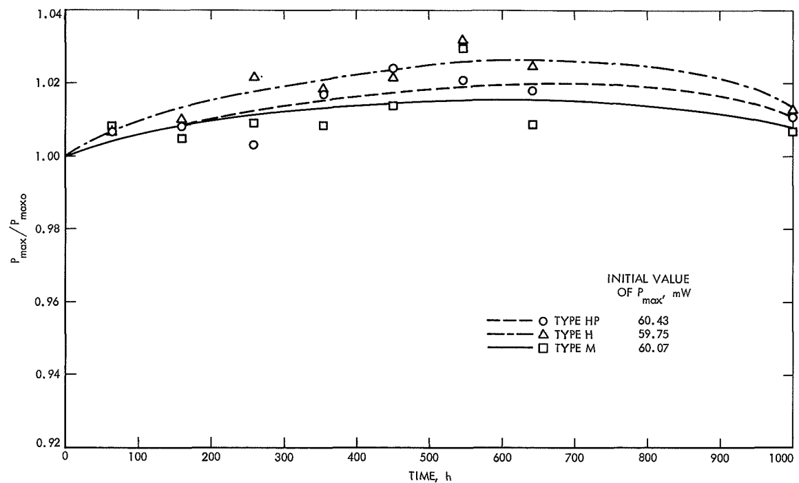
Fig. 32. Relative maximum power output of silicon solar cells as a function of time after exposure to LN_2 at -196^\circ C
