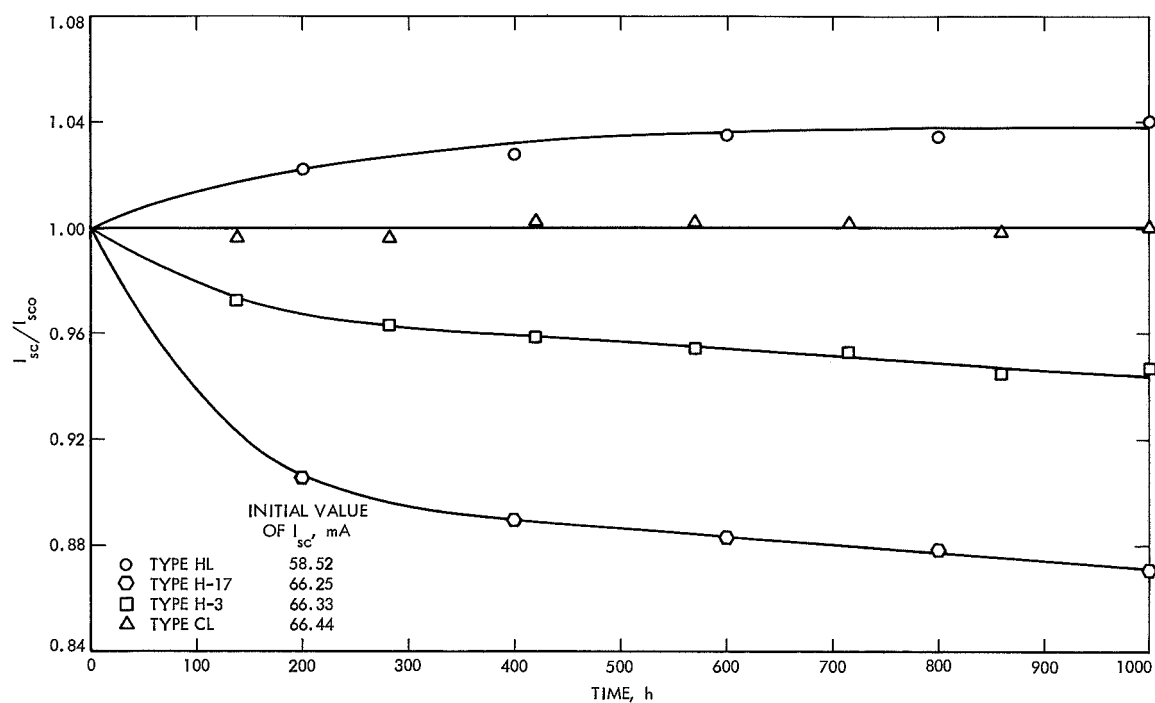
Fig. 8. Relative short-circuit current output of p-n silicon solar cells after long-term storage at 150°C
