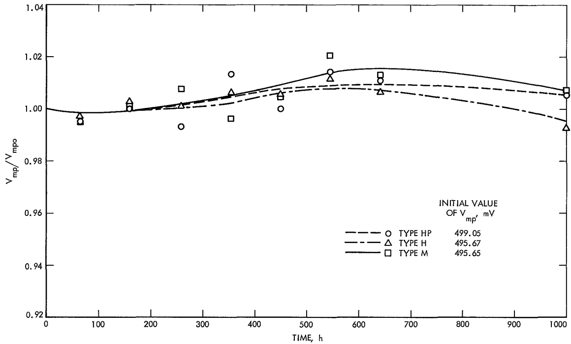
Fig. 31. Relative maximum power voltage output of silicon solar cells as a function of time after exposure to LN_2 at -196^\circ C
