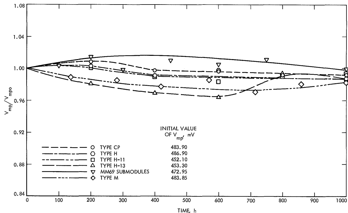
Fig. 6. Relative maximum power voltage output of n-p silicon solar cells after long-term storage at 150°C
