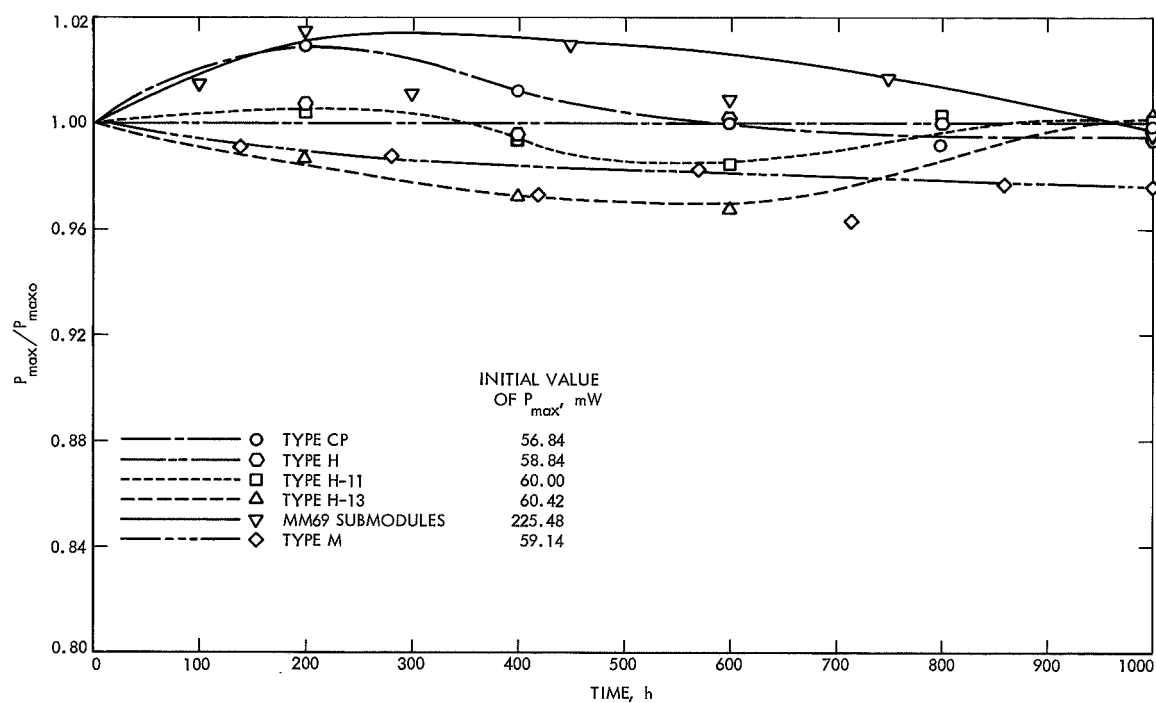
Fig. 7. Relative maximum power output of n-p silicon solar cells after long-term storage at 150°C
