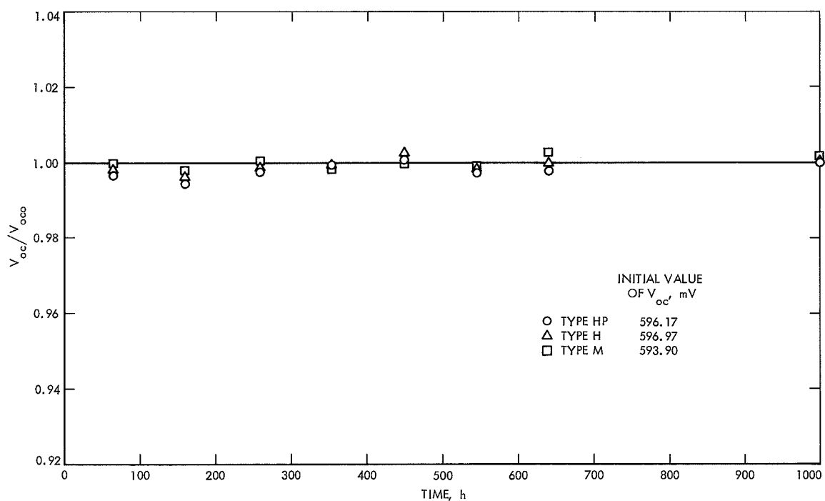
Fig. 30. Relative open-circuit voltage output of silicon solar cells as a function of time after exposure to LN_2 at -196^\circ C
