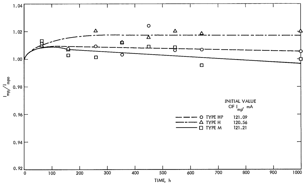
Fig. 29. Relative maximum power current output of silicon solar cells as a function of time after exposure to LN_2 at -196^\circ C
