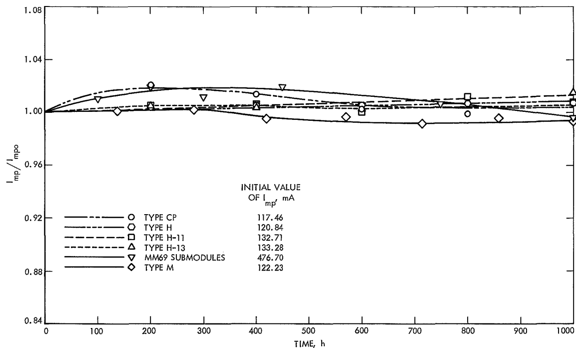
Fig. 5. Relative maximum power current output of n-p silicon solar cells after long-term storage at 150°C
