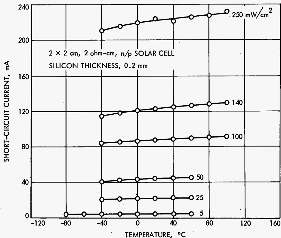
Figure 9.—Measured variation of short-circuit current with temperature (ref. 17).
