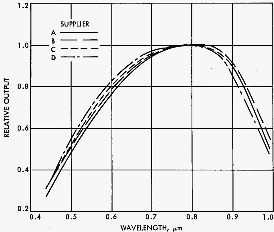
Figure 3.—Measured relative energy conversion of typical cells versus the wavelength of light (ref. 9).
