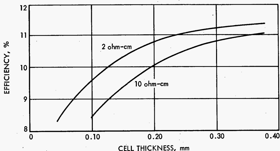
Figure 5.—Typical n/p solar cell efficiency vs silicon thickness for nominal 2 and 10 ohm-cm base resistivities. Sunlight simulator (X-25 L spectroSun) 140-mW/cm 2 balloon calibration; active area 3.9 cm 2 ; cell temperature 28°C (ref. 11).
