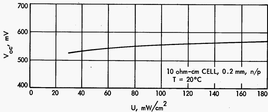
Figure 7.—Variation of open-circuit voltage V_{oc} with illumination intensity U .
