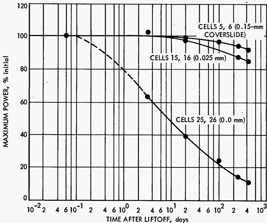
Figure 12.—Maximum power vs time for 0.30-mm-thick solar cells with various coverslide thicknesses (ATS-1, ref. 19).
