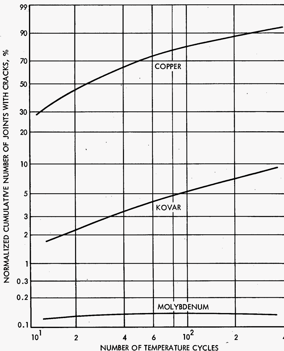
Figure 17.—Cumulative number of joints with cracks (Weibull Probability Scale) vs number of temperature cycles (+75°C to -175°C) for three interconnector materials (ref. 83).
