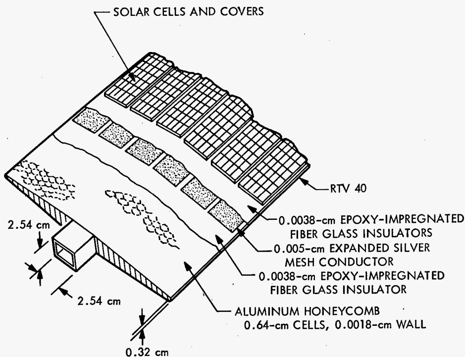
Figure 15.—Construction of the IMP-D solar paddles (ref. 29).
