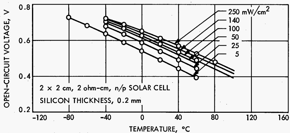
Figure 10.—Measured variation of open-circuit voltage with temperature (ref. 17).
