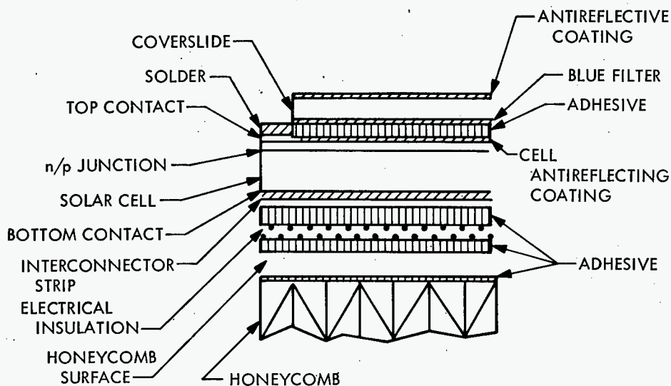
Figure 13.—Schematic of a conventional n/p solar cell element (ref. 25).
