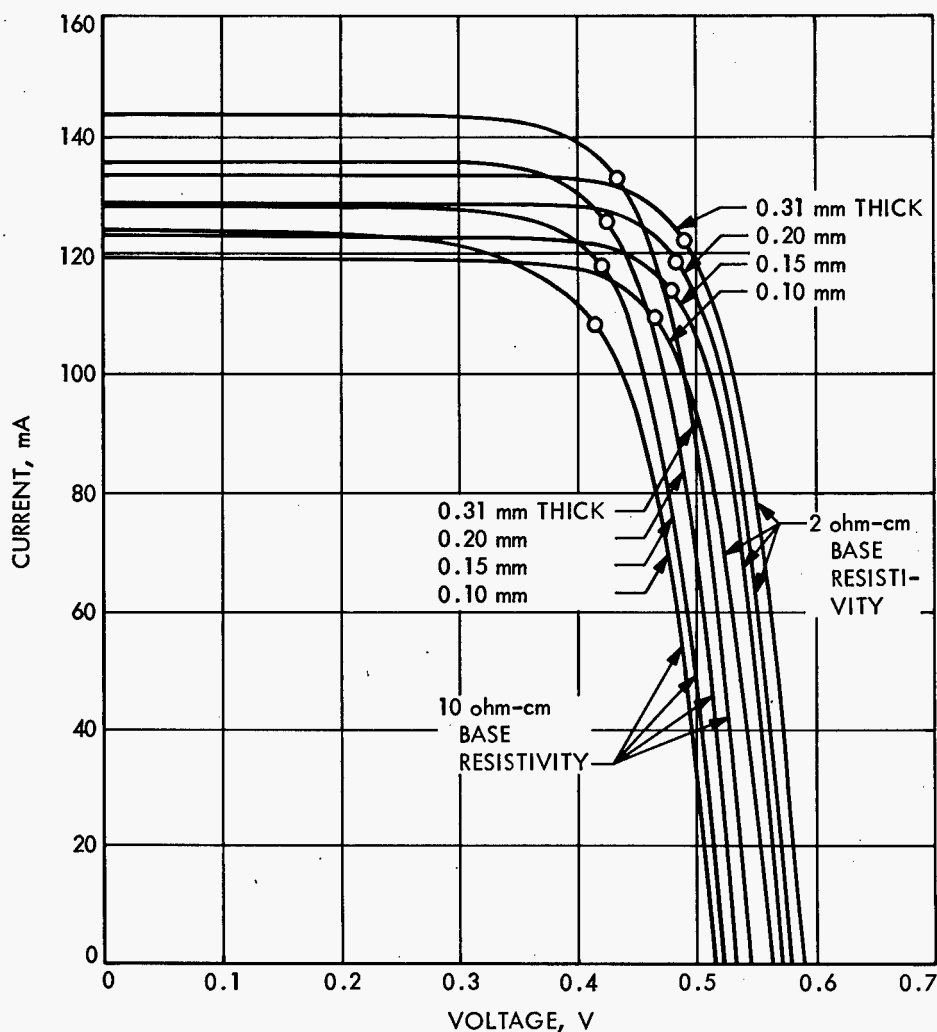
Figure 4.—Typical current output versus voltage across silicon solar cells, for several cell thicknesses and base region resistivities. Measured in 140 \text{ mW/cm}^2 simulated sunlight, for 2 \times 2 \text{ cm} n/p cells at 28^\circ\text{C} (ref. 11).
