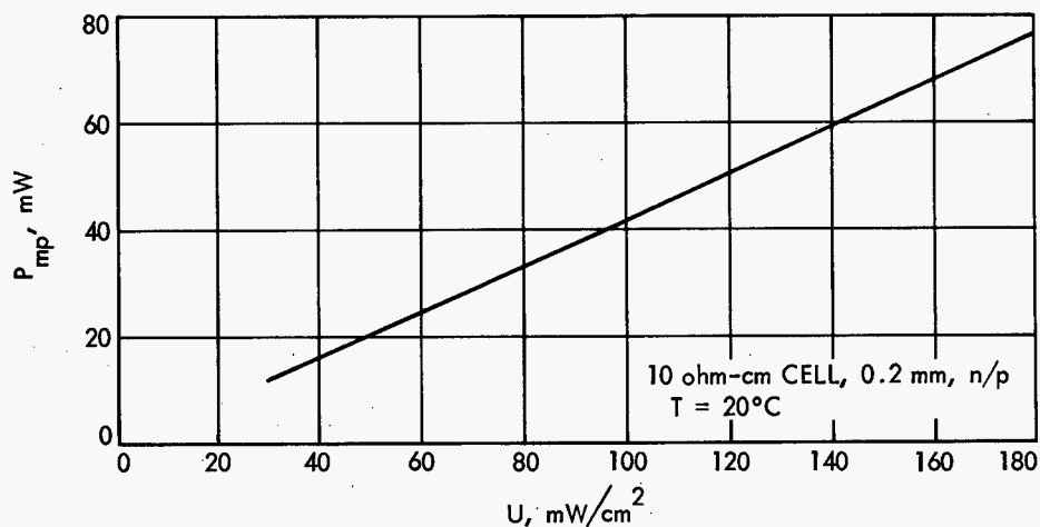
Figure 8.—Variation of maximum power P_{mp} with illumination intensity U .
