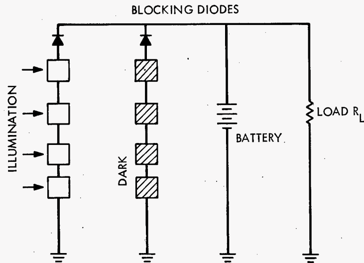
Figure 22.—Two parallel strings of solar cells, with one dark and producing no current. The isolation diodes prevent it from shunting current from the load R_L .
