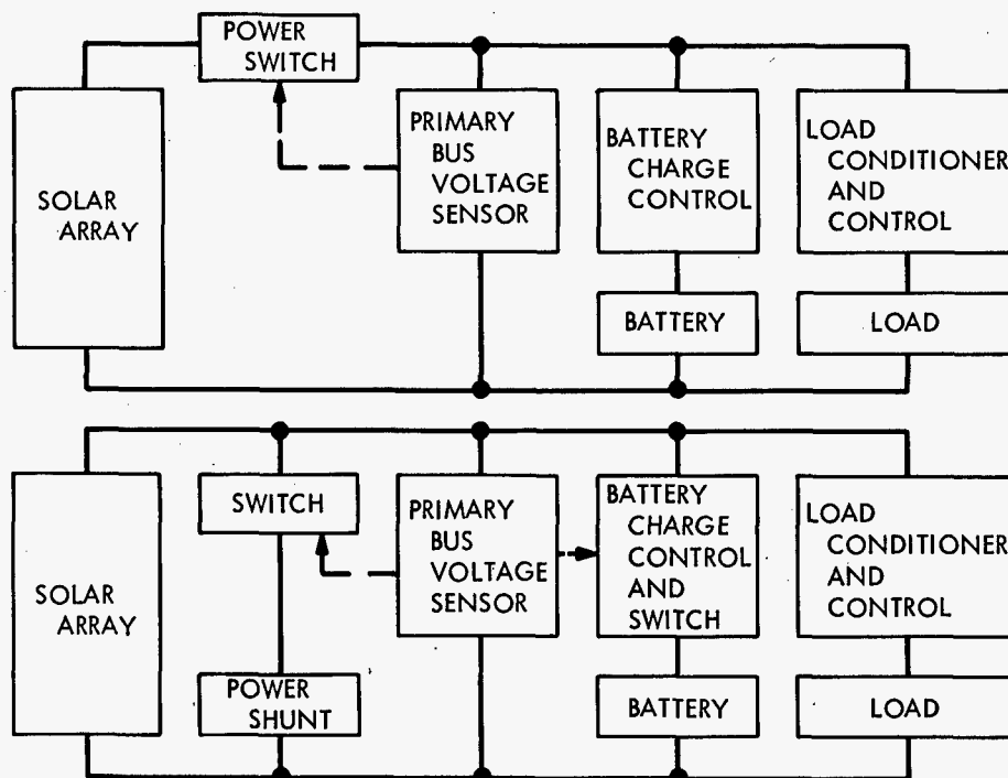
Figure 20.—Schematic diagrams of two typical power supply circuits for satellites (ref. 26).
