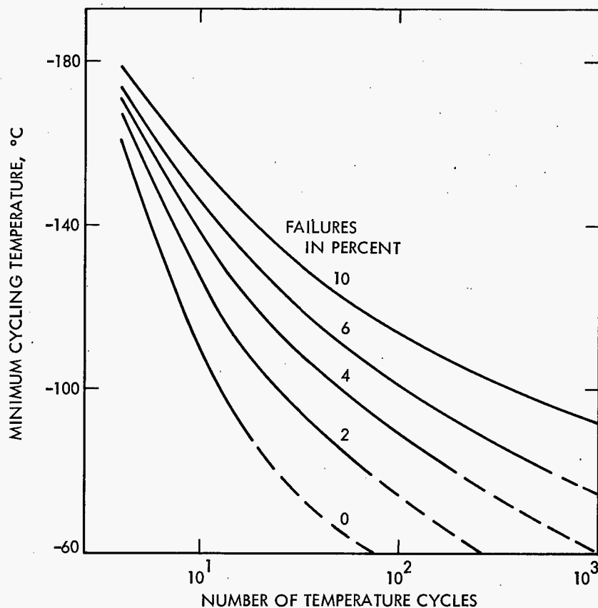
Figure 18.—Minimum permissible cycling temperature vs required number of thermal cycles for constant joint failure levels (for joints with 0.07-mm-thick copper interconnectors) (ref. 33).
