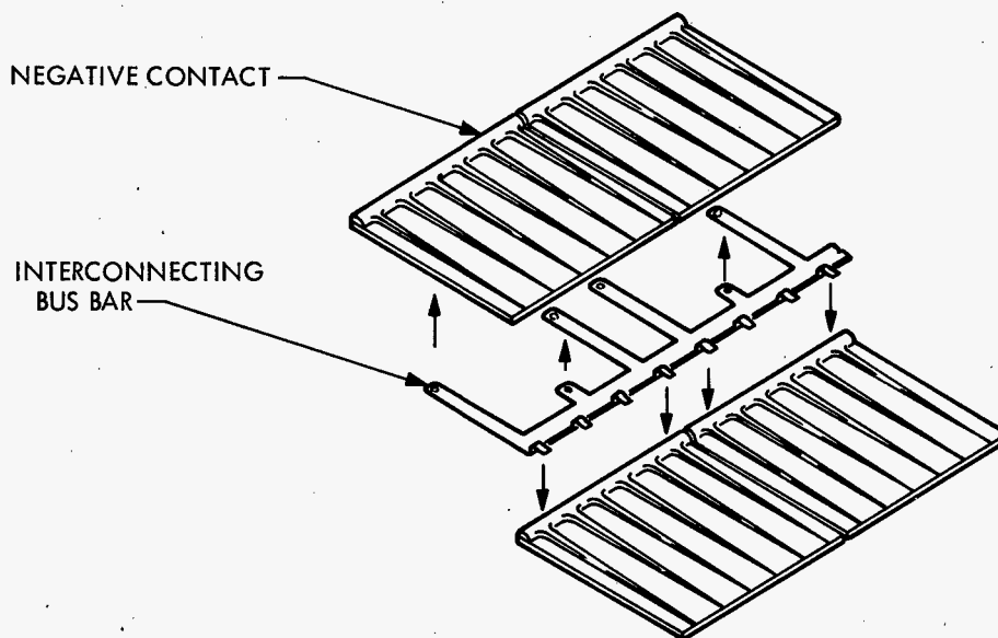
Figure 2.—Four typical solar cells ( 2 \times 2 cm) and interconnector. The thickness of the front (negative) contact is exaggerated.
