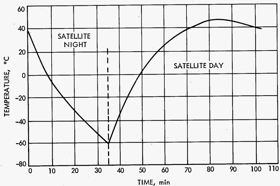
Figure 16.—The Nimbus 2, with solar cell array on two oriented panels, initially provided 450 watts at 40°C. The panel temperature, measured through one orbit, is shown above.
