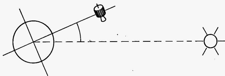
Figure 21.—Spin-stabilized synchronous satellites may have their lateral surfaces at an angle of 23 deg with respect to the earth–Sun line near the times of winter (and summer) solstice. (Cosine of 23 deg is 0.92.)
