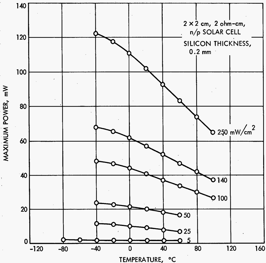
Figure 11.—Measured variation of maximum power with temperature (ref. 17).
