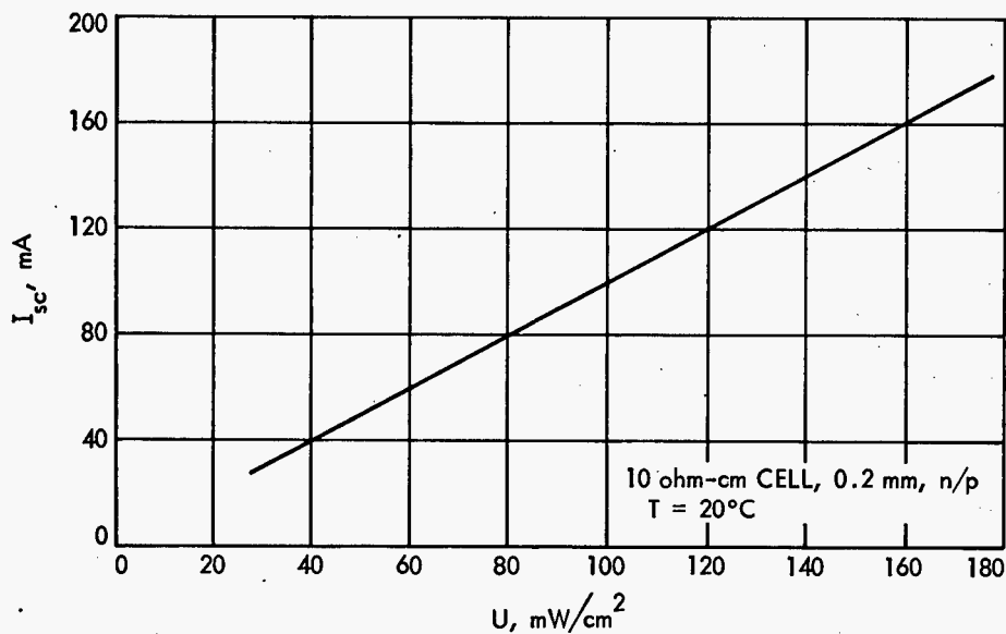
Figure 6.—Variation of short-circuit current I_{sc} with illumination intensity U (ref. 13).
