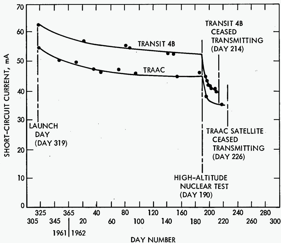
Figure 1.—Solar cell output as a function of time for Transit 4B and TRAAC (ref. 5).
