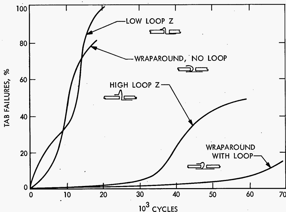
Figure 19.—Stress relief loops, interconnector flexure test results (ref. 34). The high loop is 1.3 mm high and the low loop is 0.4 mm high.
