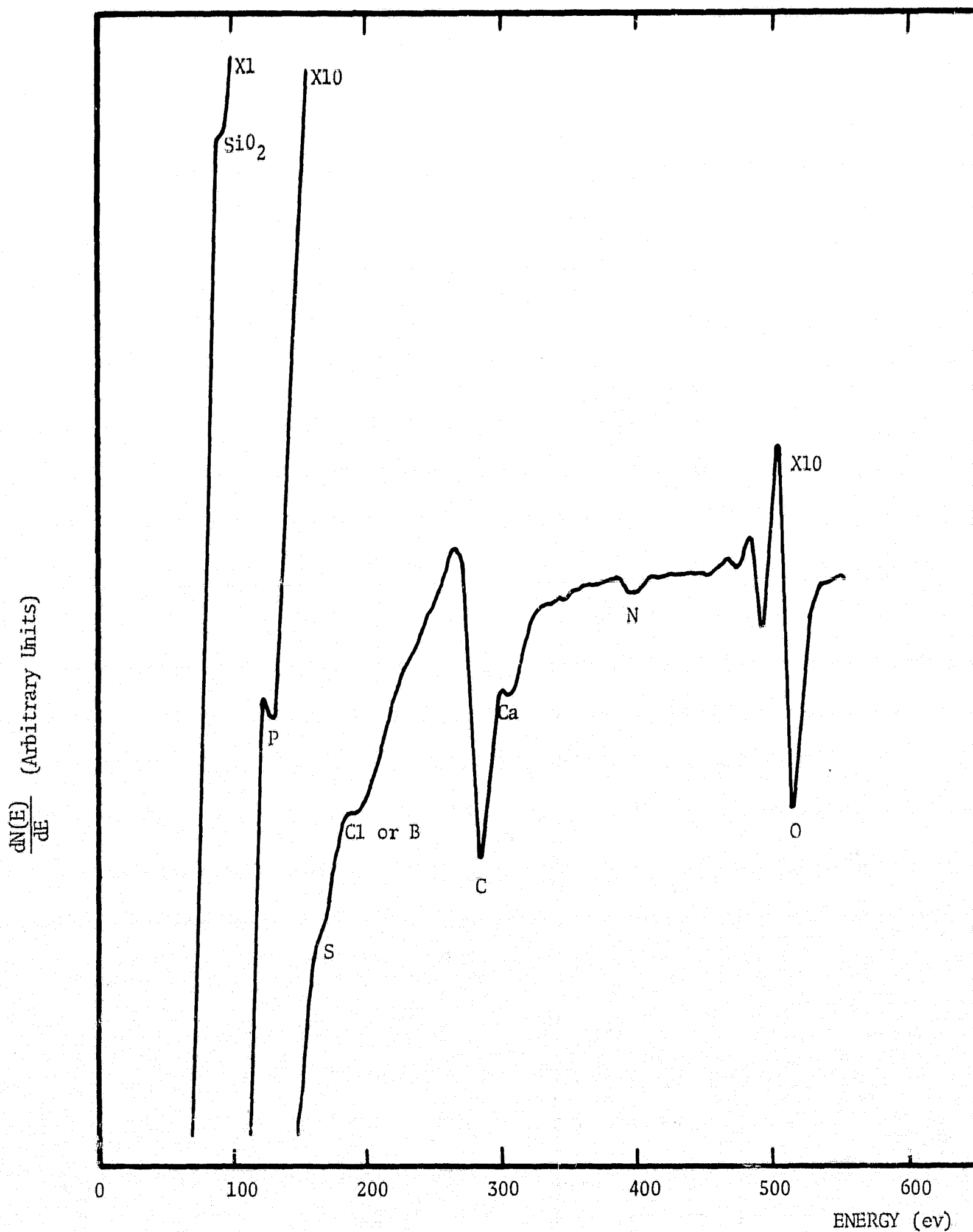
FIGURE 29. TAKEN FROM COMPLETED DEVICE
