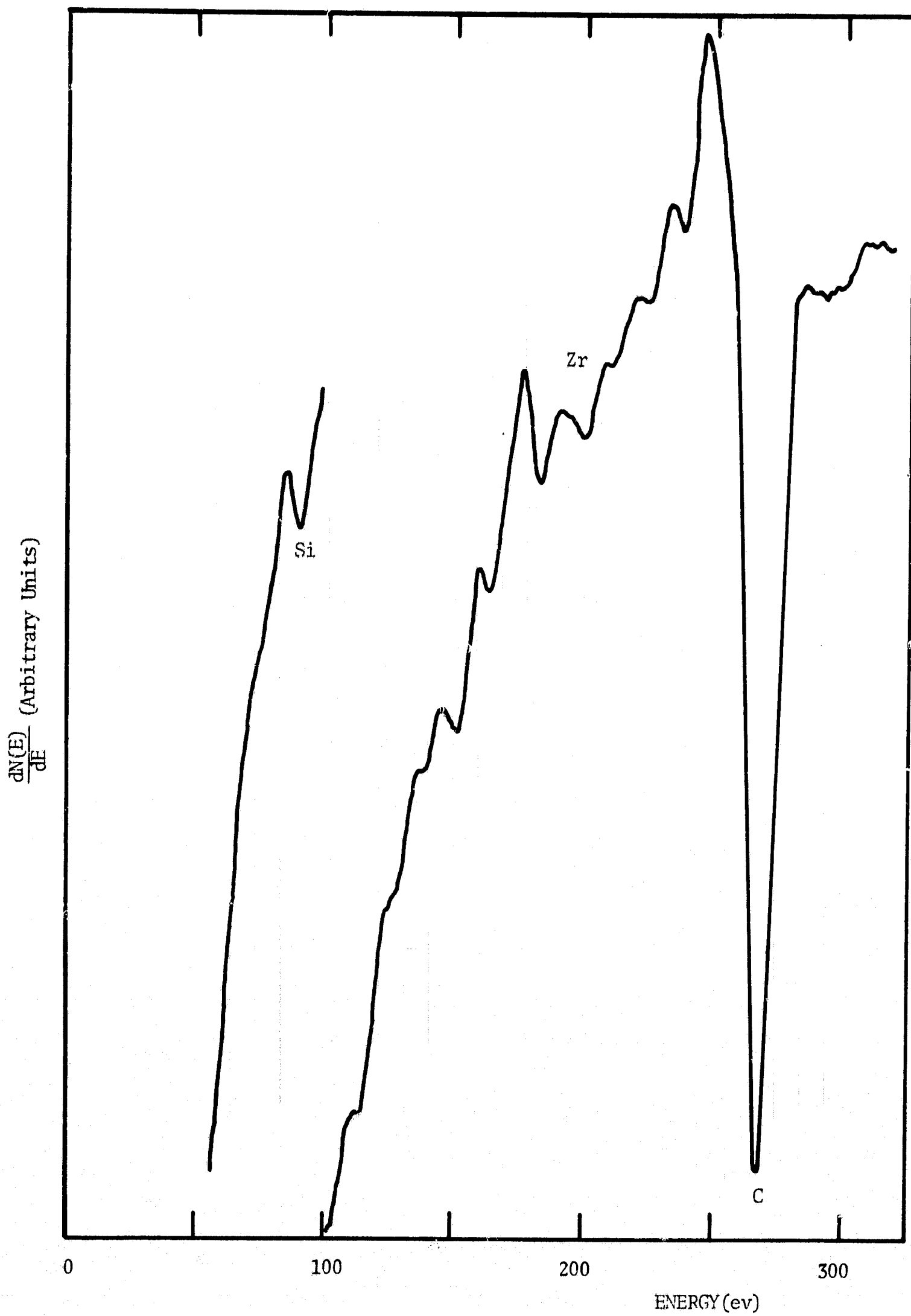
FIGURE 4. WAFER INTENTIONALLY CONTAMINATED WITH Zr
