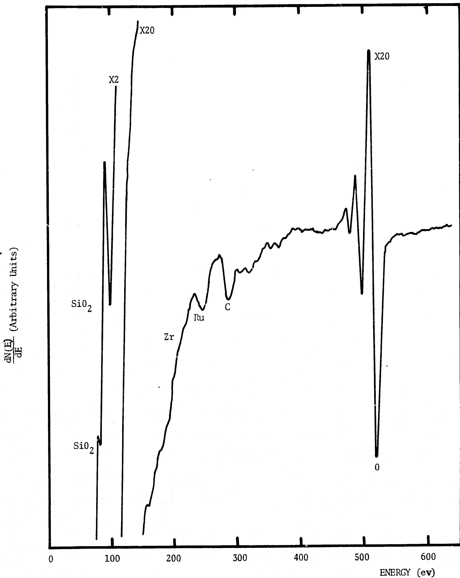
FIGURE 14. TYPICAL SPECTRUM OF WAFER AFTER FIRST OXIDATION
