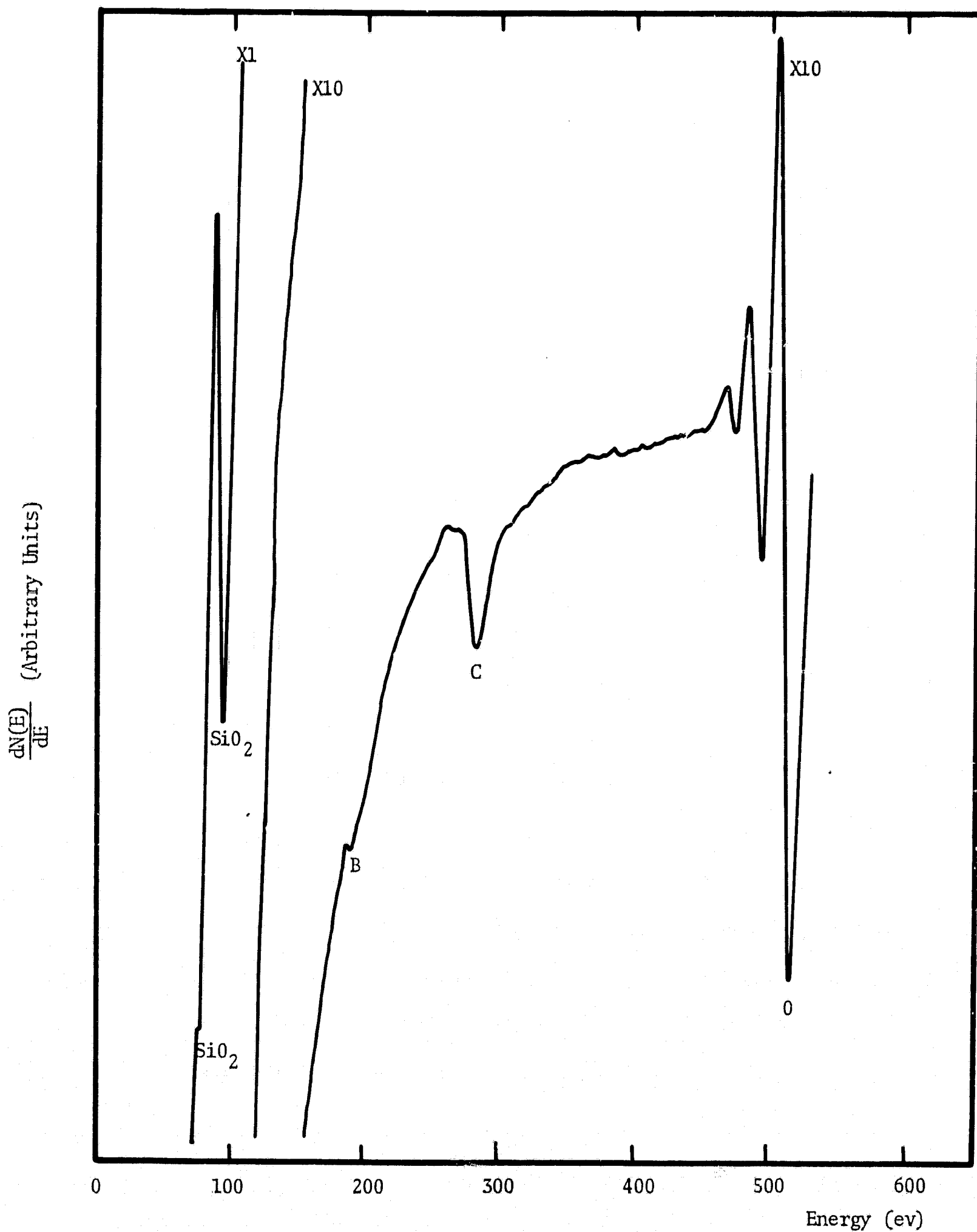
FIGURE 19. WAFER AFTER BASE DIFFUSION SHOWING SURFACE BORON 30
