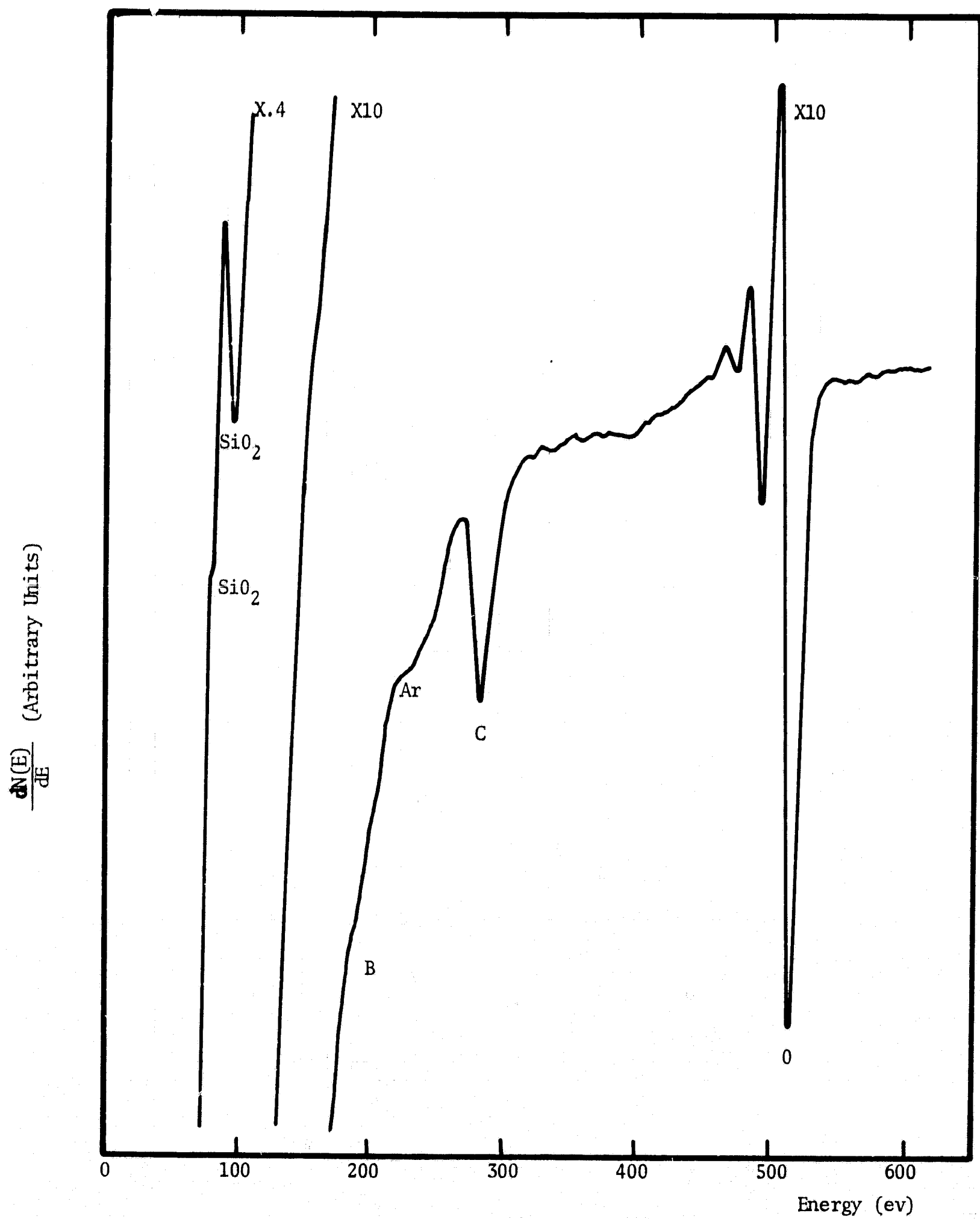
FIGURE 18. TYPICAL WAFER AFTER BASE DIFFUSION
