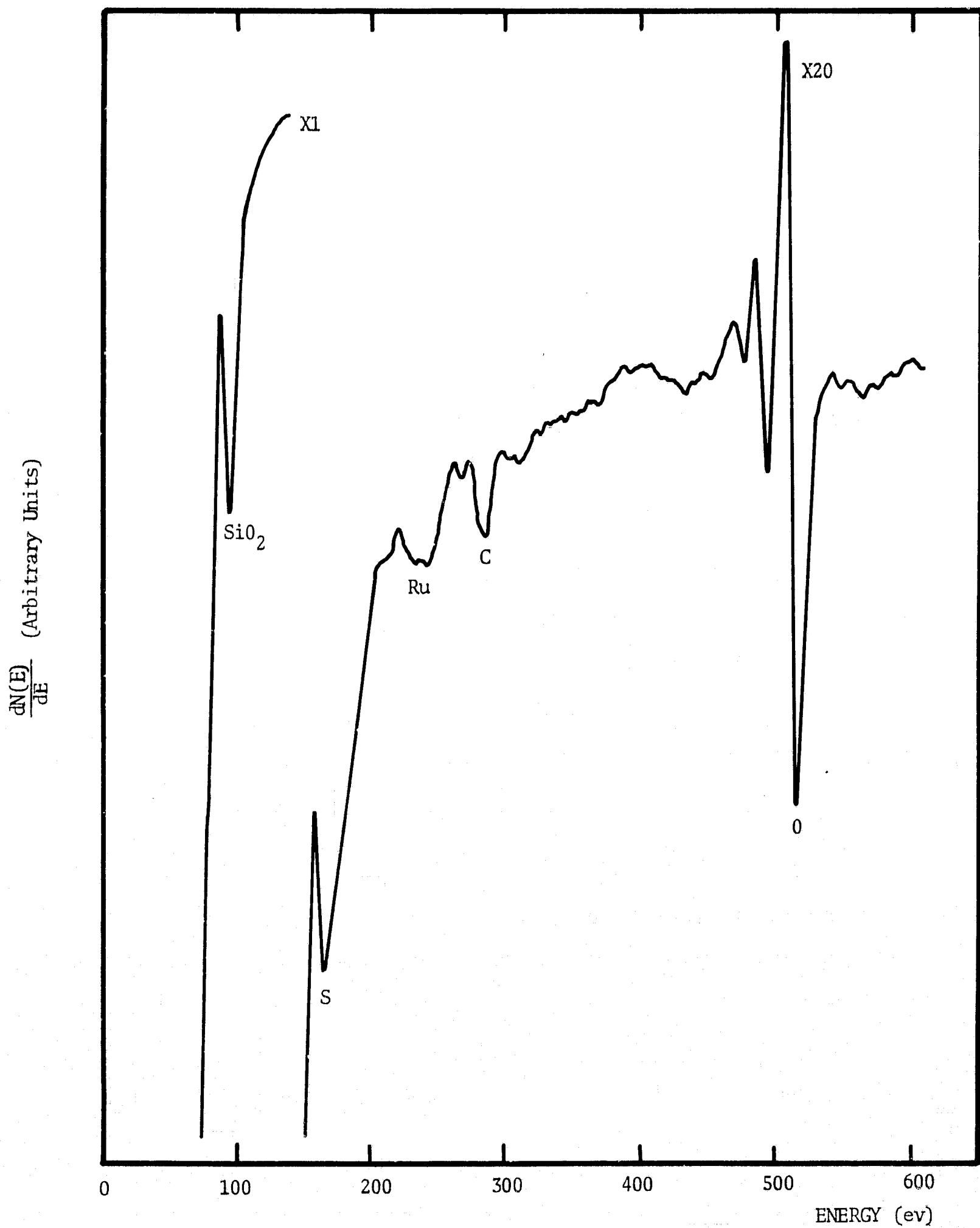
FIGURE 15. WAFER AFTER FIRST OXIDATION SHOWING S CONTAMINATION
