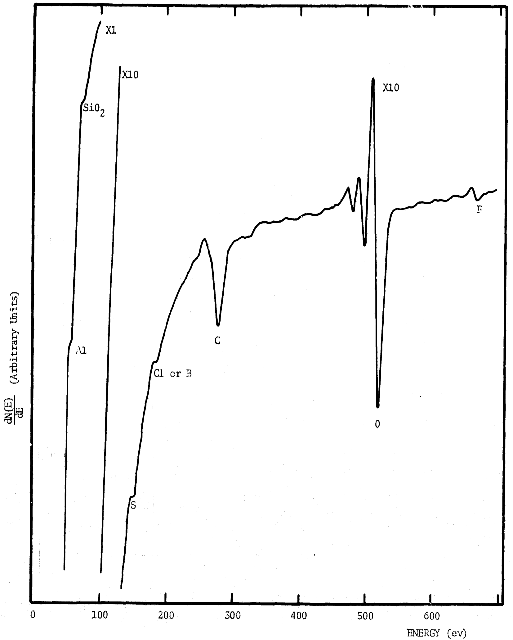
FIGURE 26. WAFER AFTER AL MASK, PHOTORESIST REMOVED SHOWING F CONTAMINATION 40
