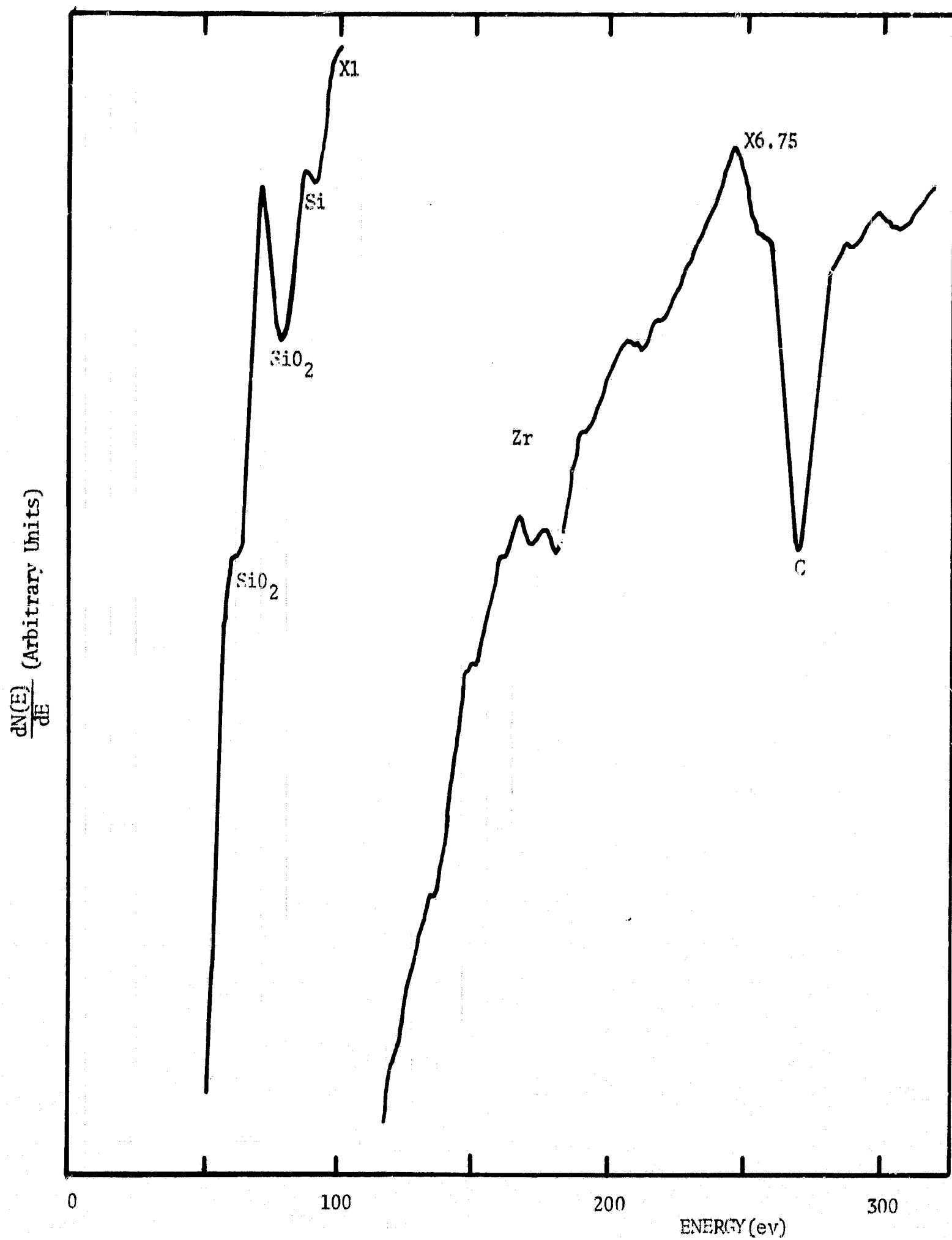
FIGURE 3. WAFER AFTER POLISHING (mild cleaning)
