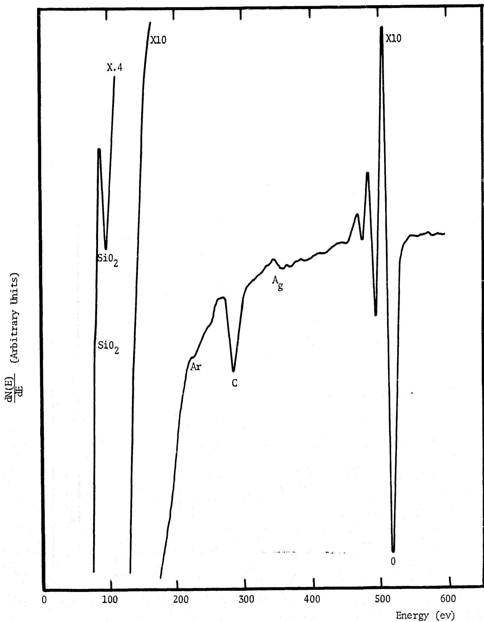
FIGURE 21. WAFER AFTER BASE DIFFUSION SHOWING \text{Ag} CONTAMINATION 32
