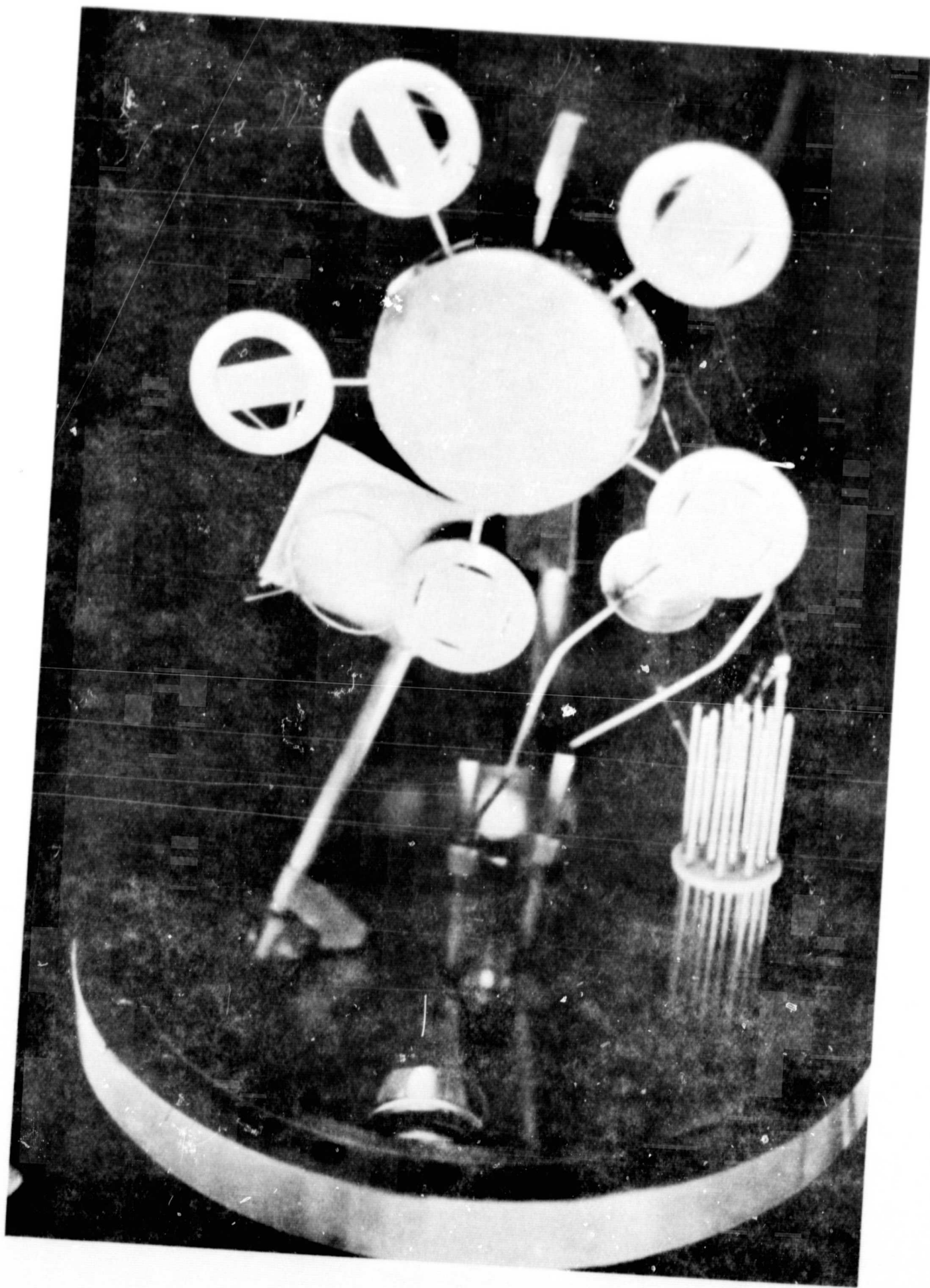
Figure 2. Sample Turret for Five Samples.
