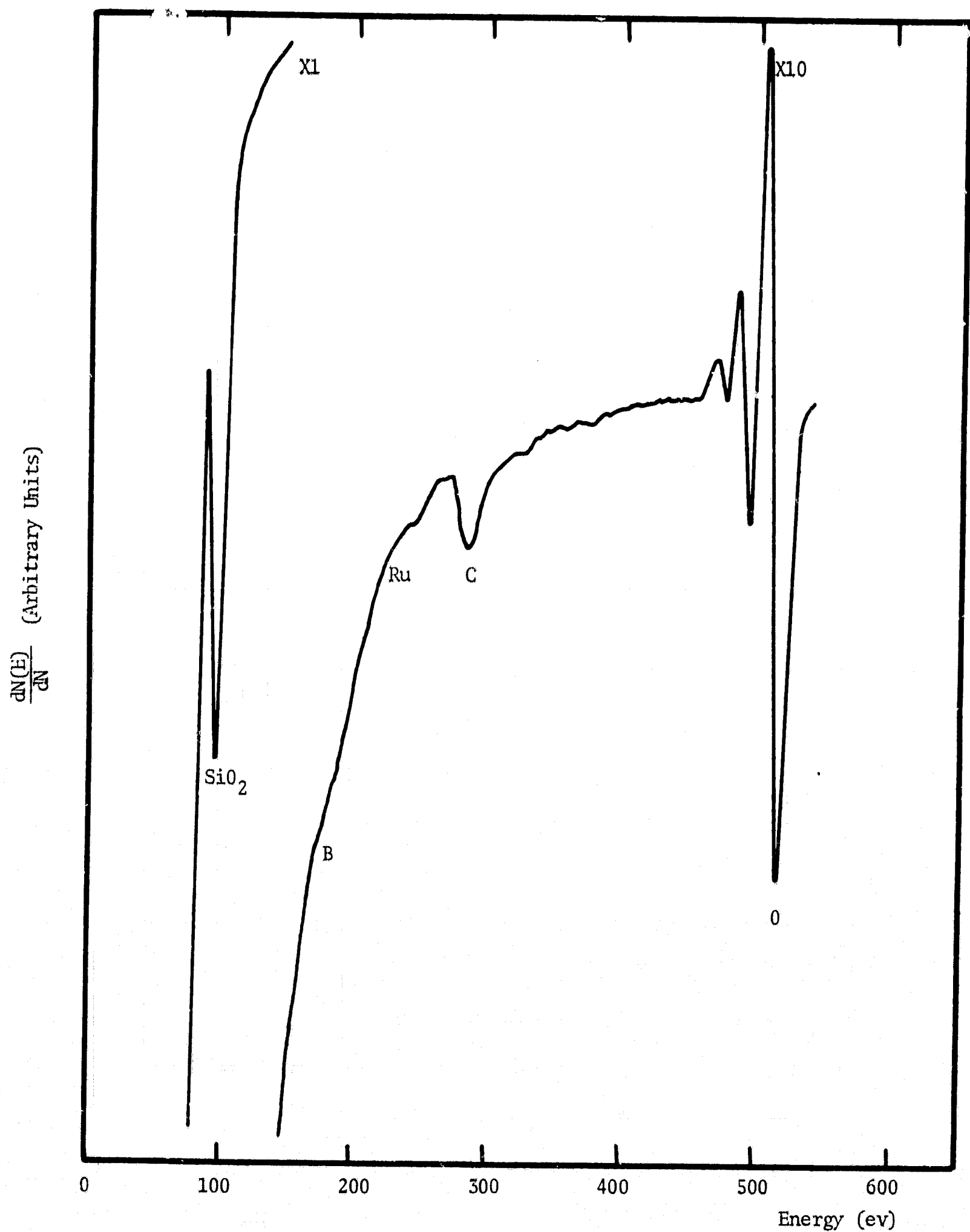
FIGURE 20. WAFER AFTER BASE DIFFUSION SHOWING Ru
