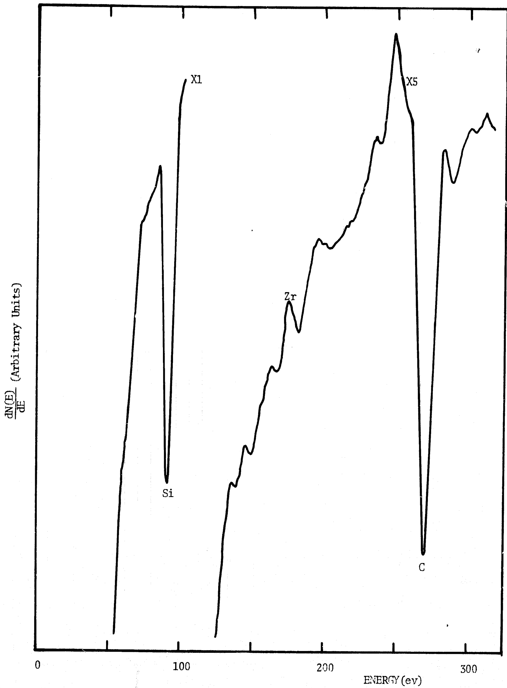
FIGURE 5. WAFER AFTER HF DIP AND HEATING
