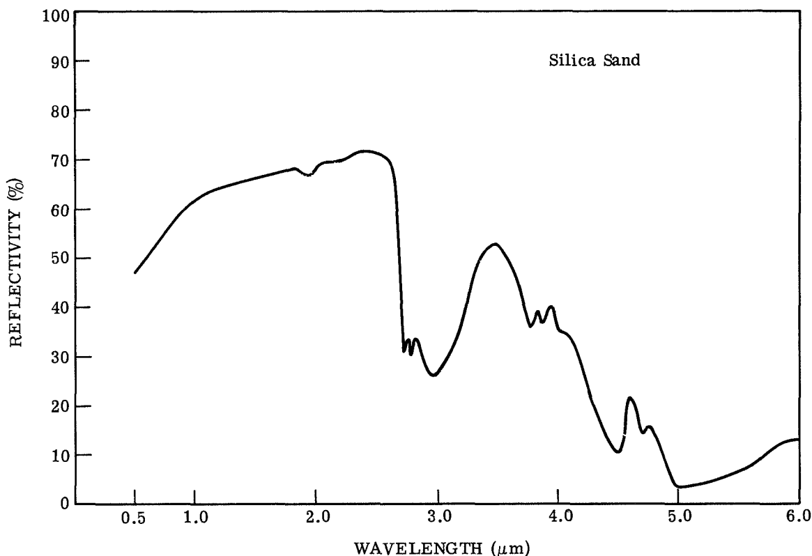
FIGURE 17. REFLECTANCE OF SILICA SAND
