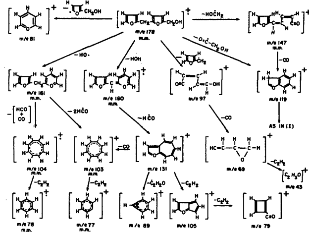
Fig. 5. Proposed fragmentation route for 5-furfuryl-furfuryl alcohol.
