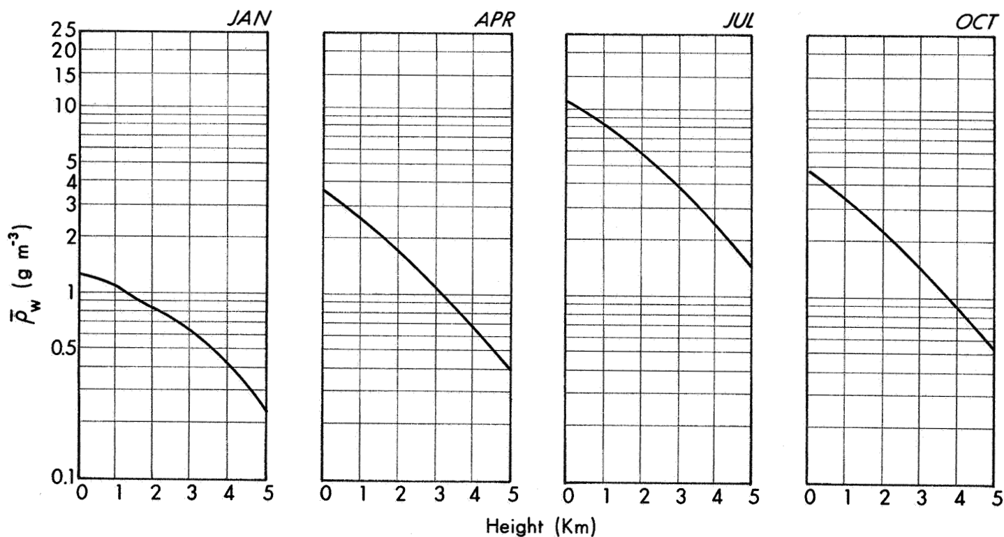
Figure A-4 Mean Absolute Humidity vs Height for Midseason Months - Region 4
