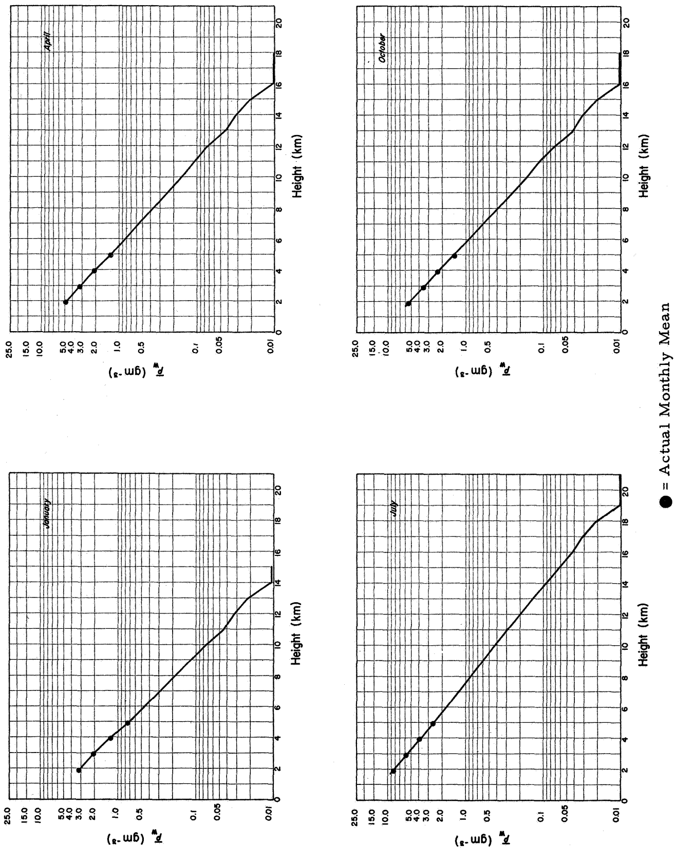
Figure 11 Comparison between Actual and Derived Mean Absolute Humidity vs Height for Midseason Months - Region 26
