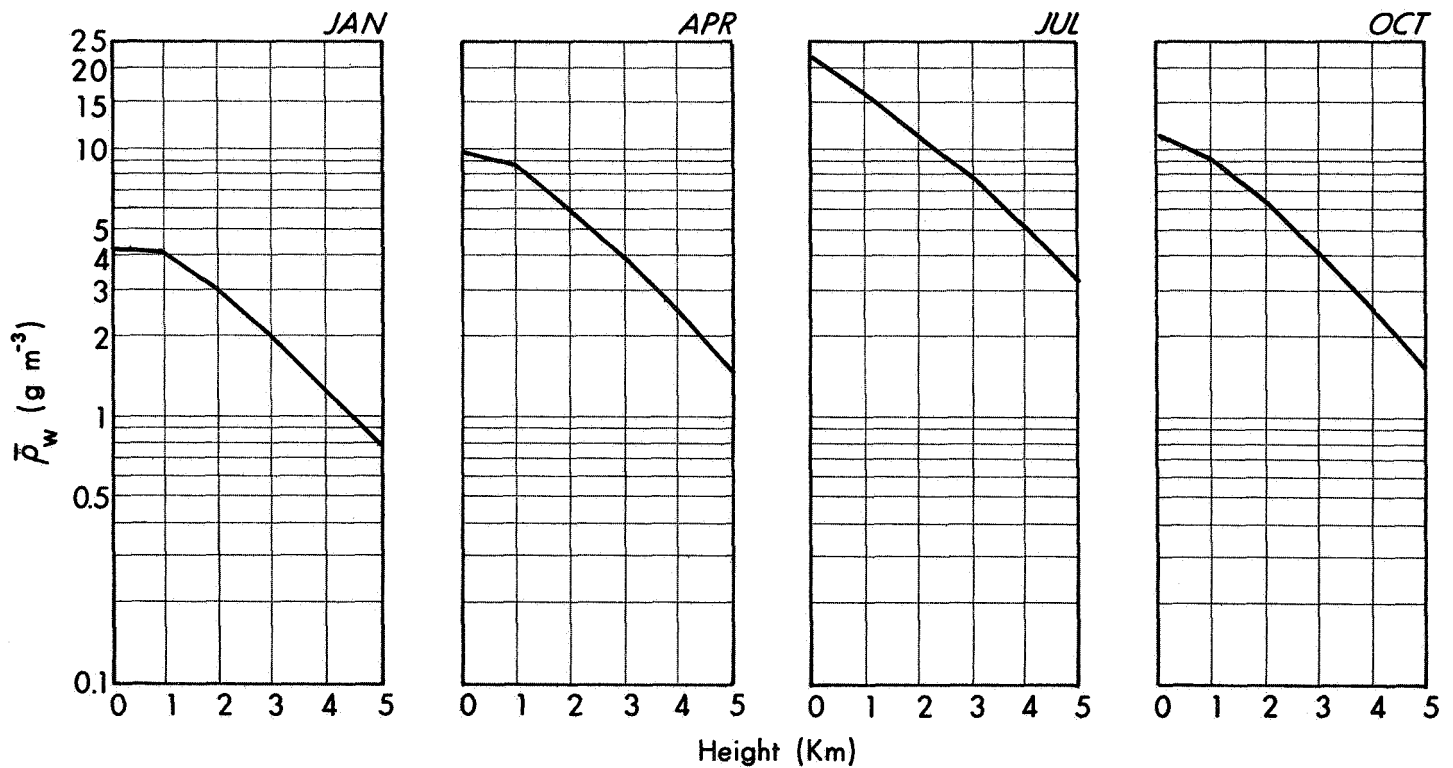
Figure A-34 Mean Absolute Humidity vs Height for Midseason Months - Region 34
